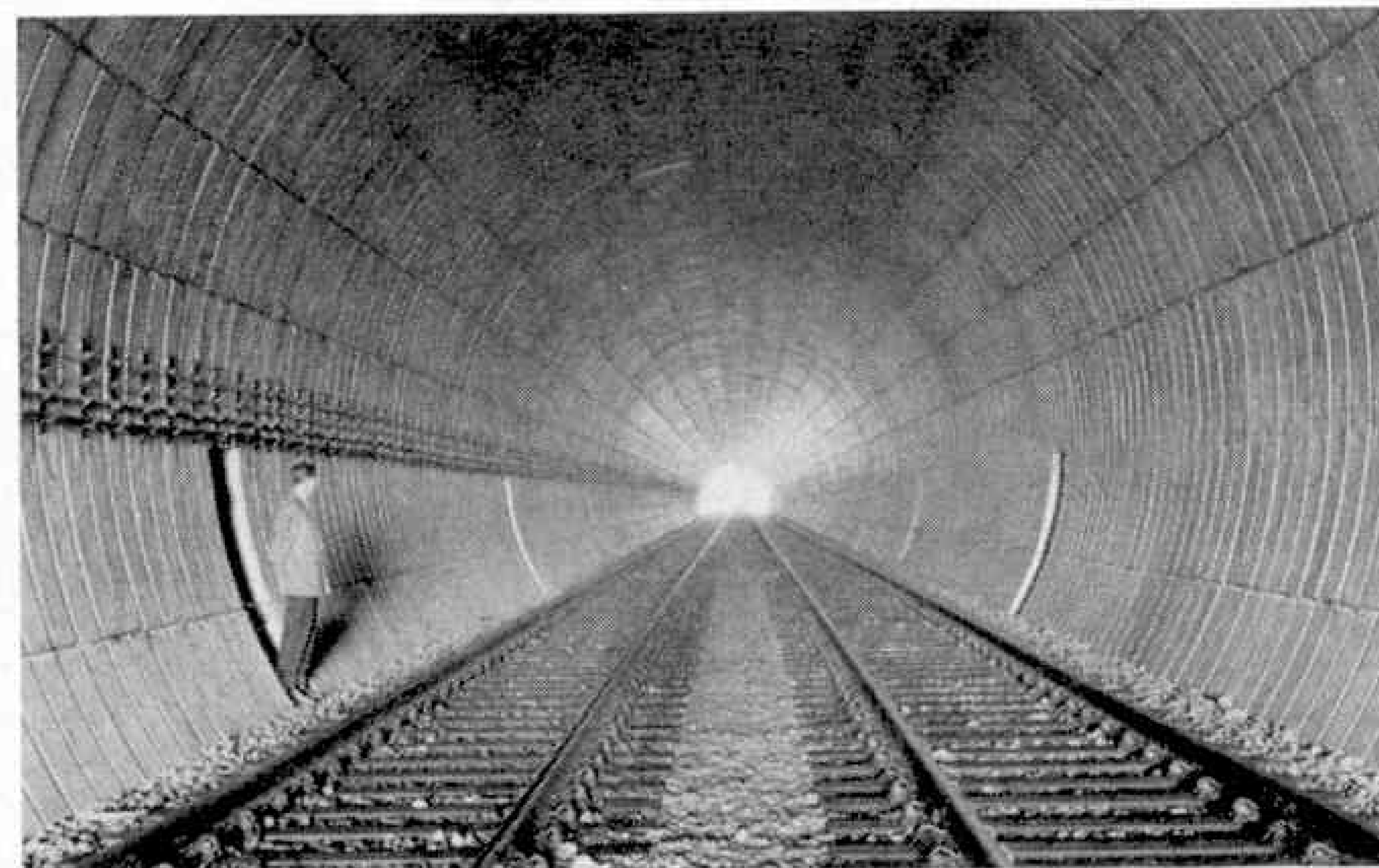
Inside one of the new tunnels, with the track completed. The tunnel lining, built of pre-cast concrete segments, is clearly shown, as also are the refuges for surfacemen and the hooks for supporting the signalling cables.
