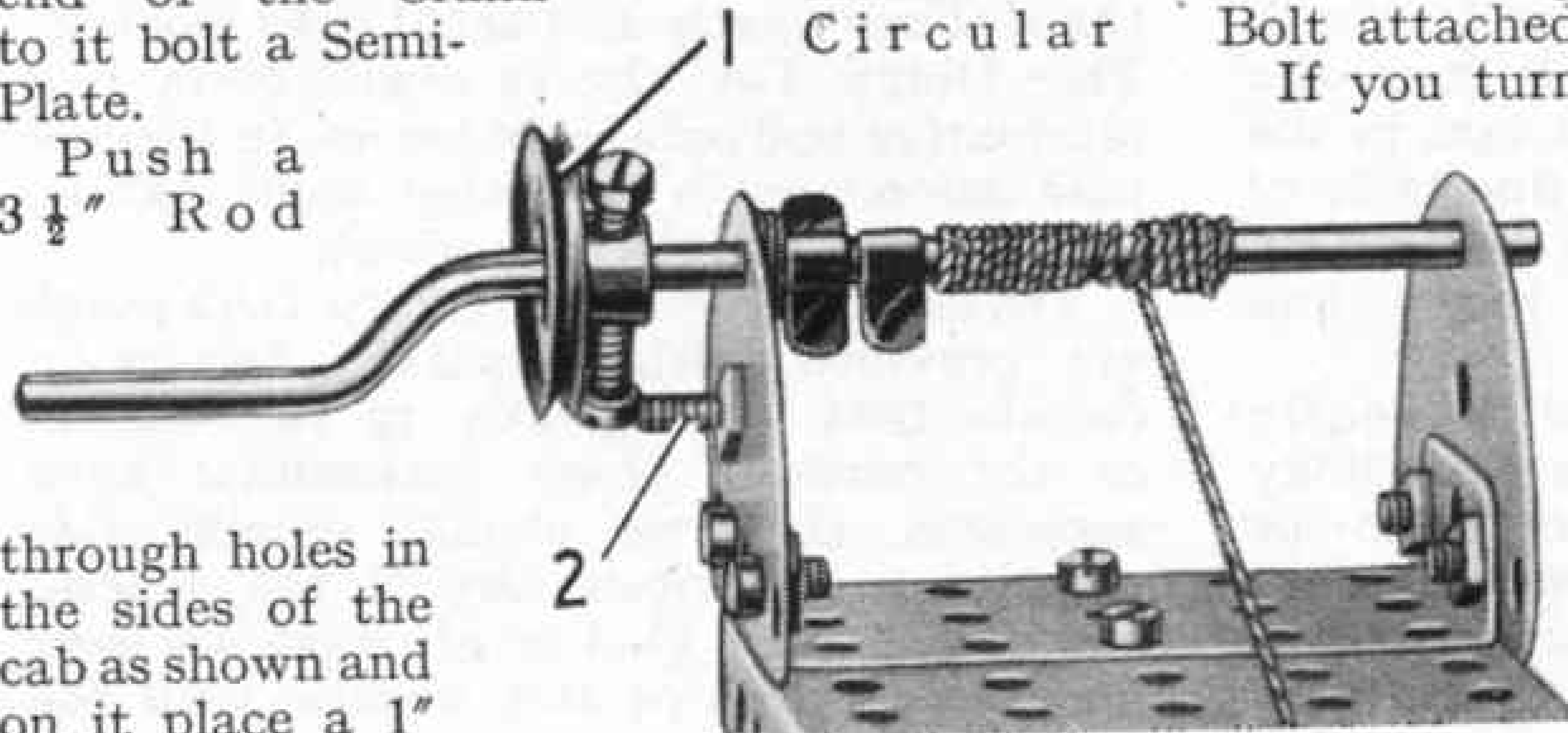
No. 4. This simple mechanism shows an easy way to attach Cord to a Crank Handle, and a simple brake mechanism for small models.
