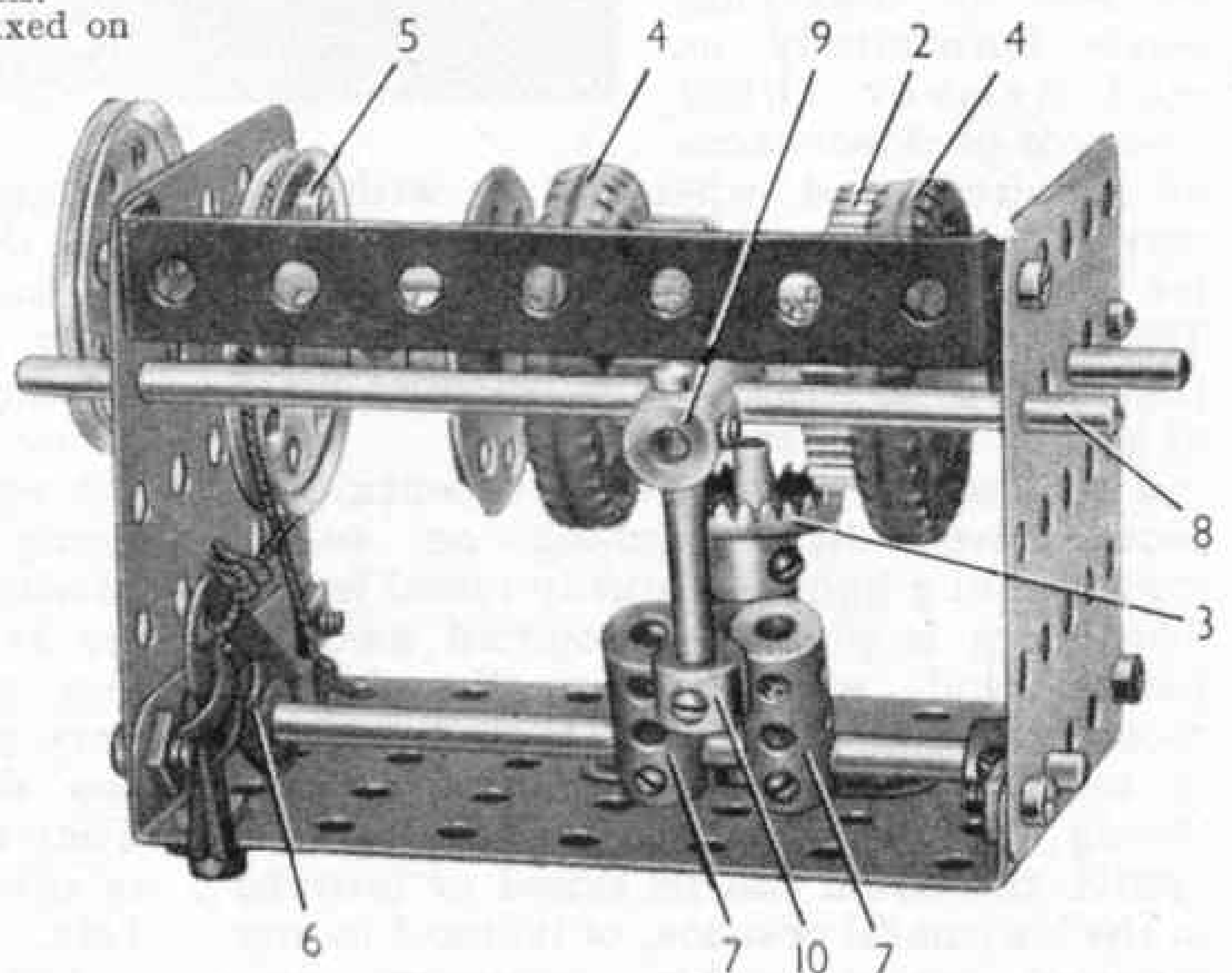
Fig. 4. Another view of the crane winding drum mechanism, showing the lever arrangement that controls the brake automatically.
