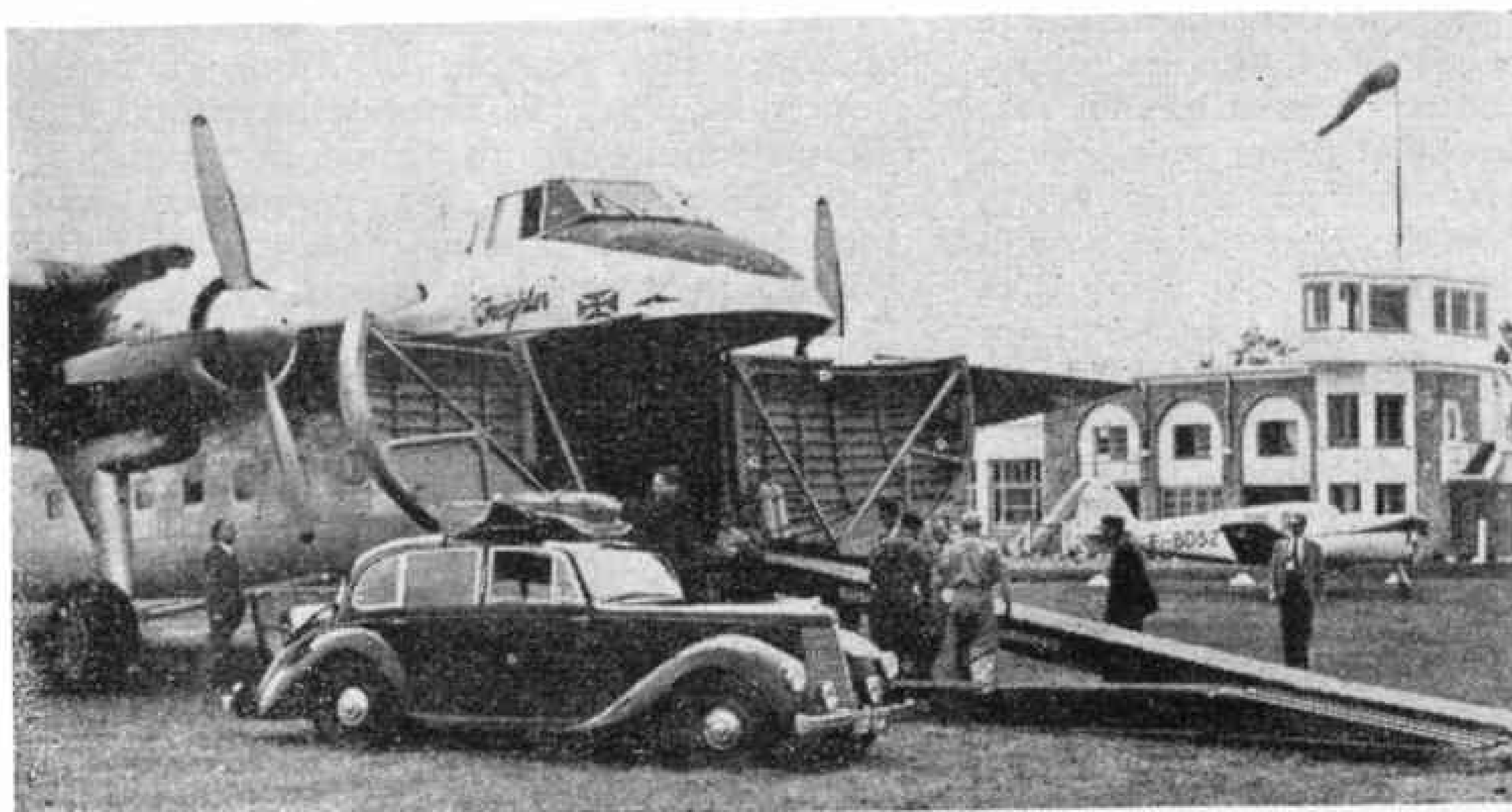
The first motor car ever transported by Silver City's Air Ferry was an Armstrong Siddeley saloon, on 14th July 1948. It is seen here at Le Touquet Airport. Photograph by courtesy of The Bristol Aeroplane Company Limited.
