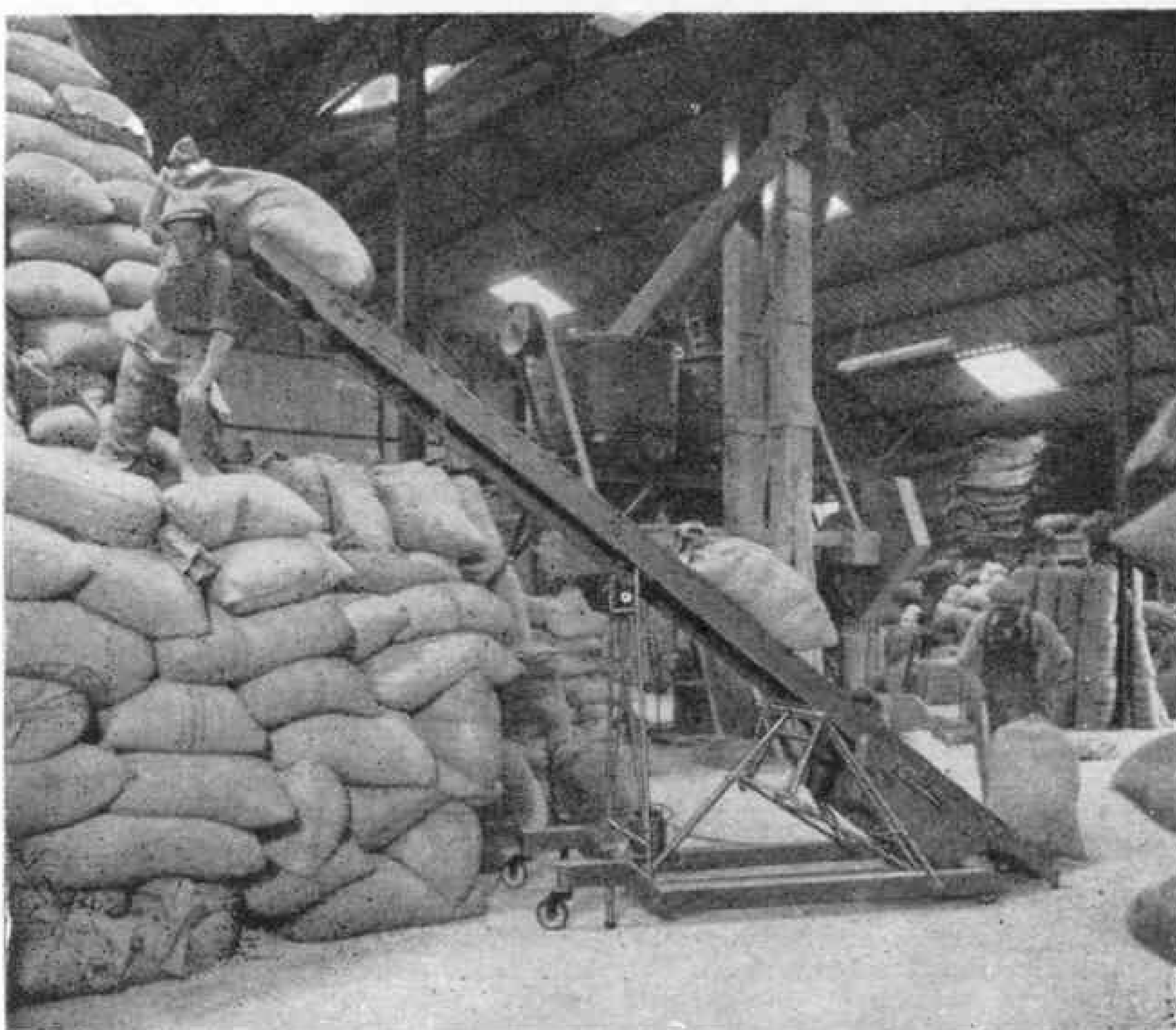
Fig. 1. The LoadaVeyor, with the boom at the maximum angle, in action stacking sacks of animal feeding stuffs.
