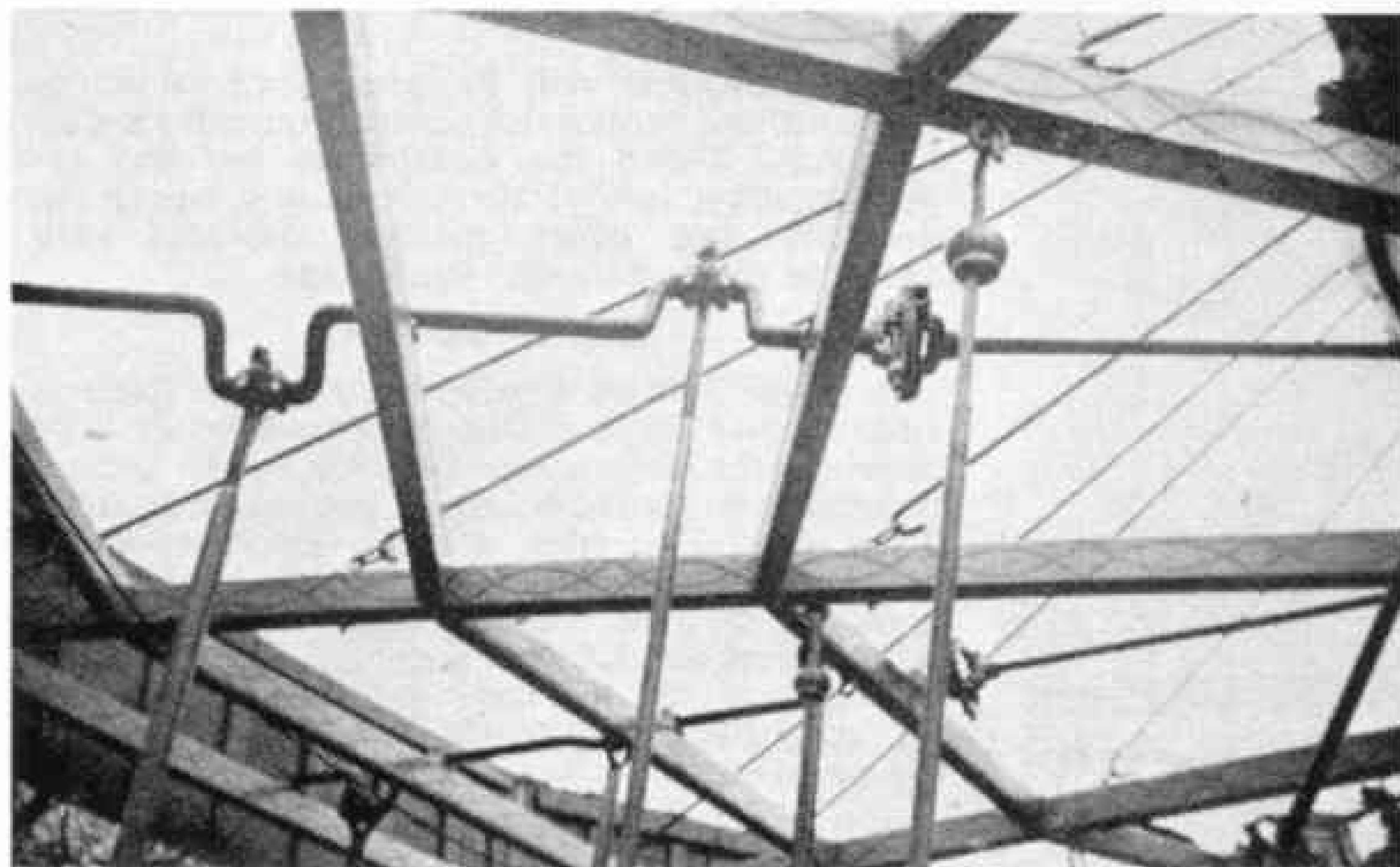
Overhead cranks and crankshafts, with universal joints.
