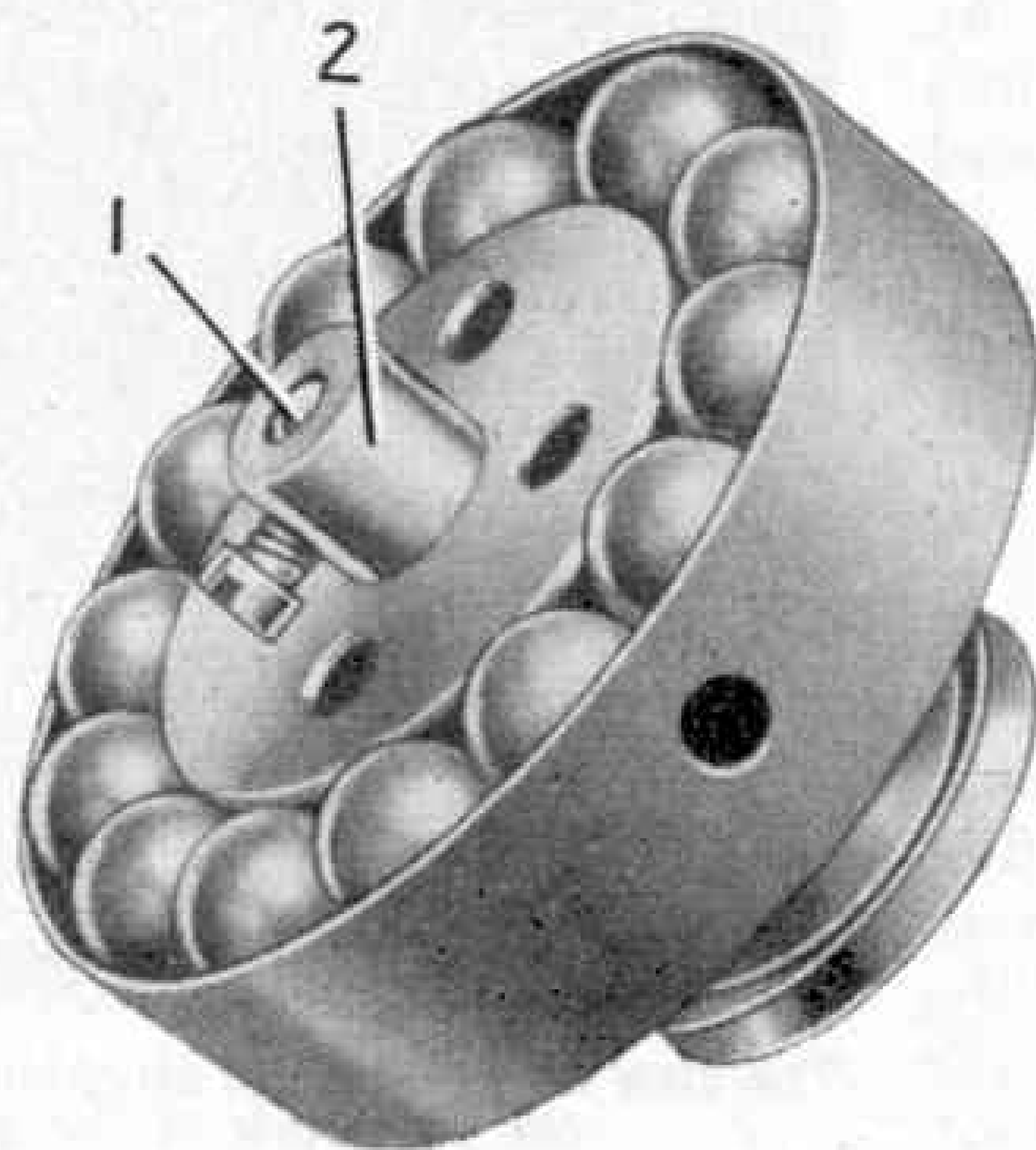
Fig. 2. A useful built-up ball bearing unit.
