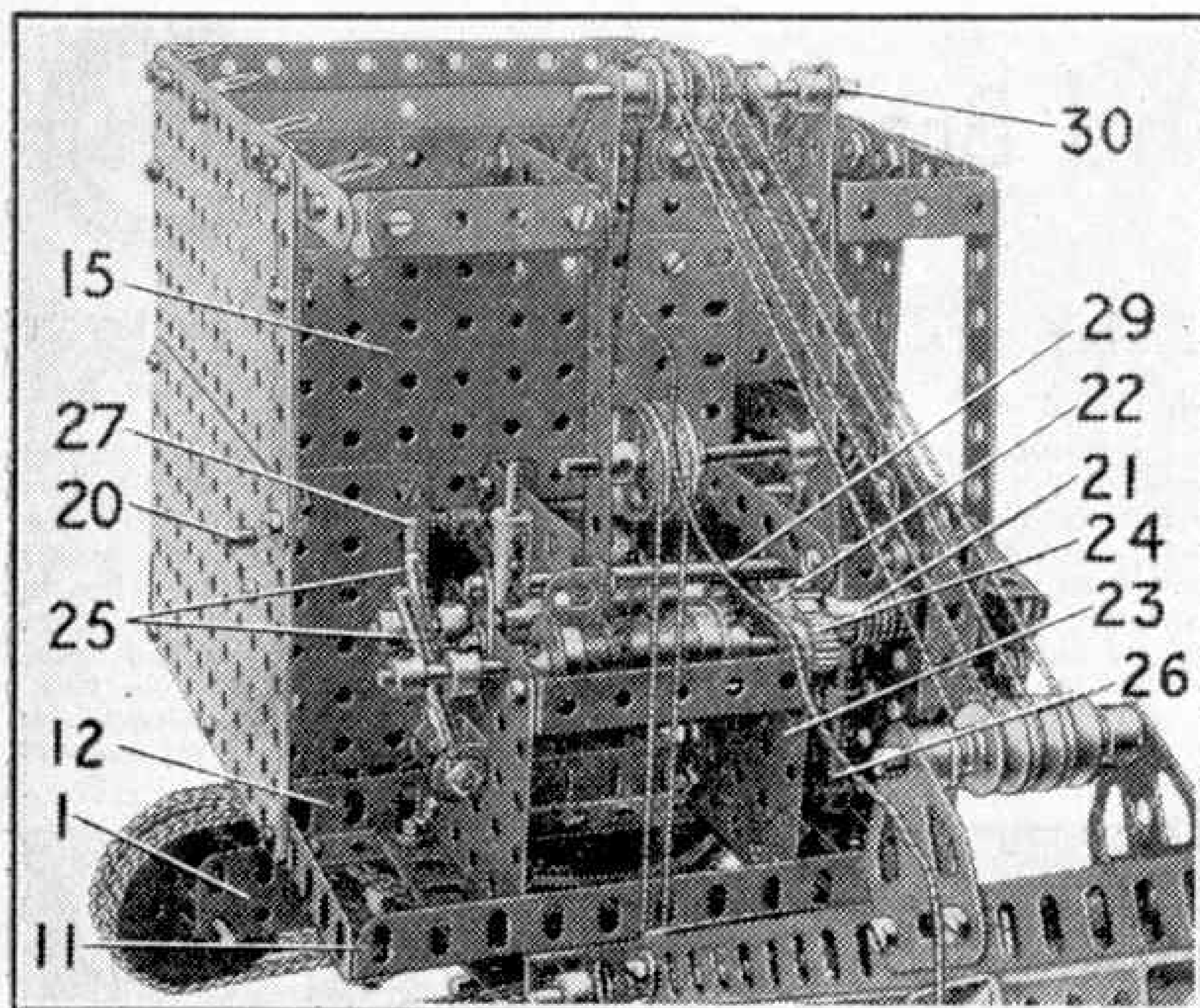
Fig. 3. The mechanism of the shovel is shown here, with the controls for swivelling, luffing and other movements.
