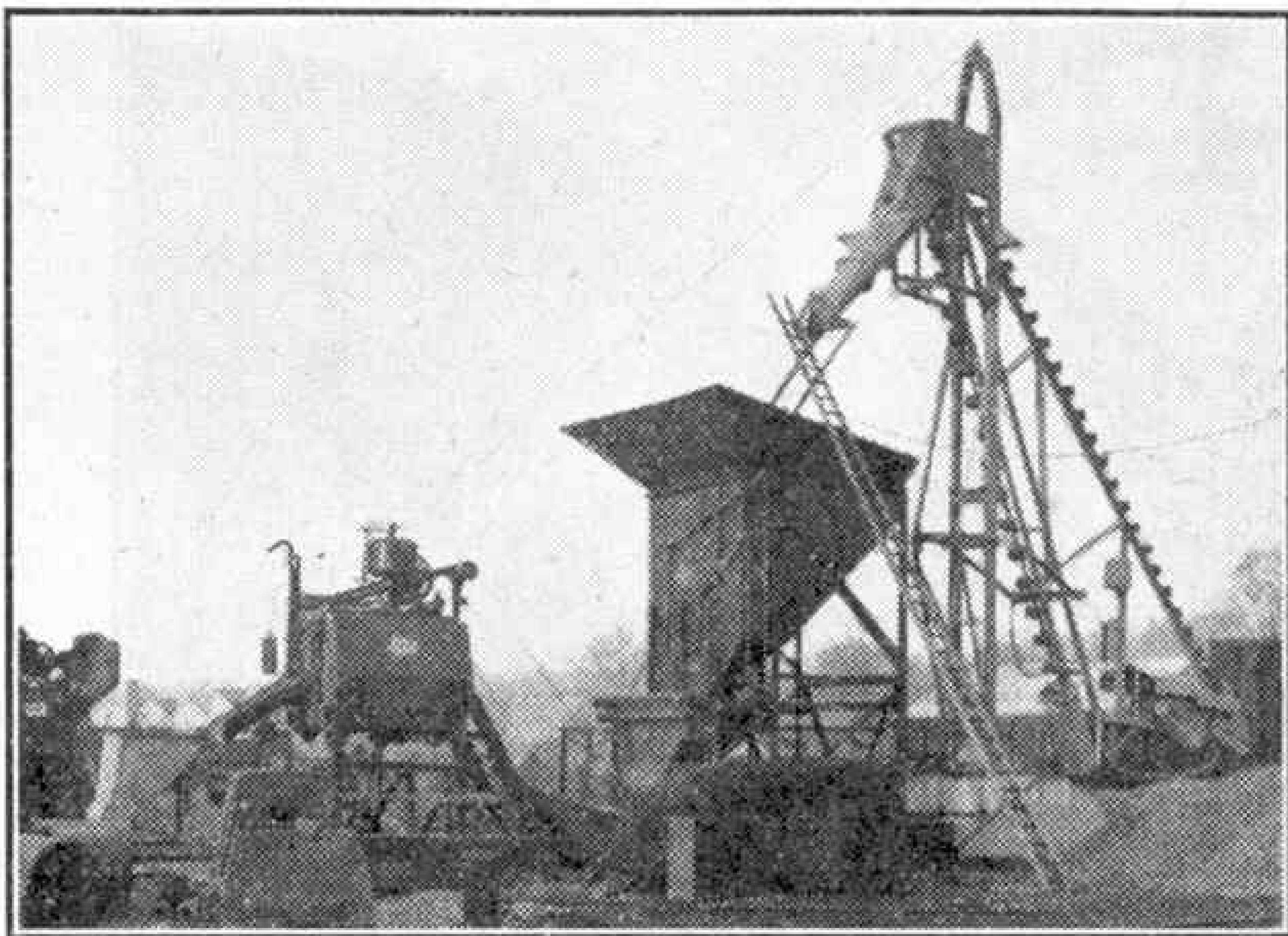
Fig. 7. Concrete mixing plant.
