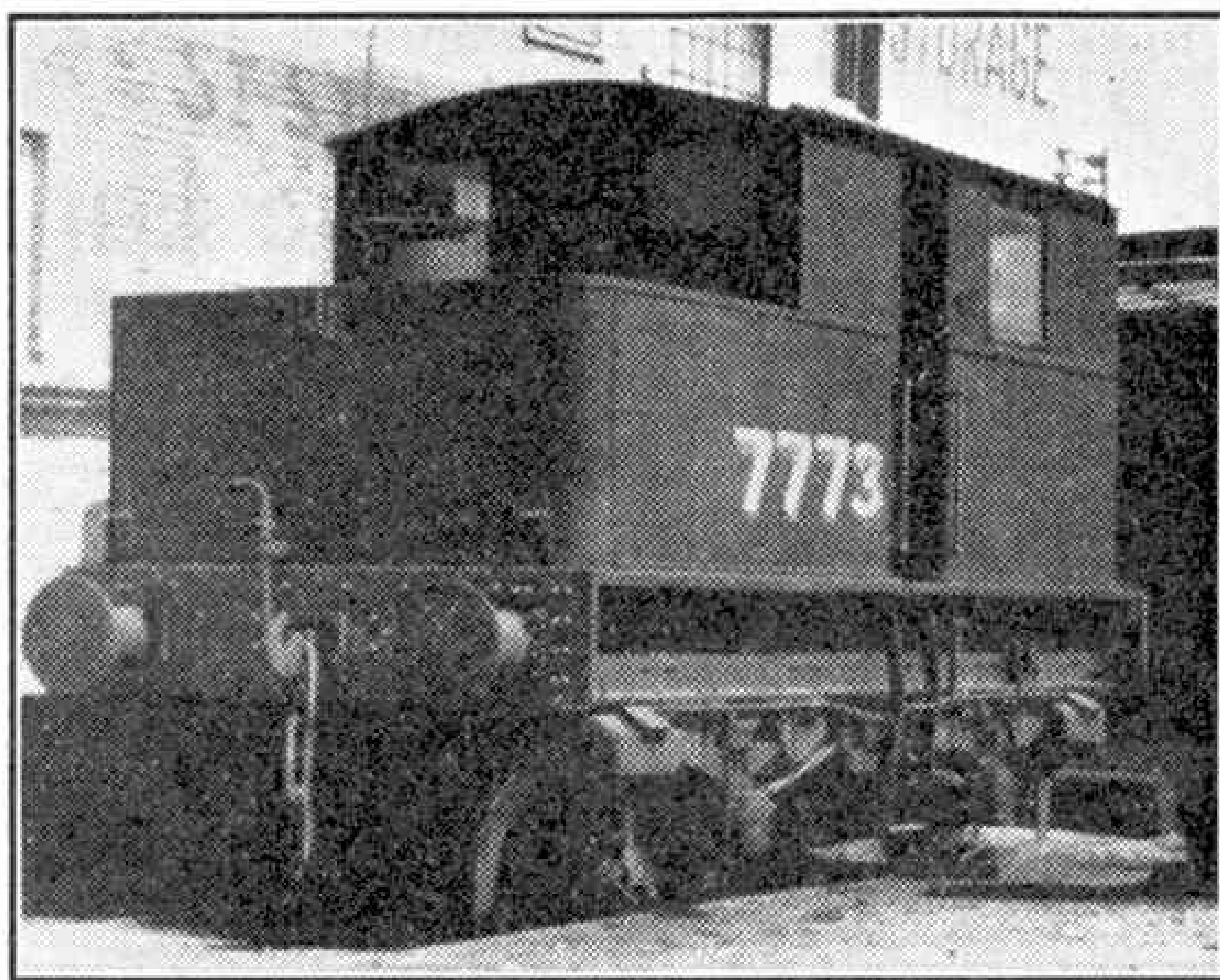
"Sentinel" locomotive No. 7773 at Lowestoft is used for duties in the Engineer's Yard and the docks.
