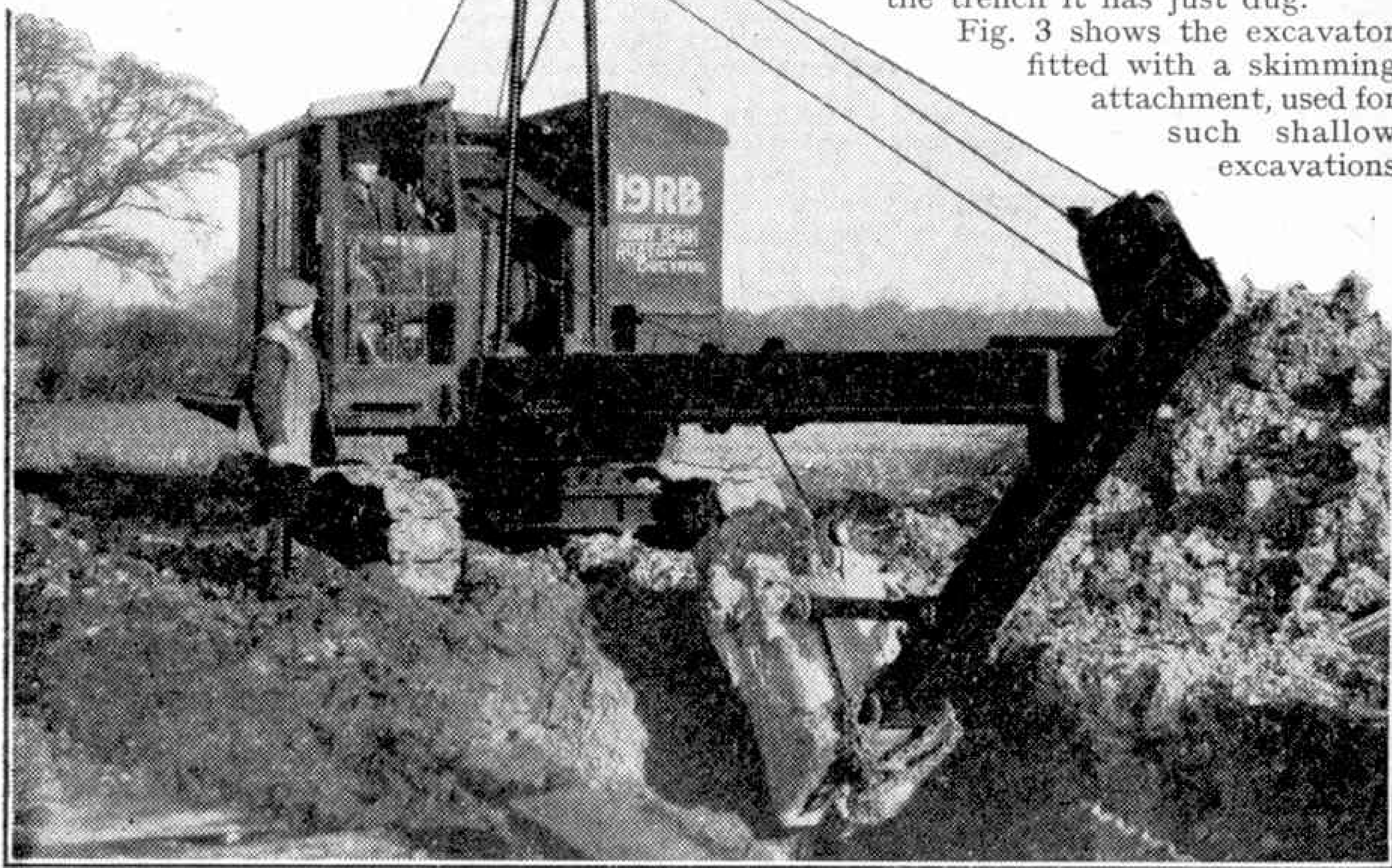
Fig. 1. Mechanical excavator working as a "back acter."
