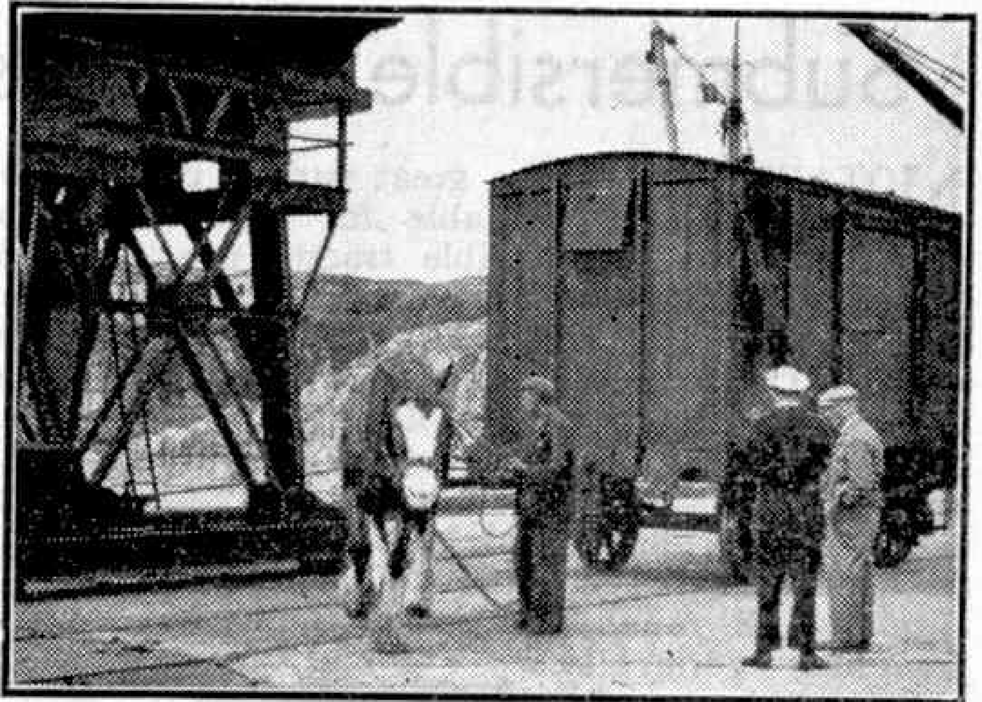
Motive Power! Horses are frequently used, as here at Kyle of Lochalsh, for shunting purposes on dock lines and wharves. Photograph by E. S. B. Elcome, Woking.
