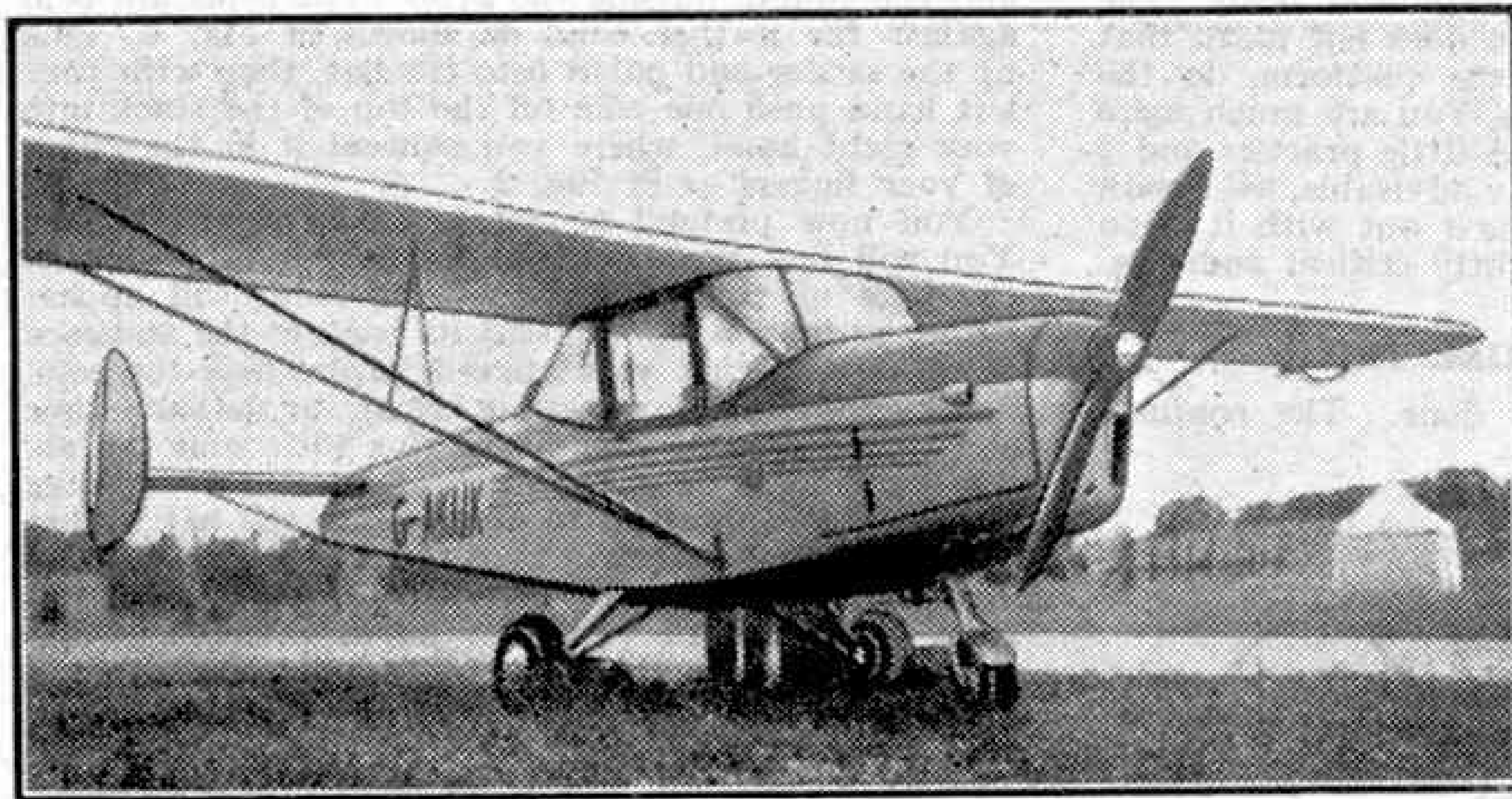
The Chrislea "Super Ace," a very promising British four-seater light aeroplane now in quantity production.
