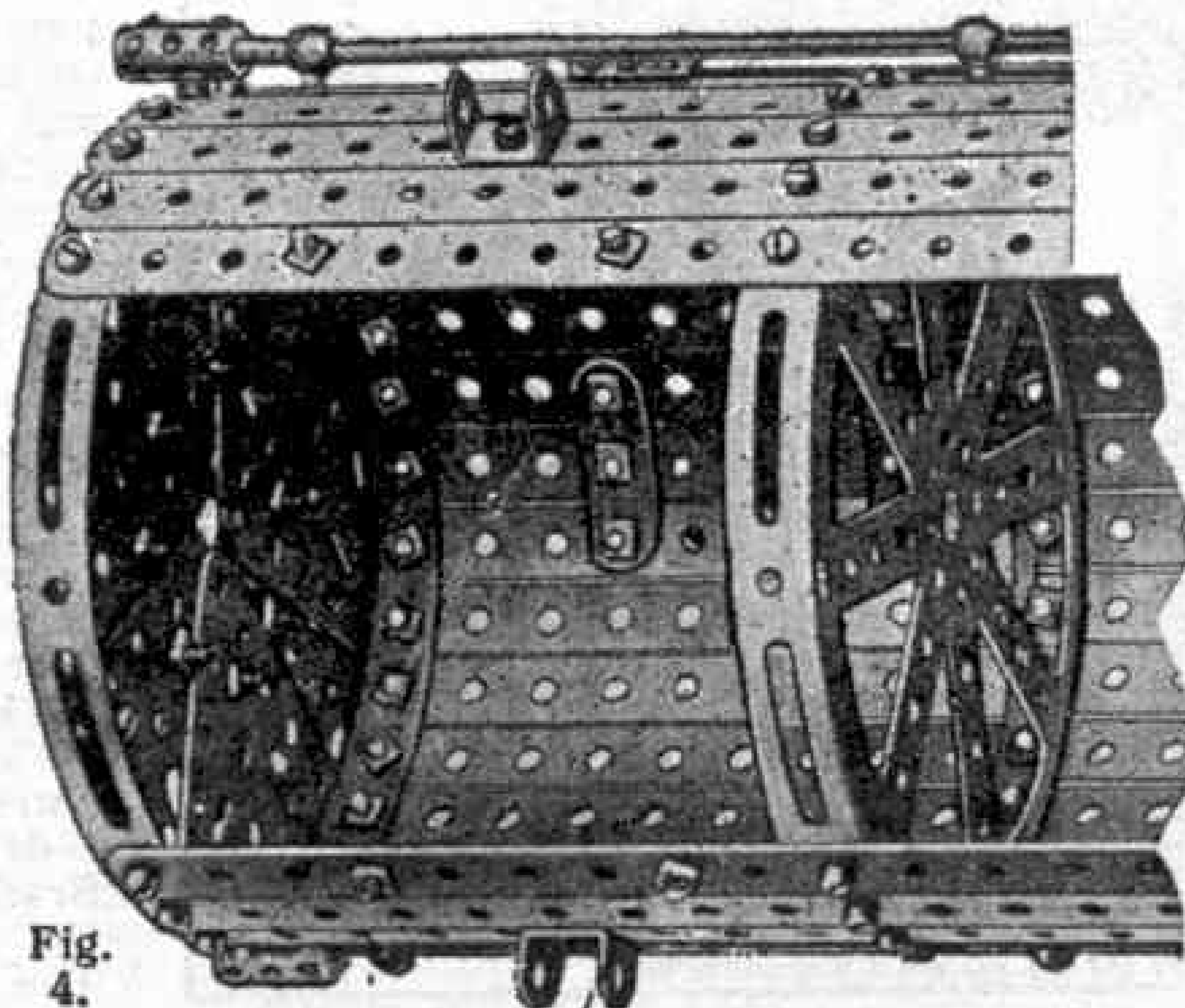
Figs. 3 and 4 above show typical uses for the Meccano Wheel Flange and Hub Disc respectively.
