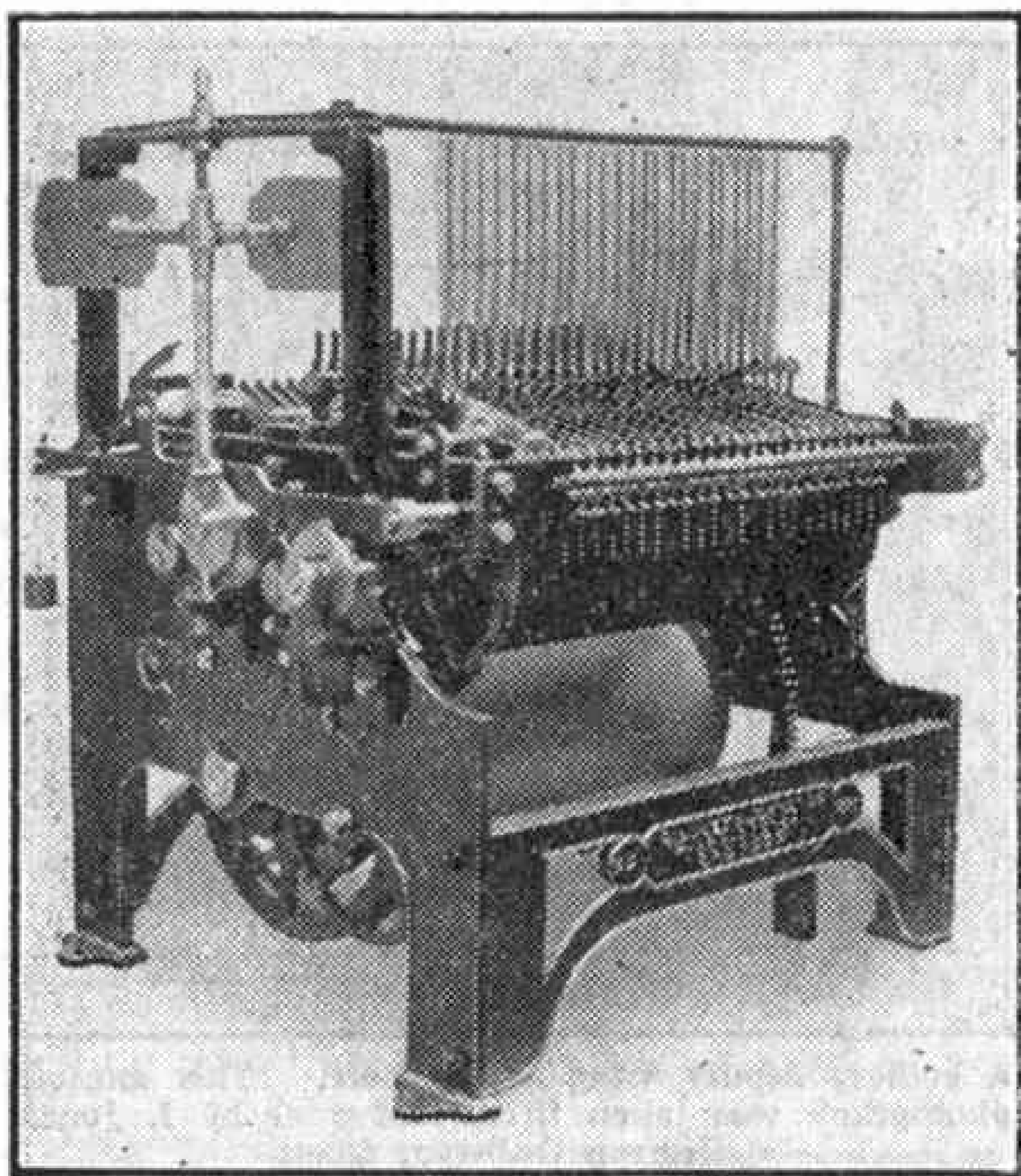
A carillon tune-playing machine.
