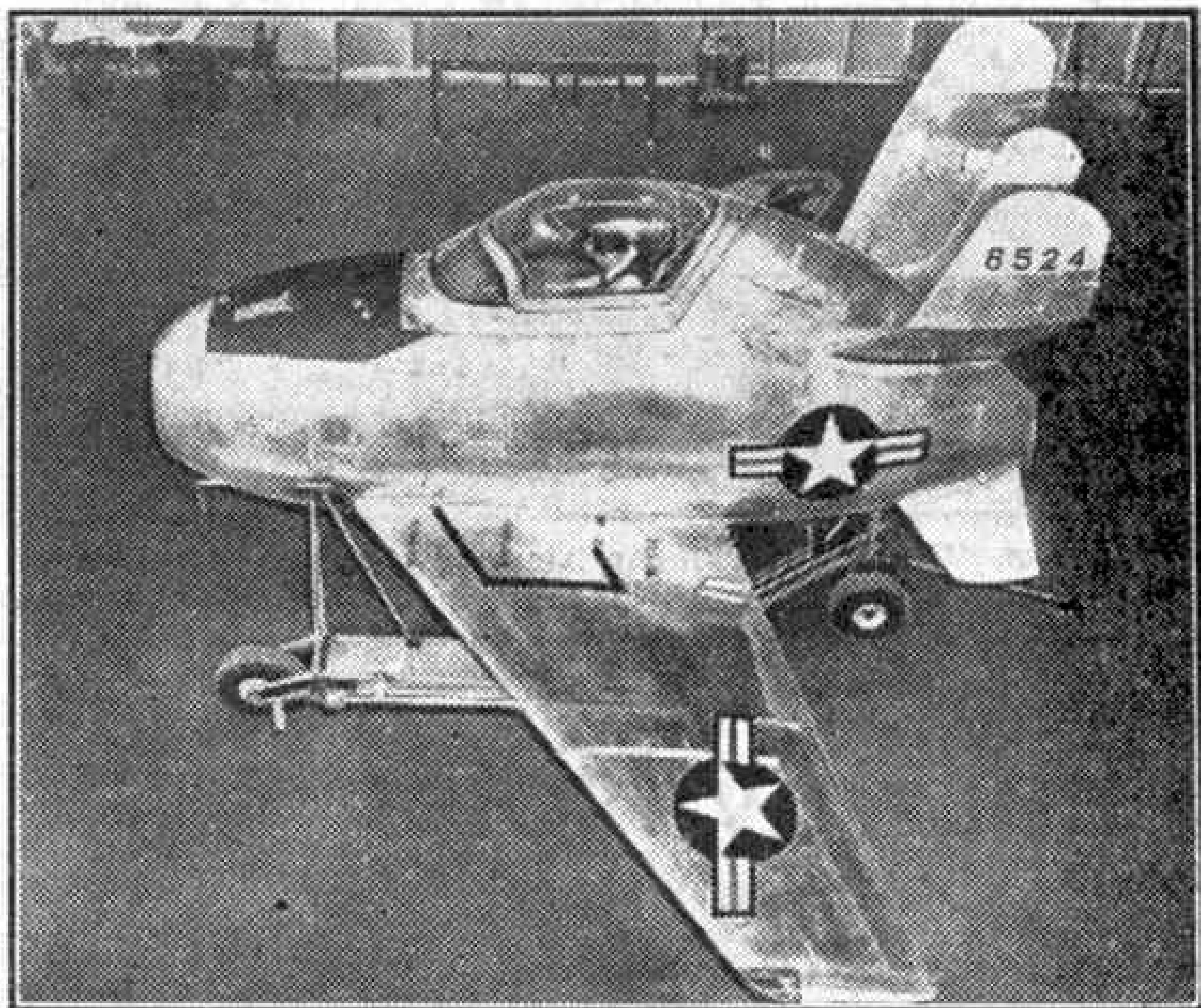
The McDonnell XF-85 Parasite fighter, designed to fit into the bomb-bay of a Convair B-36 bomber. Photograph by courtesy of the United States Air Force.
