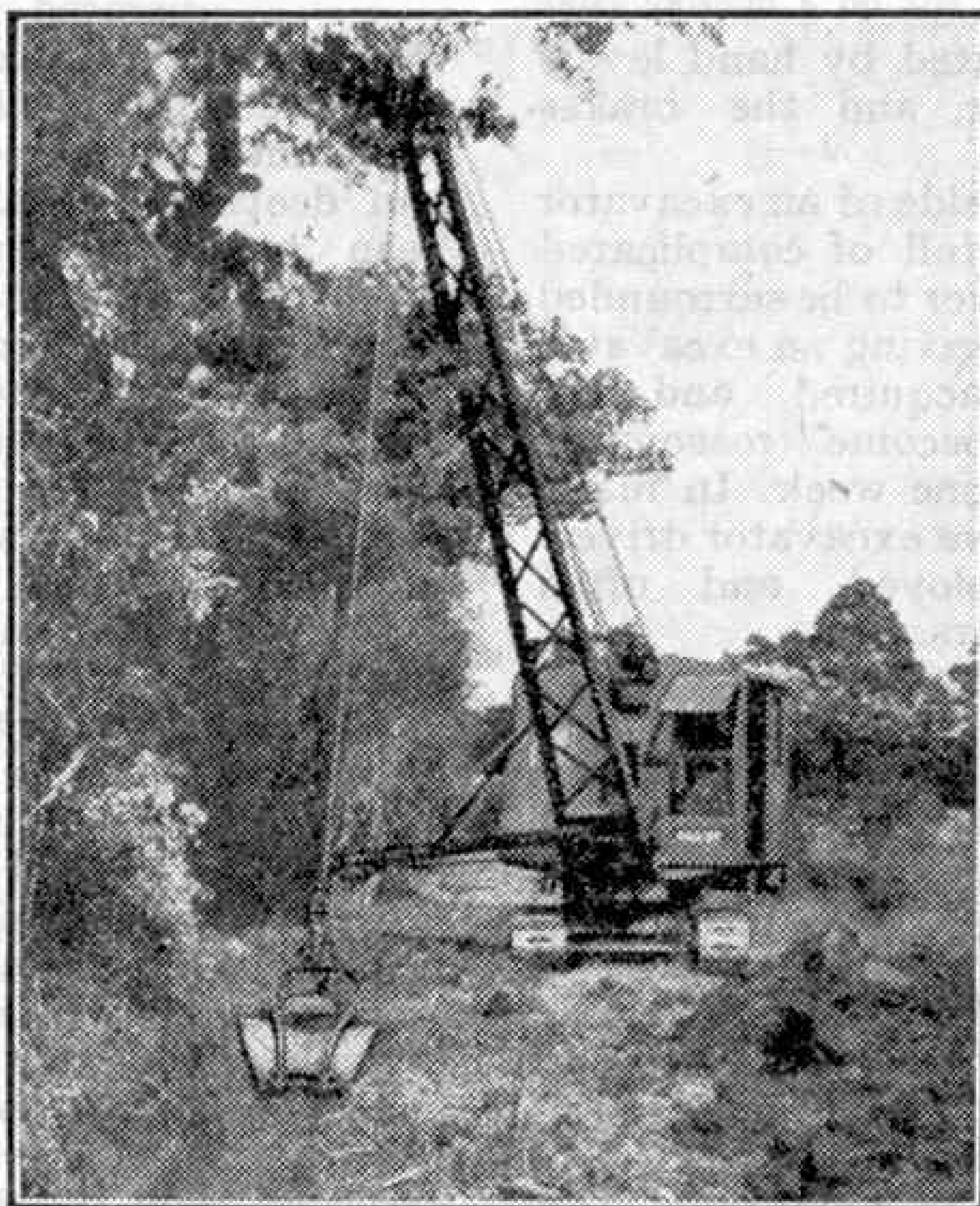
"Cub" excavator, weighing 8½ tons, with Side Dragline attachment. For the illustrations to this article we are indebted to Priestman Bros. Ltd., of Hull, manufacturers of the Universal Excavators shown.
