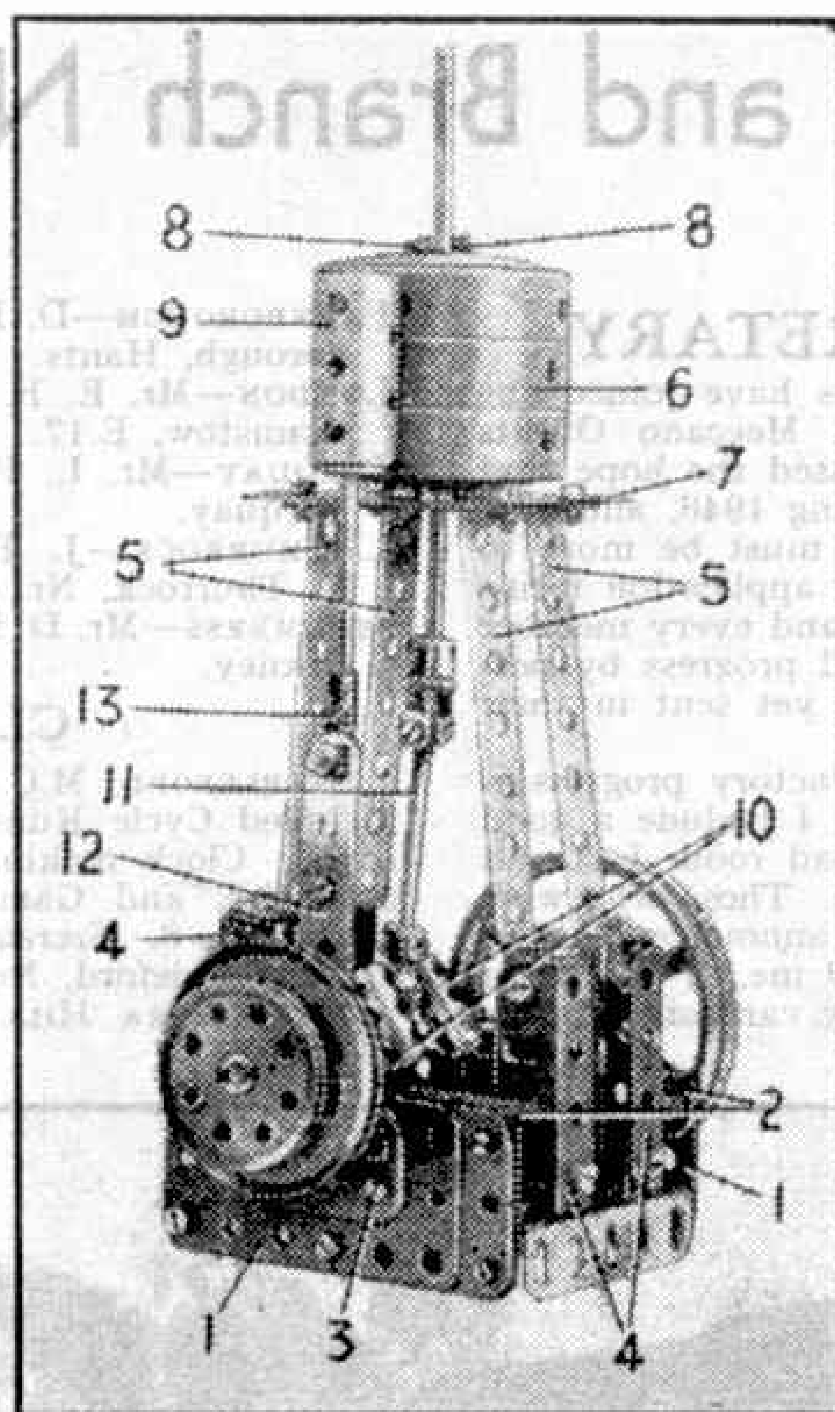
Fig. 2. Simple Vertical Engine.
