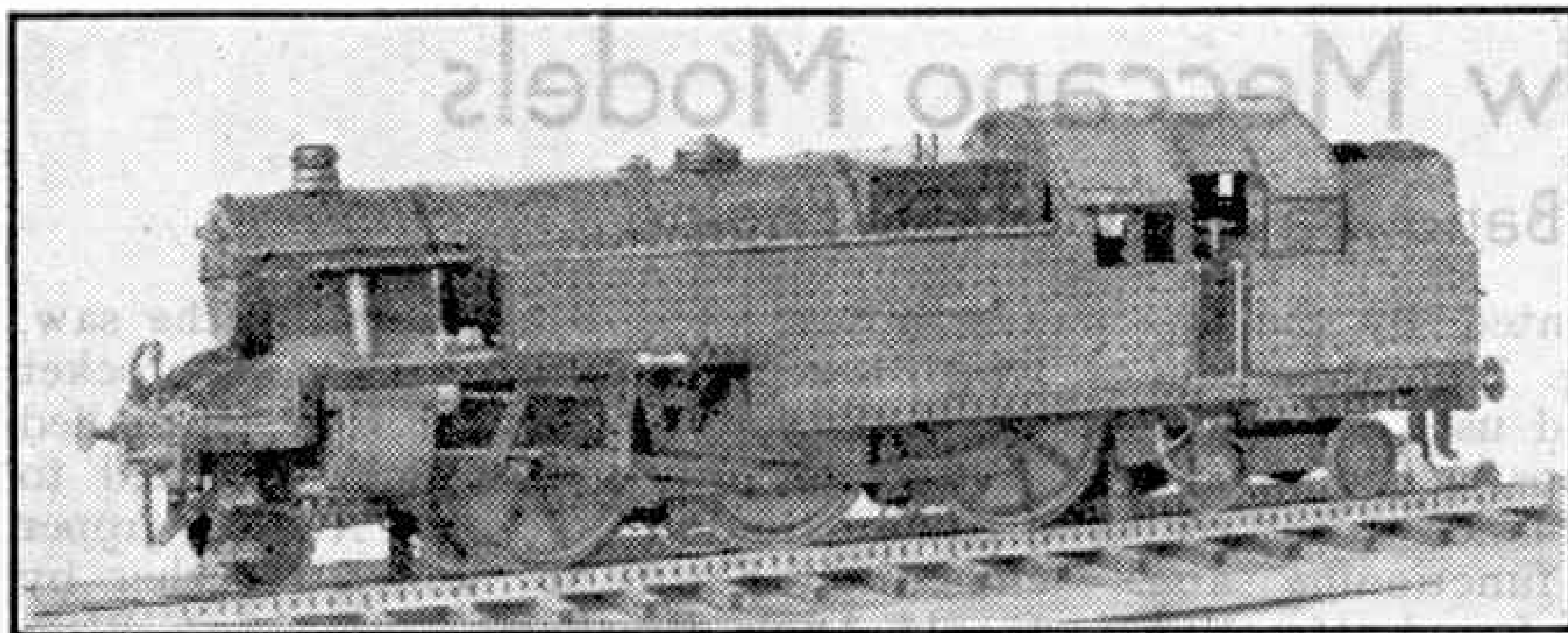
Fig. 3. This realistic model of an L.M.S. 2-6-4 tank locomotive was built by C. Howard, Pendlebury, Hinckley.
