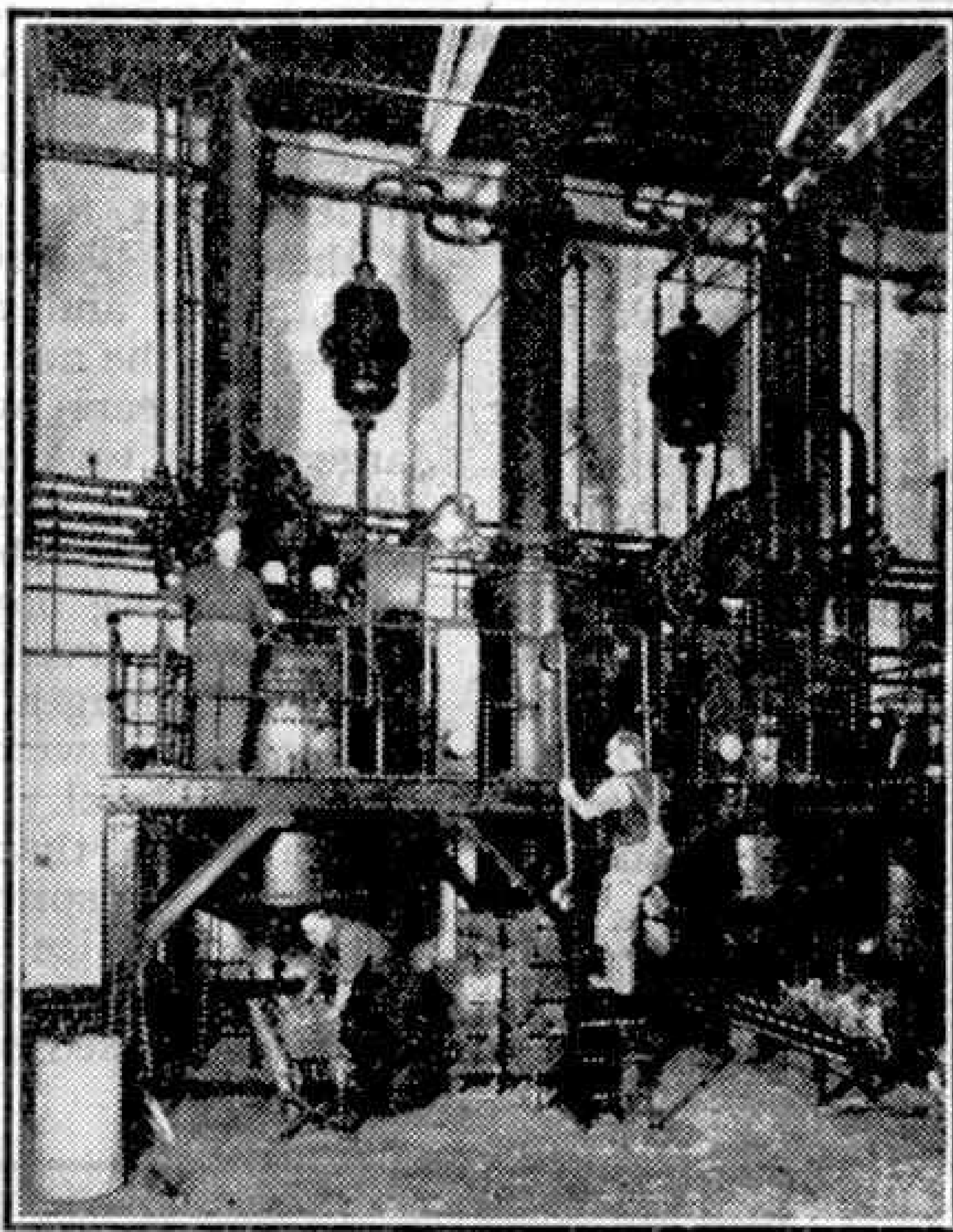
Digesters for the manufacture of synthetic resins. The illustrations to this article were taken at the Elo Works of Birkbys Ltd., Liversedge, Yorks.
