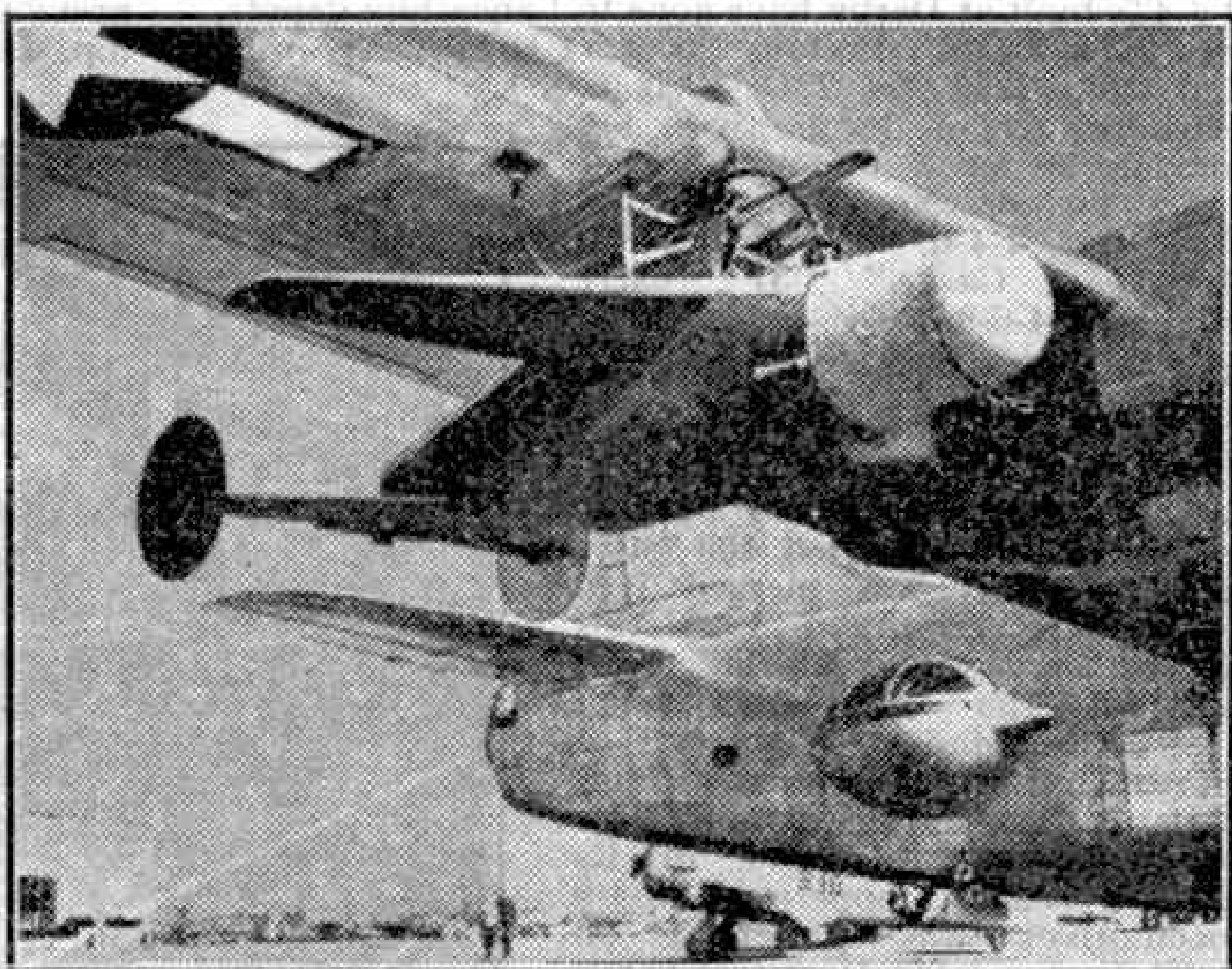
The U.S. Navy's radar-guided "Bat" bomb slung under the wing of a "Privateer" patrol bomber. The machine carries one of these bombs under each wing.
