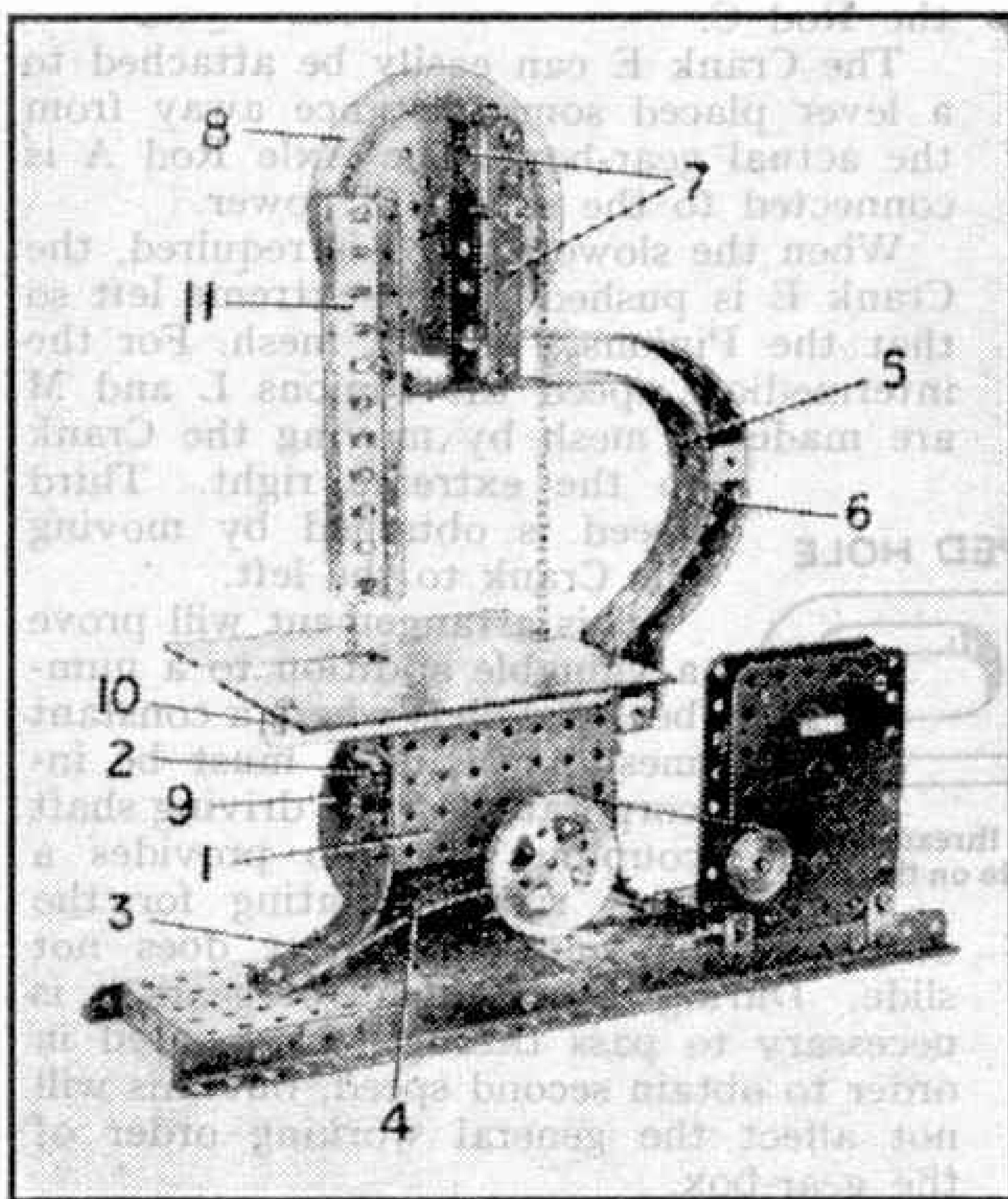
Fig. 1. Band Saw.
