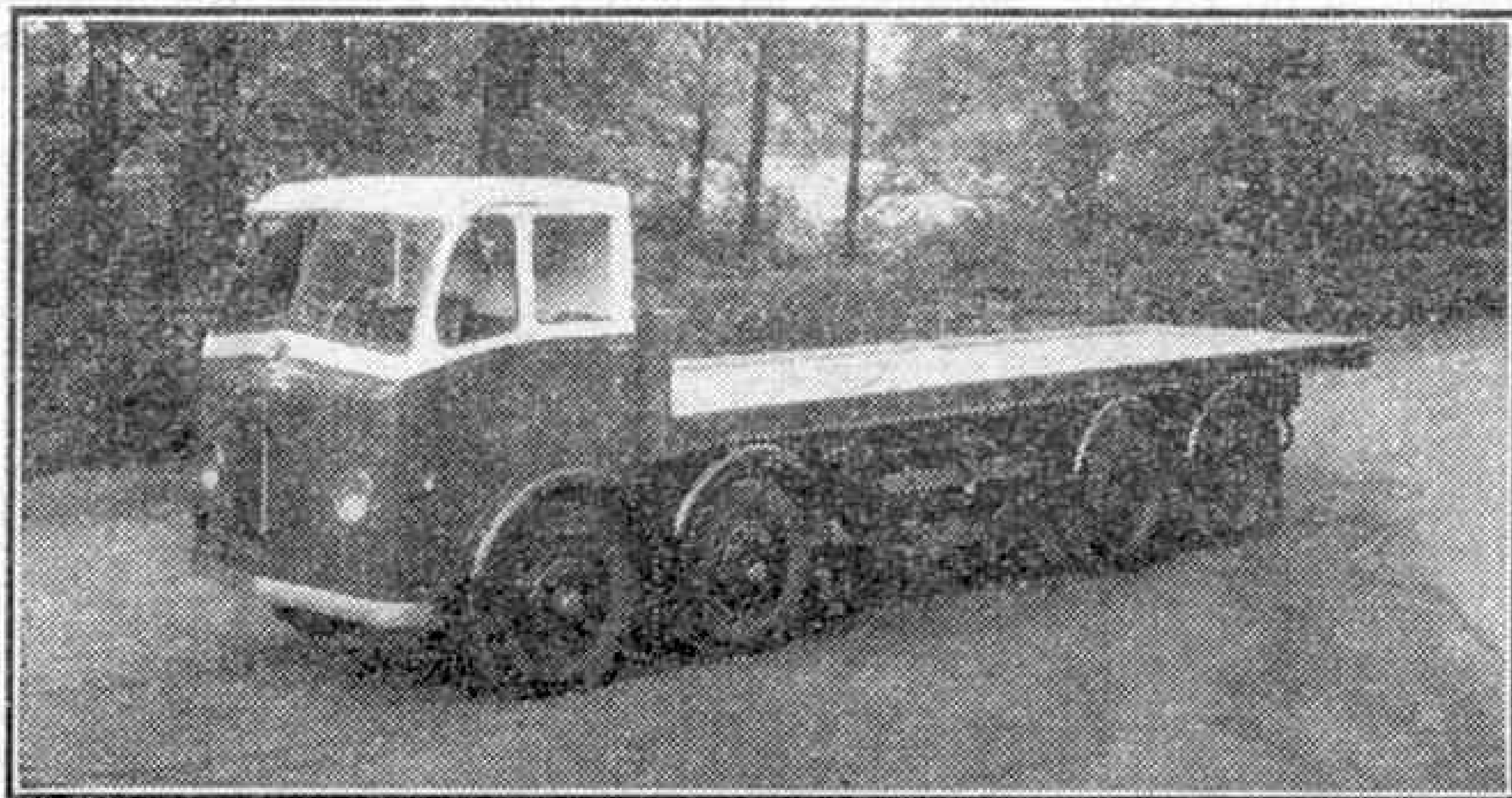
The Leyland "Octopus." Photograph by courtesy of Leyland Motors Ltd.
