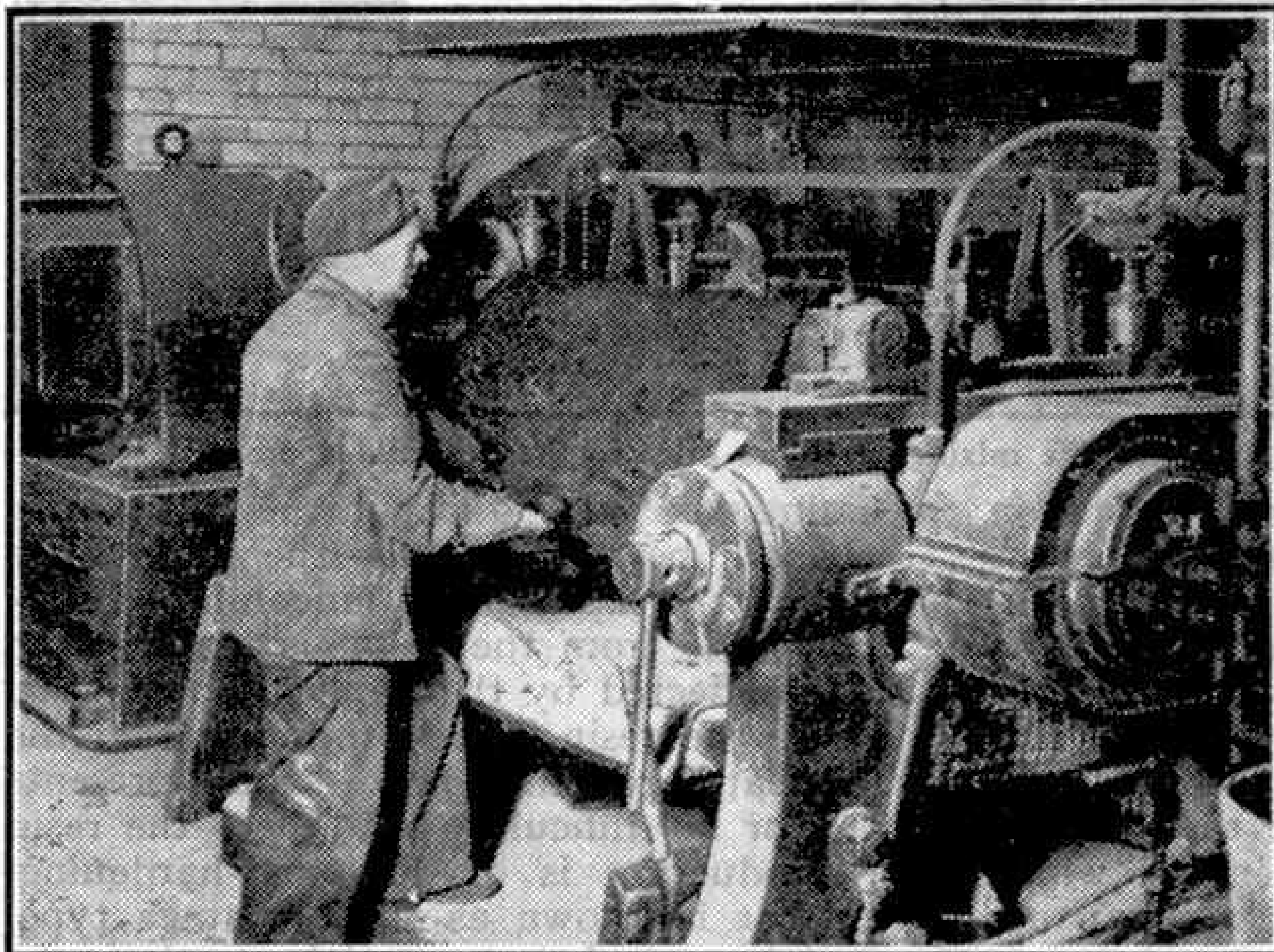
Blanket of phenolic material coming off the hot kneading rolls.
