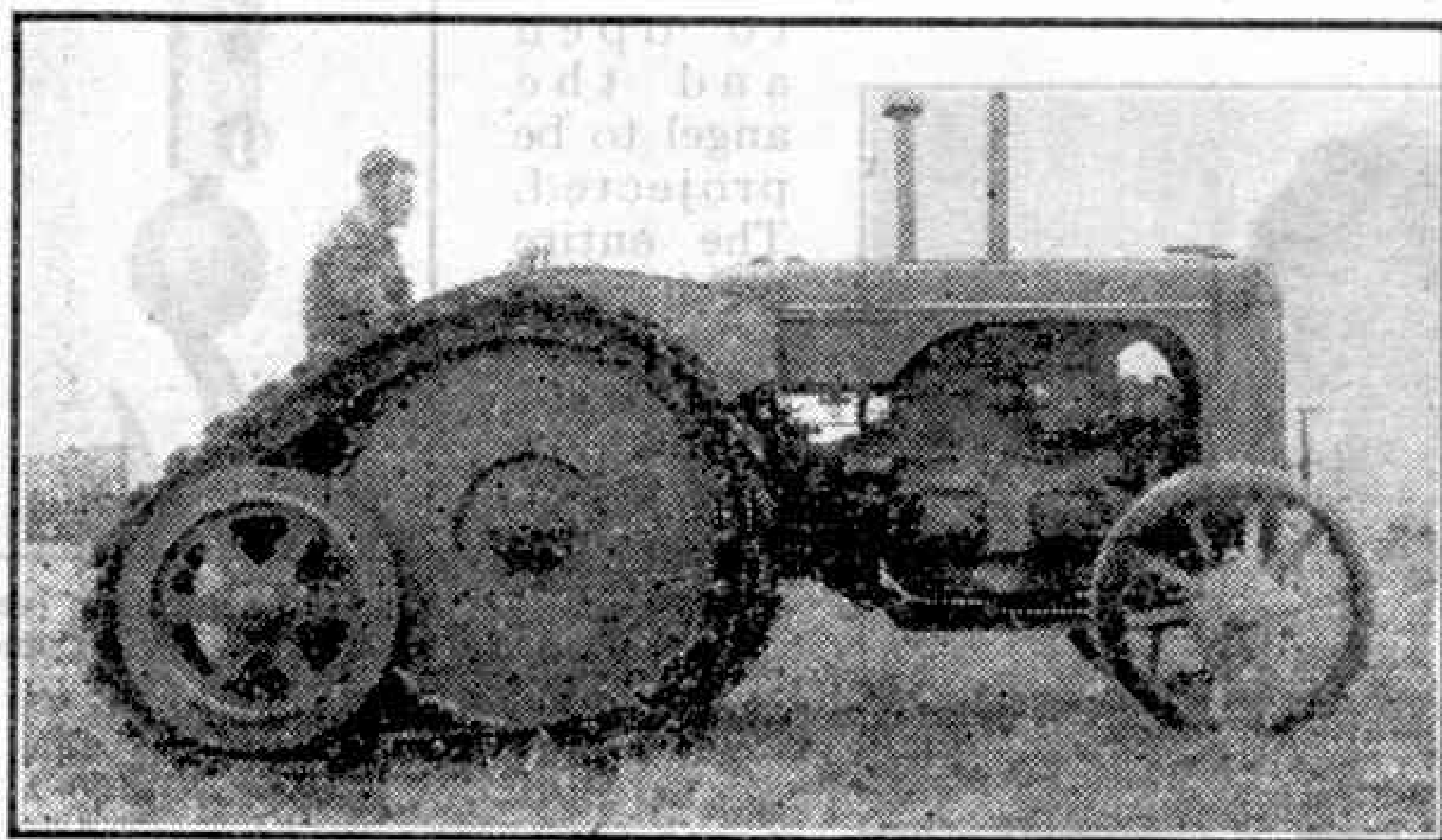
A tractor mounted on type D.G. track equipment. For this illustration and the one below we are indebted to Roadless Traction Ltd., Hounslow.
