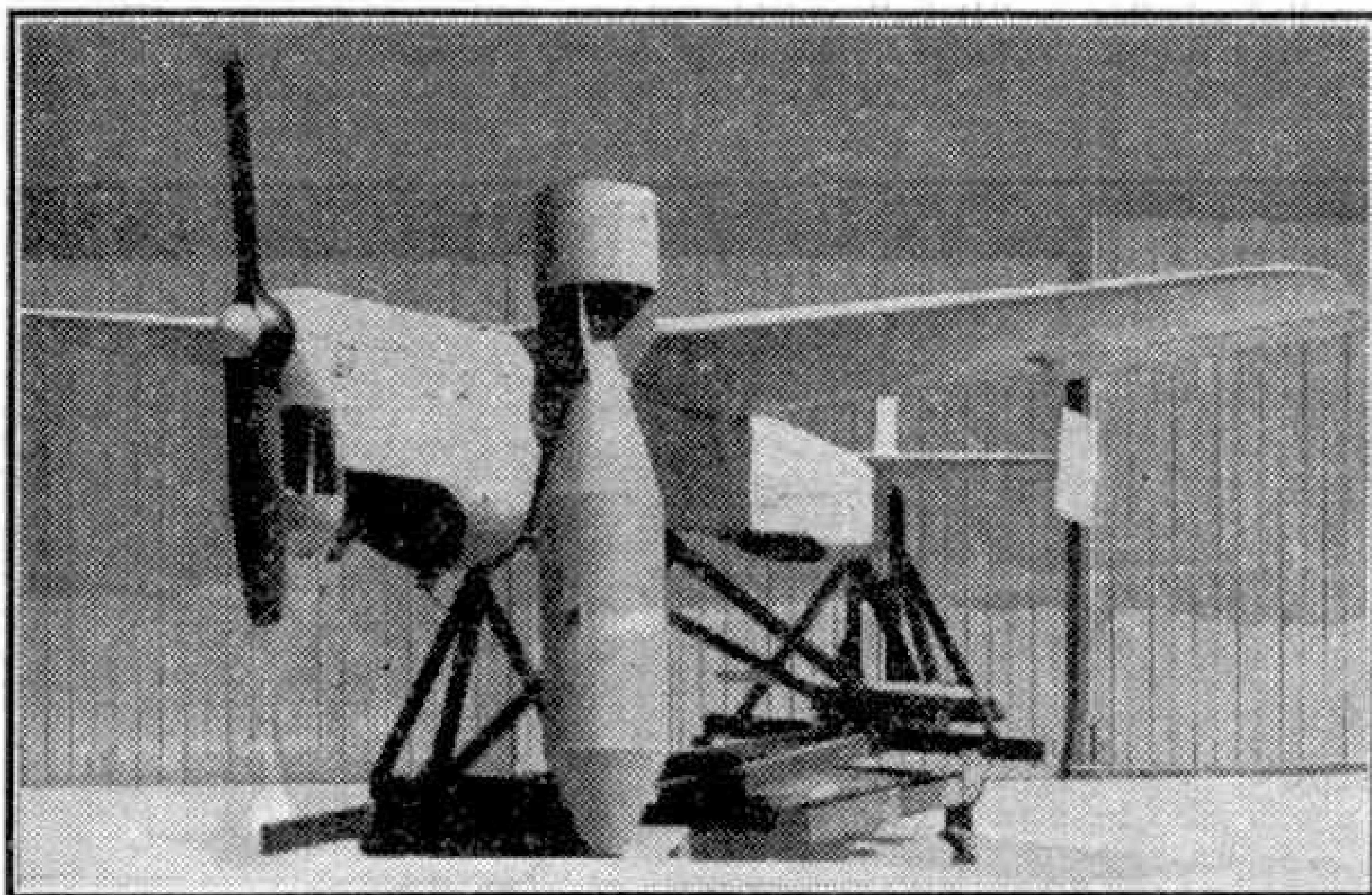
Miles "Hoopla." The underside of the fuselage is cut away to accommodate the 1,000 lb. bomb. Photograph by courtesy of Miles Aircraft Ltd.
