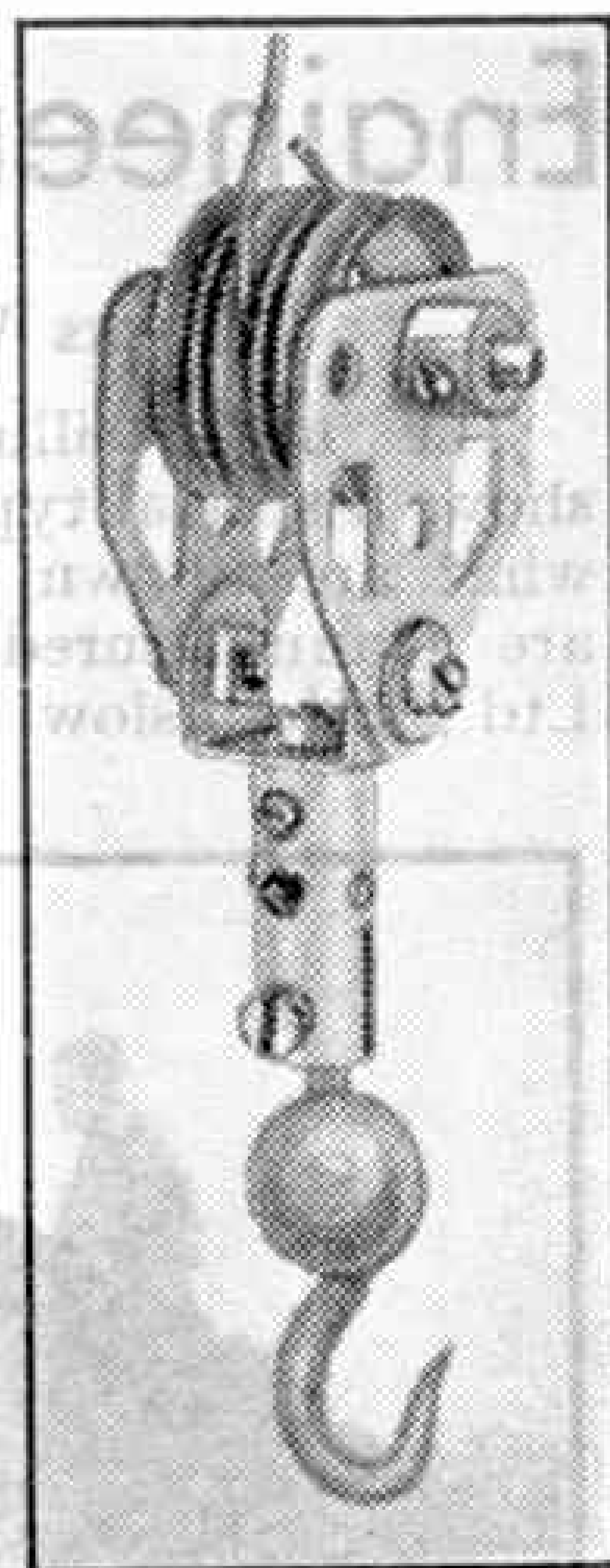
Fig. 1. A built-up load hook for a crane.
