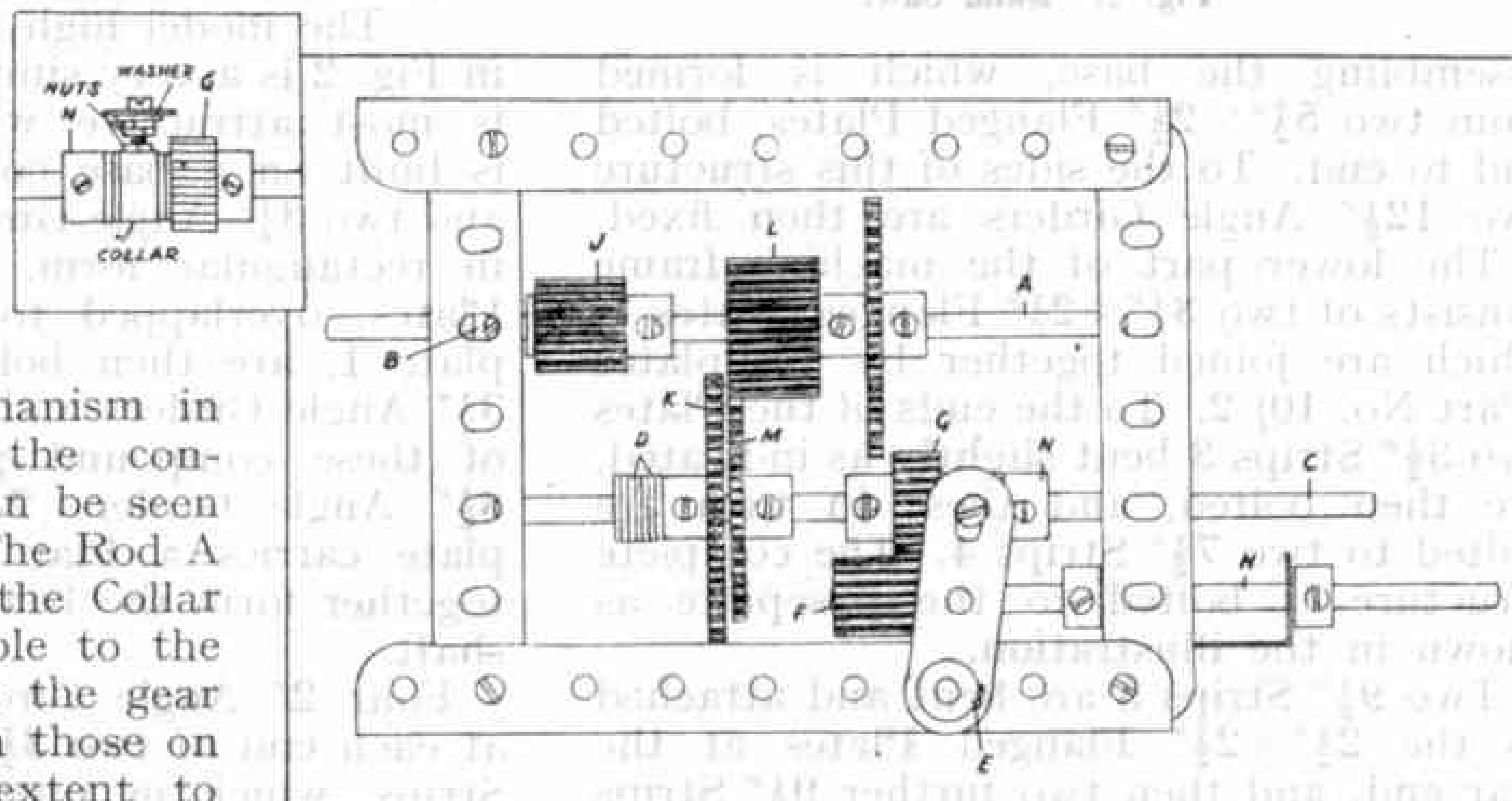
Fig. 5. An interesting three-speed gear-box designed by P. Horne, Johannesburg.
