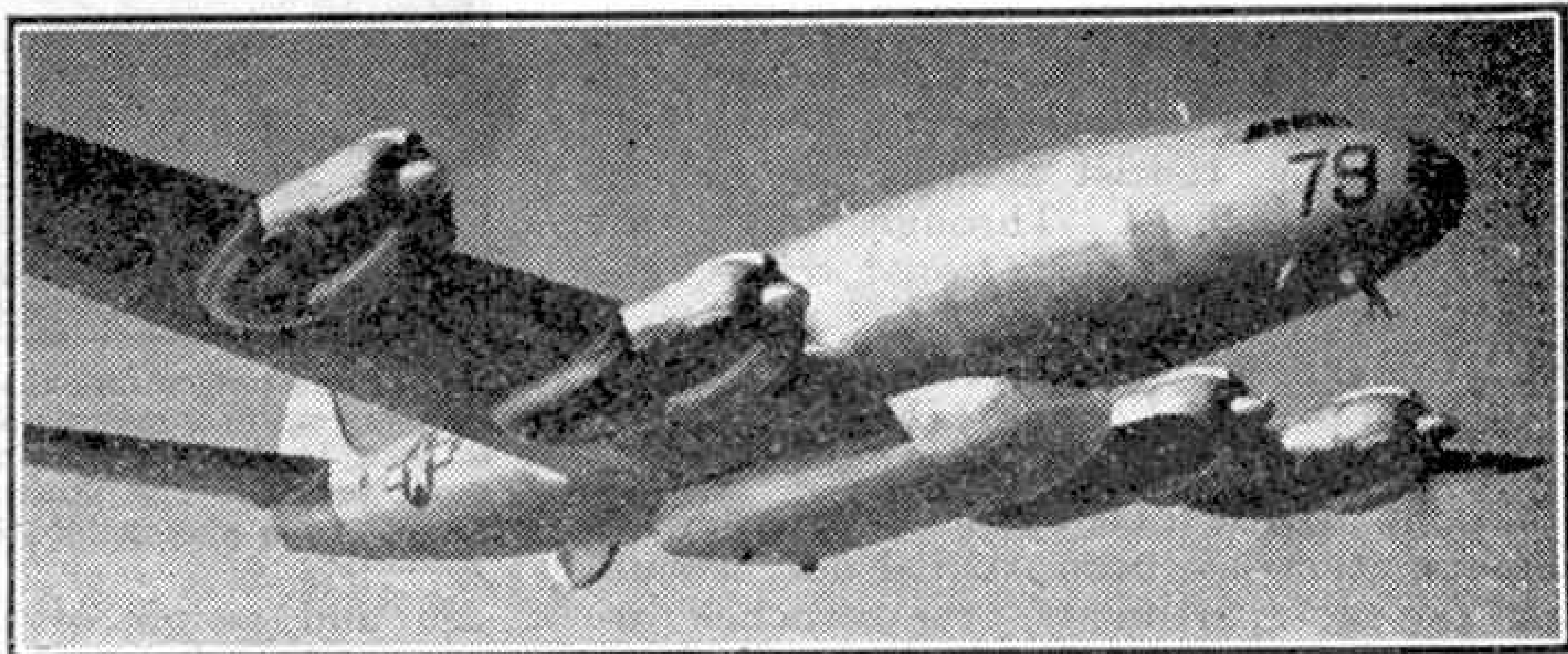
When fitted with a "Speedpak" external carrier under the centre of the fuselage, as shown here, the "Constellation" transport can carry almost double its original load. Photograph by courtesy of the Lockheed Aircraft Corporation, U.S.A.
