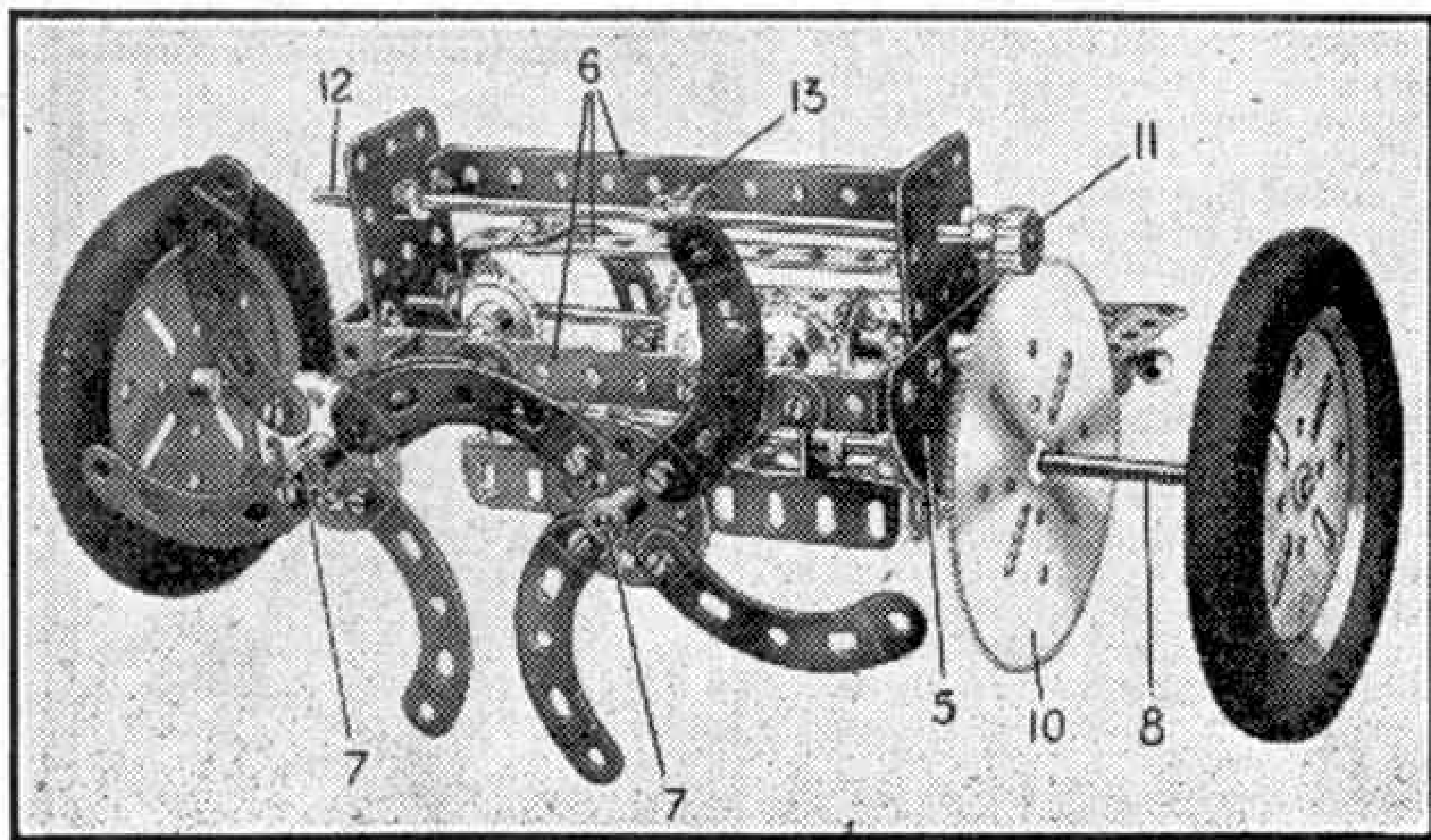
Fig. 2. Rear view of the hay turner.
