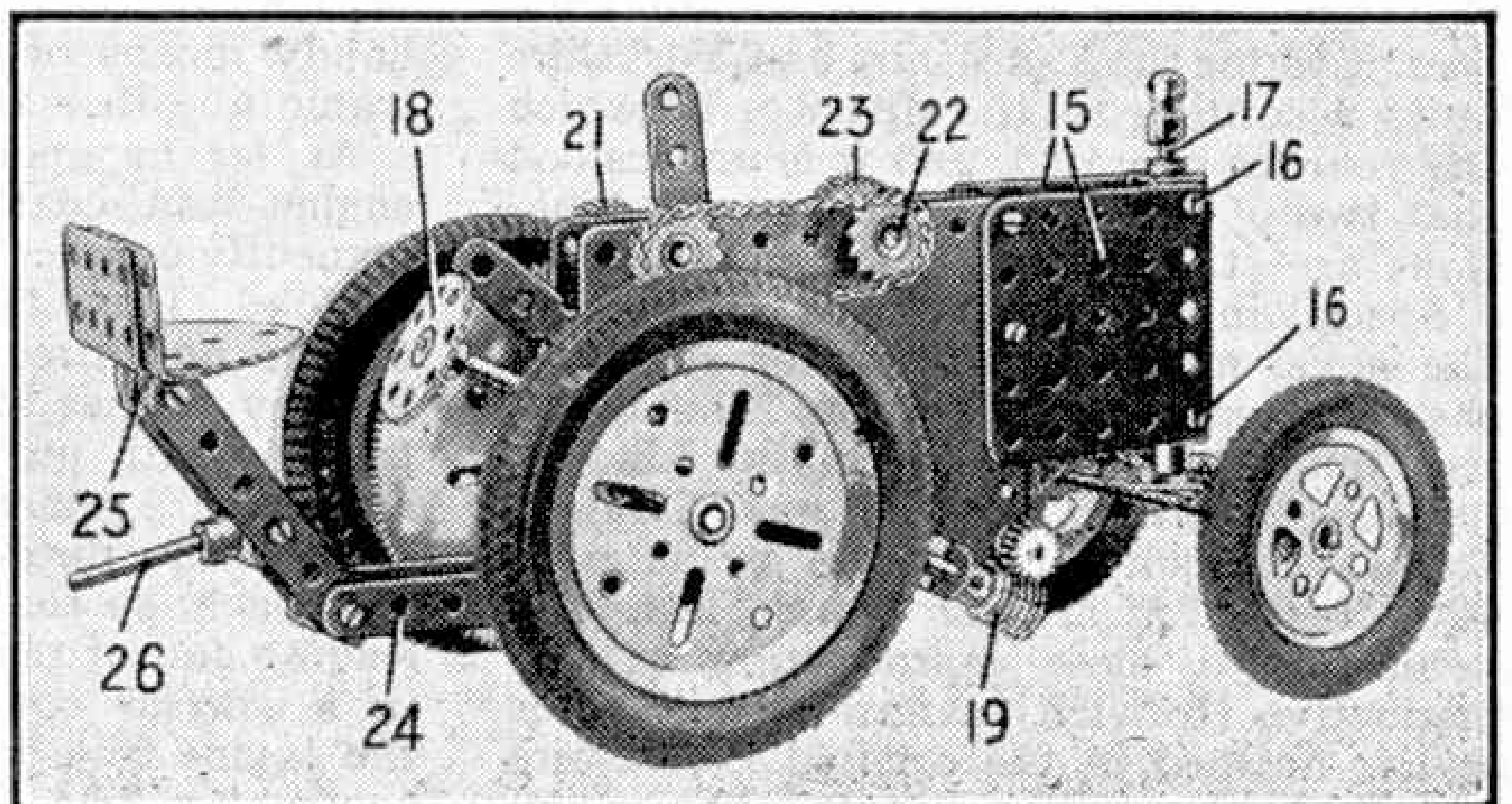
Fig. 4. A general view of the tractor. This can be used for hauling other models.
