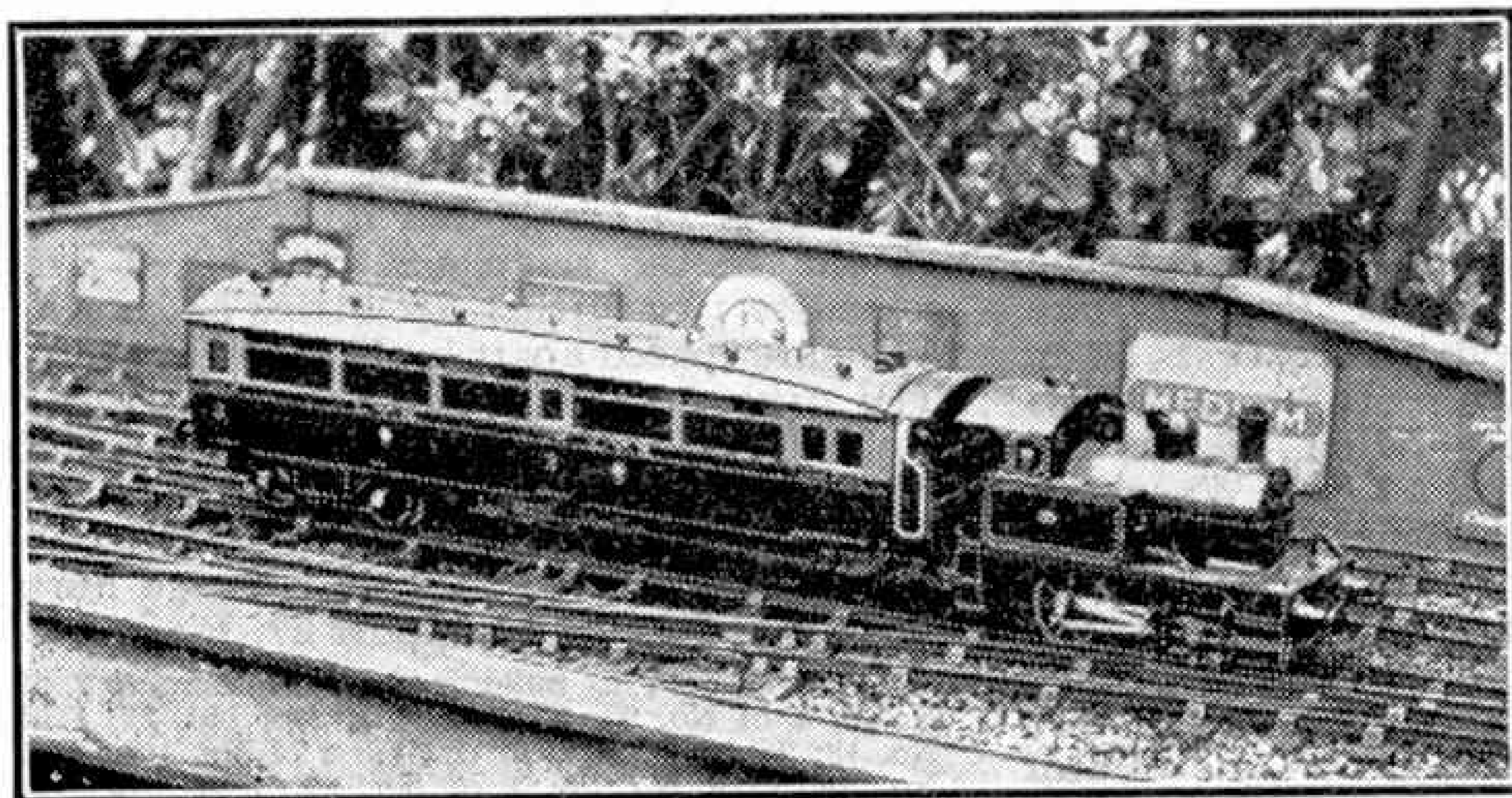
The " Dolly Tub Express " in miniature. This Gauge 0 reproduction of a former Lancashire and Yorkshire rail motor unit was built by Mr. C. B. Smith, Lincoln. The engine incorporates a Hornby M1/2 clockwork mechanism.
