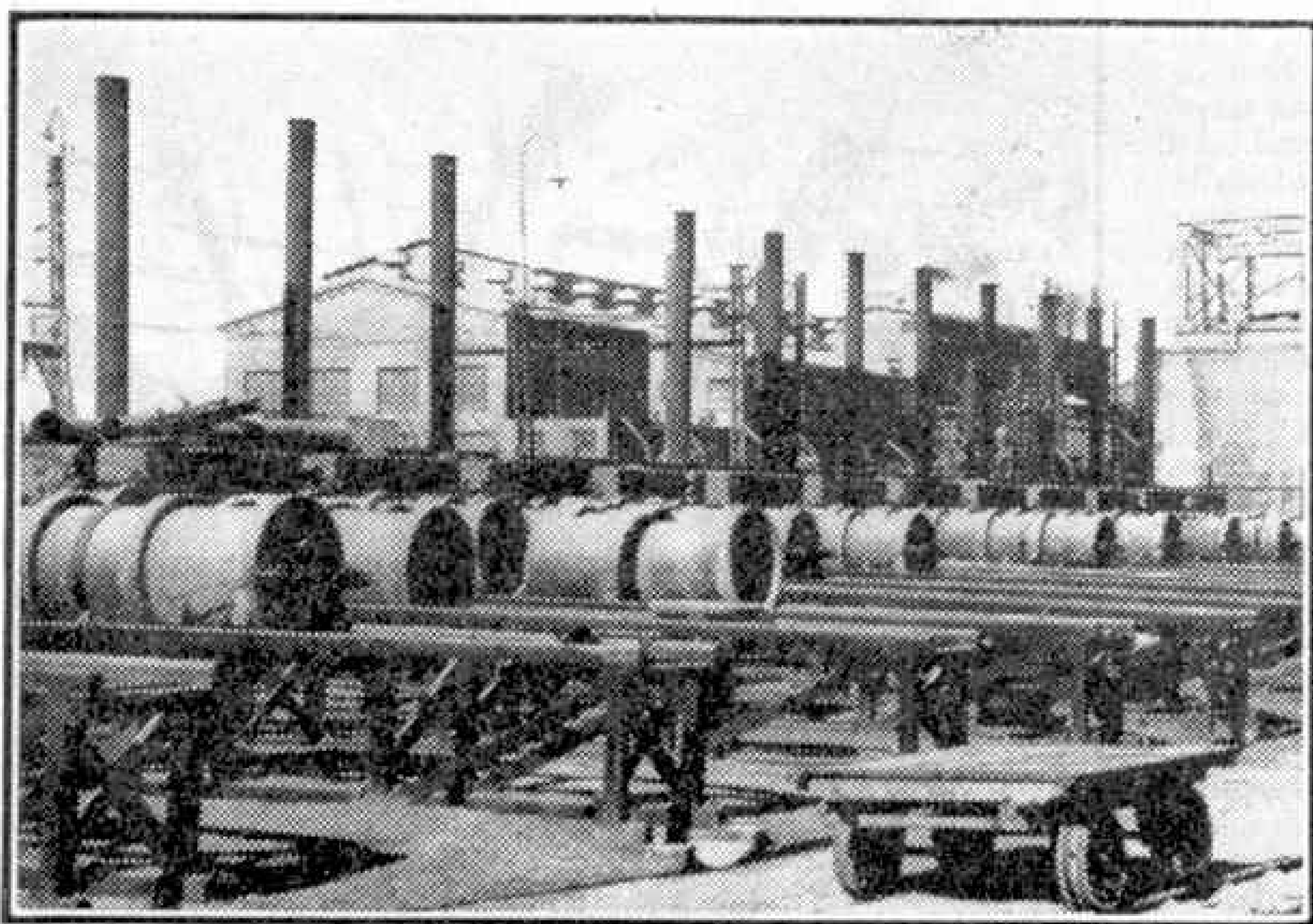
An iodine plant in Chile, where the element is recovered as an important by-product in the extraction of Chilean nitrate. The illustrations to this article are reproduced by courtesy of the Iodine Educational Bureau.
