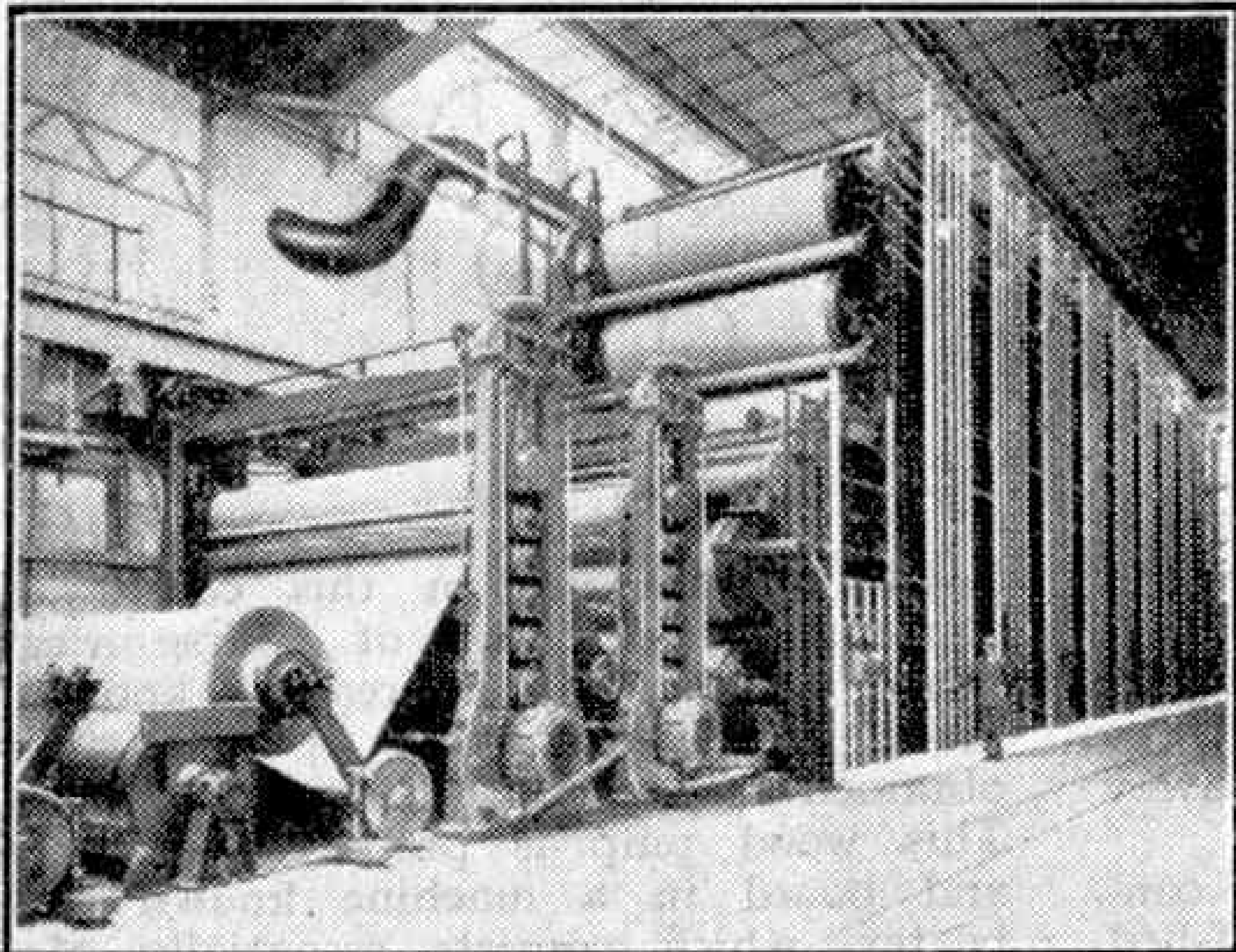
The world's largest board-making machine at Thames Board Mills. This machine is 300 ft. long, 50 ft. high and 15 ft. wide, and weighs 2,000 tons.
