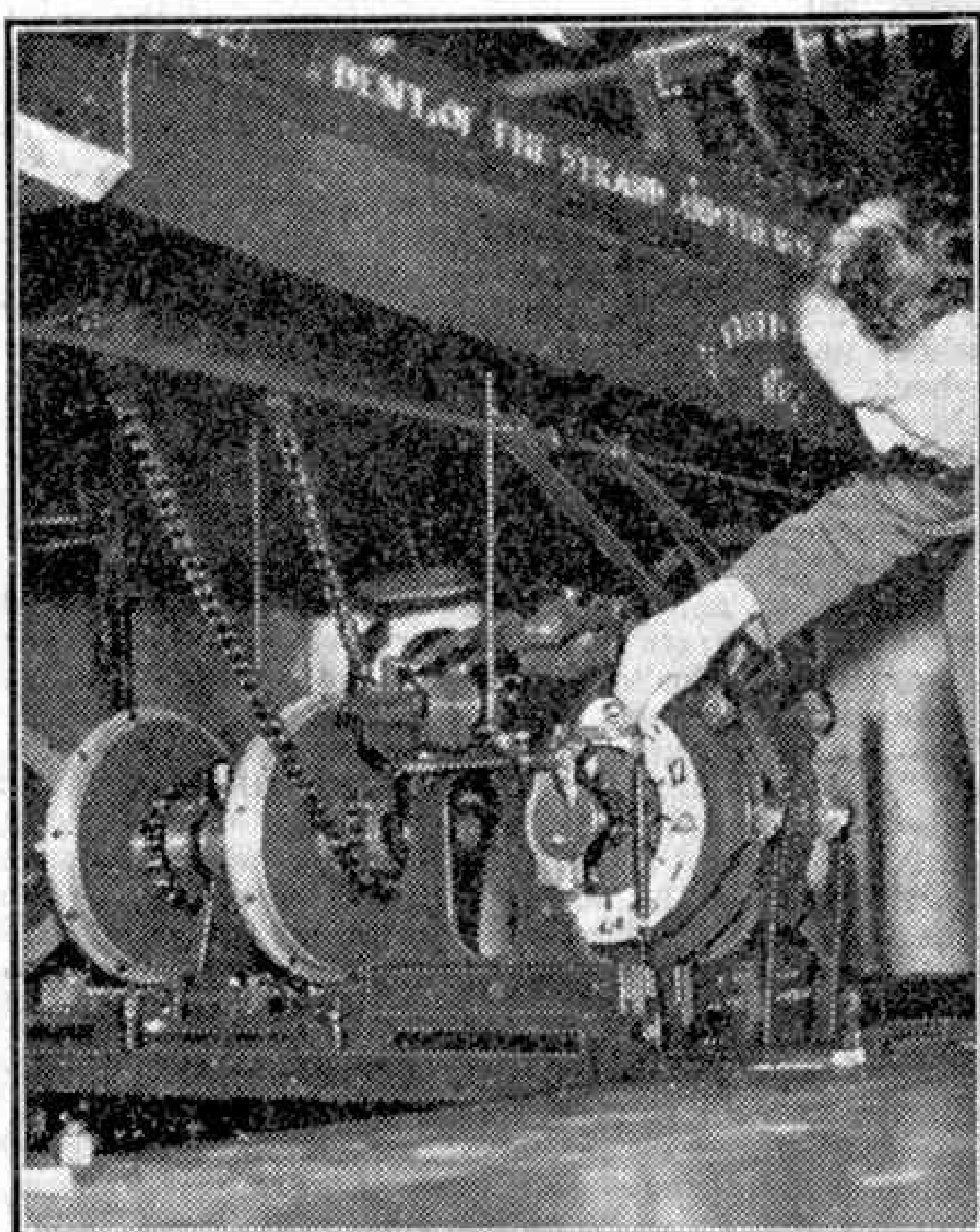
The electrically driven winding mechanism, which operates through roller chains.
