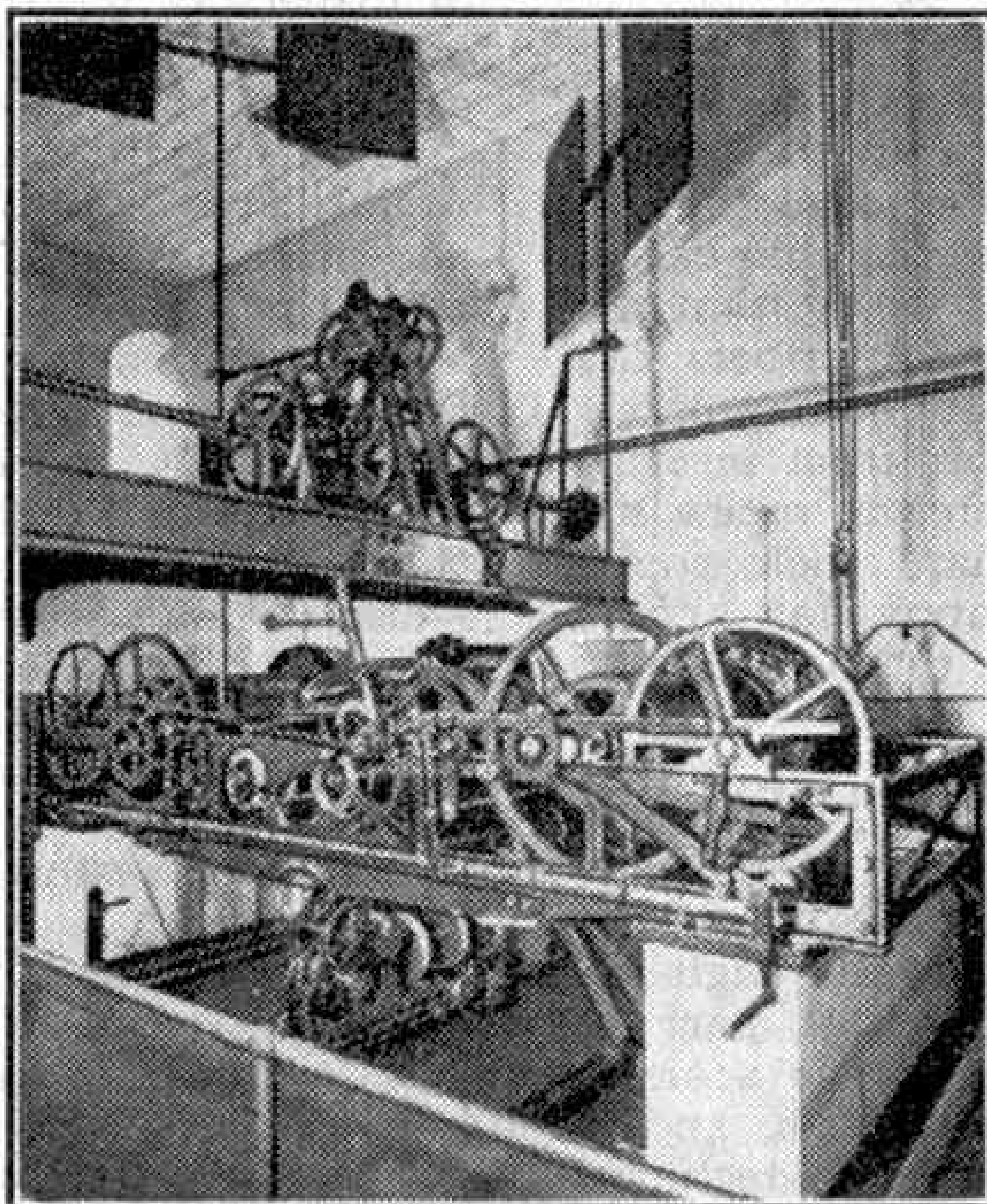
Mechanism of the great clock seen from the chiming train end, showing the bevel wheels driving the shafts to the hands. The air brakes are seen at the top of the illustration; they control the speed of chiming and striking. Photograph by courtesy of the "Horological Journal."
