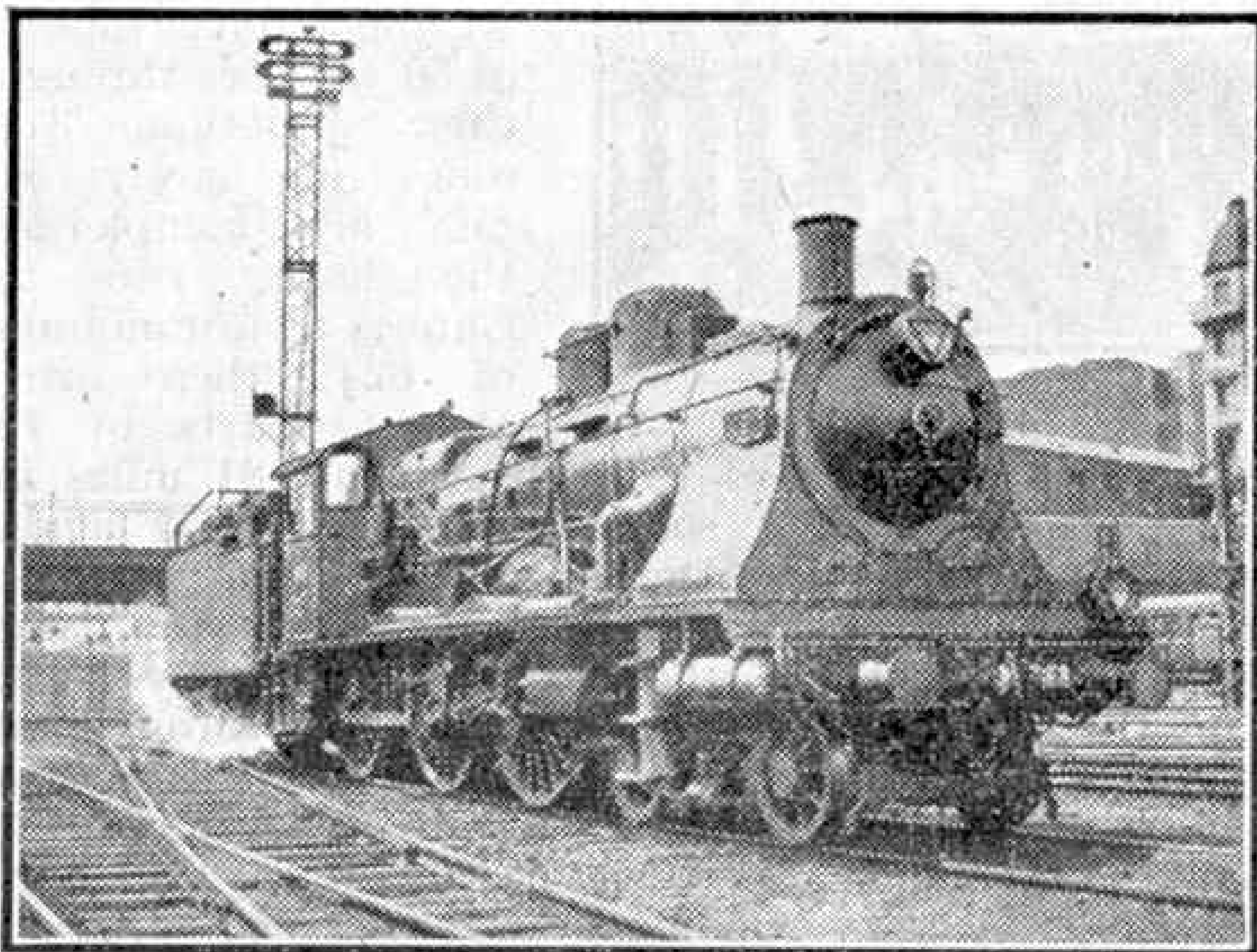
Est 4-6-0 No. 3168, with widened front and casing. Photograph by O. S. Nock.
