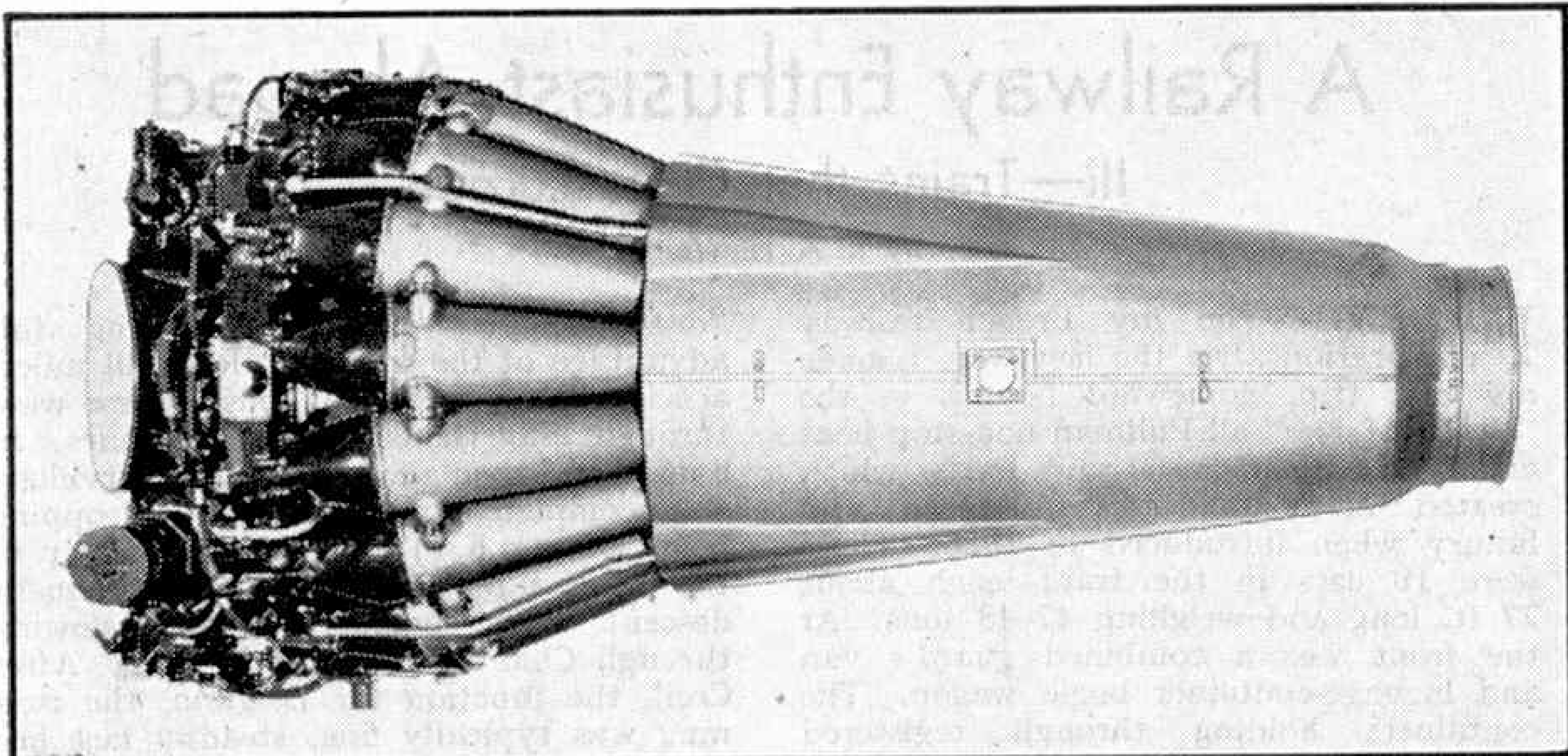
The de Havilland "Goblin" Turbojet, the standard power unit of the D.H. "Vampire" interceptor fighter. Photograph by courtesy of The de Havilland Aircraft Co. Ltd.
