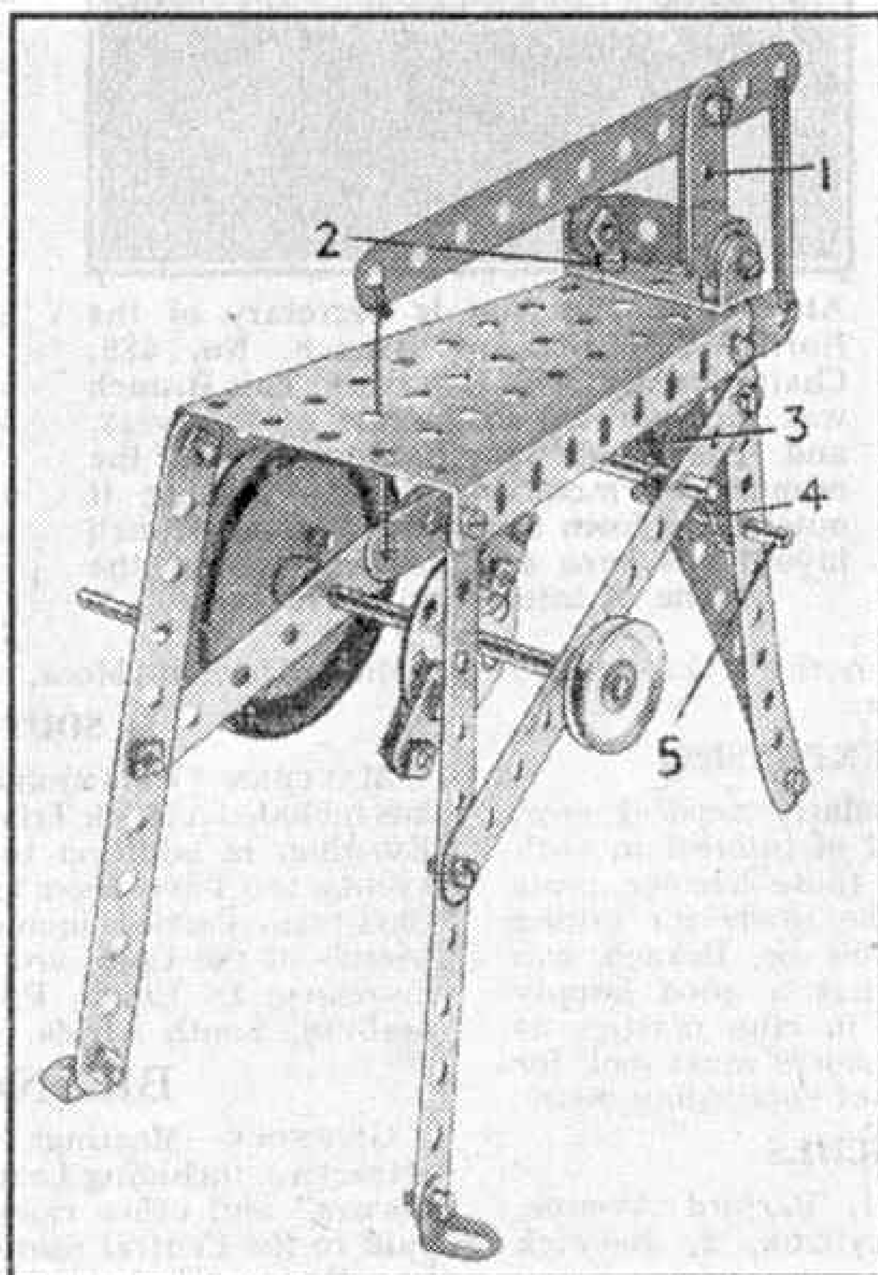
Fig. 3. A simple fret-machine that operates realistically.
