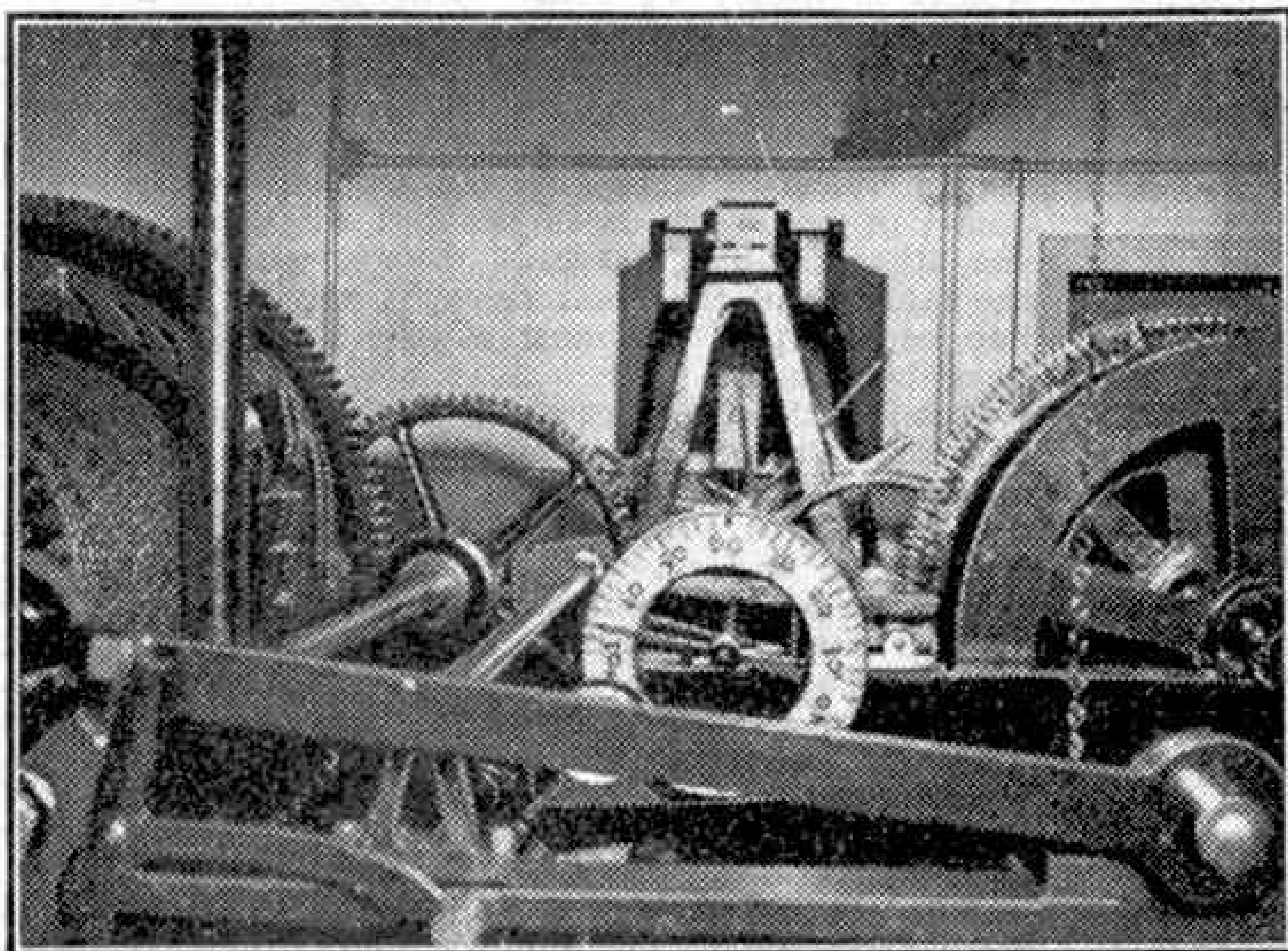
The escapement and timekeeping part of the clock, with the seconds dial. Photograph by courtesy of the "Horological Journal."
