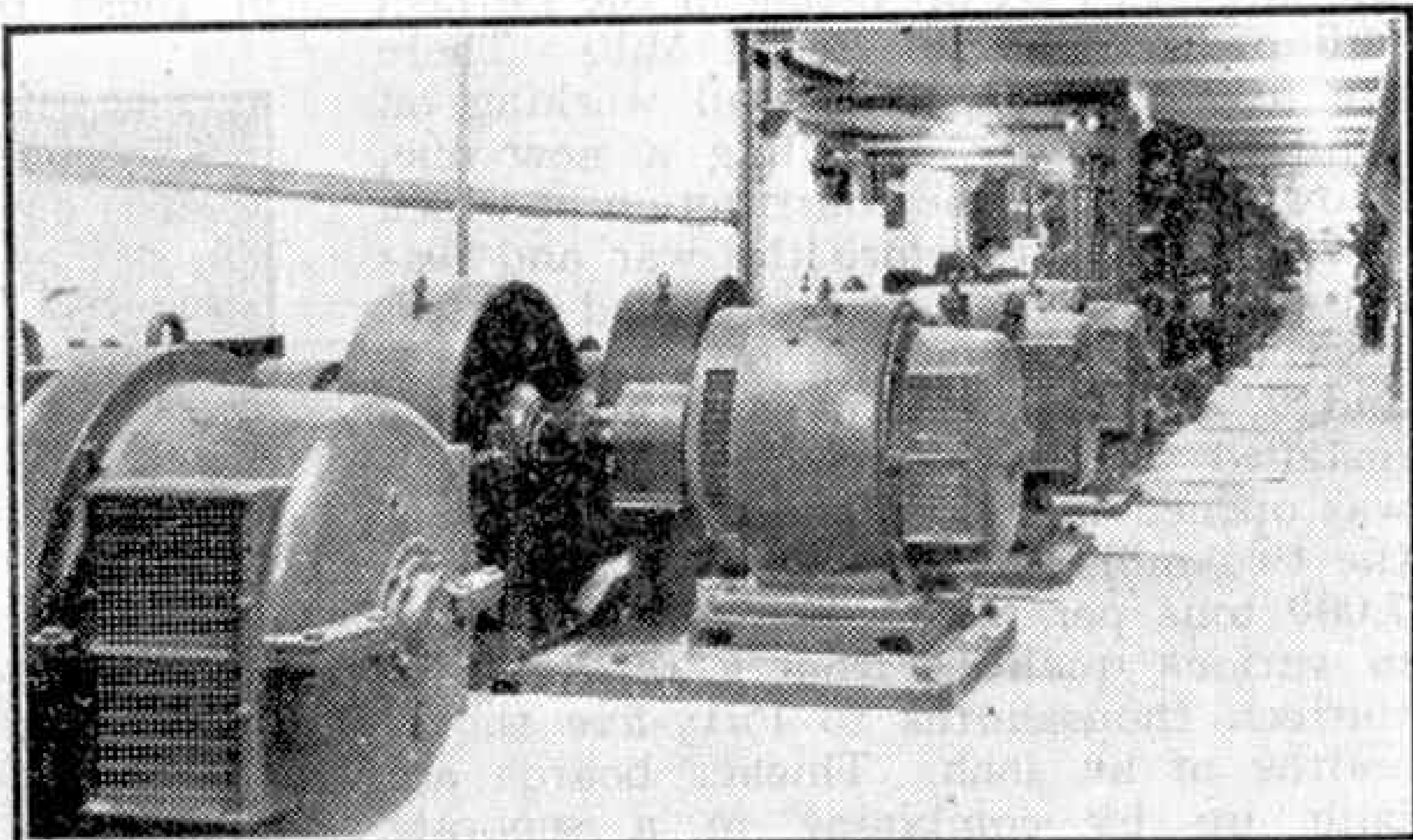
The electrical drive of a board-making machine, showing heavy-duty motors and switchgear.
