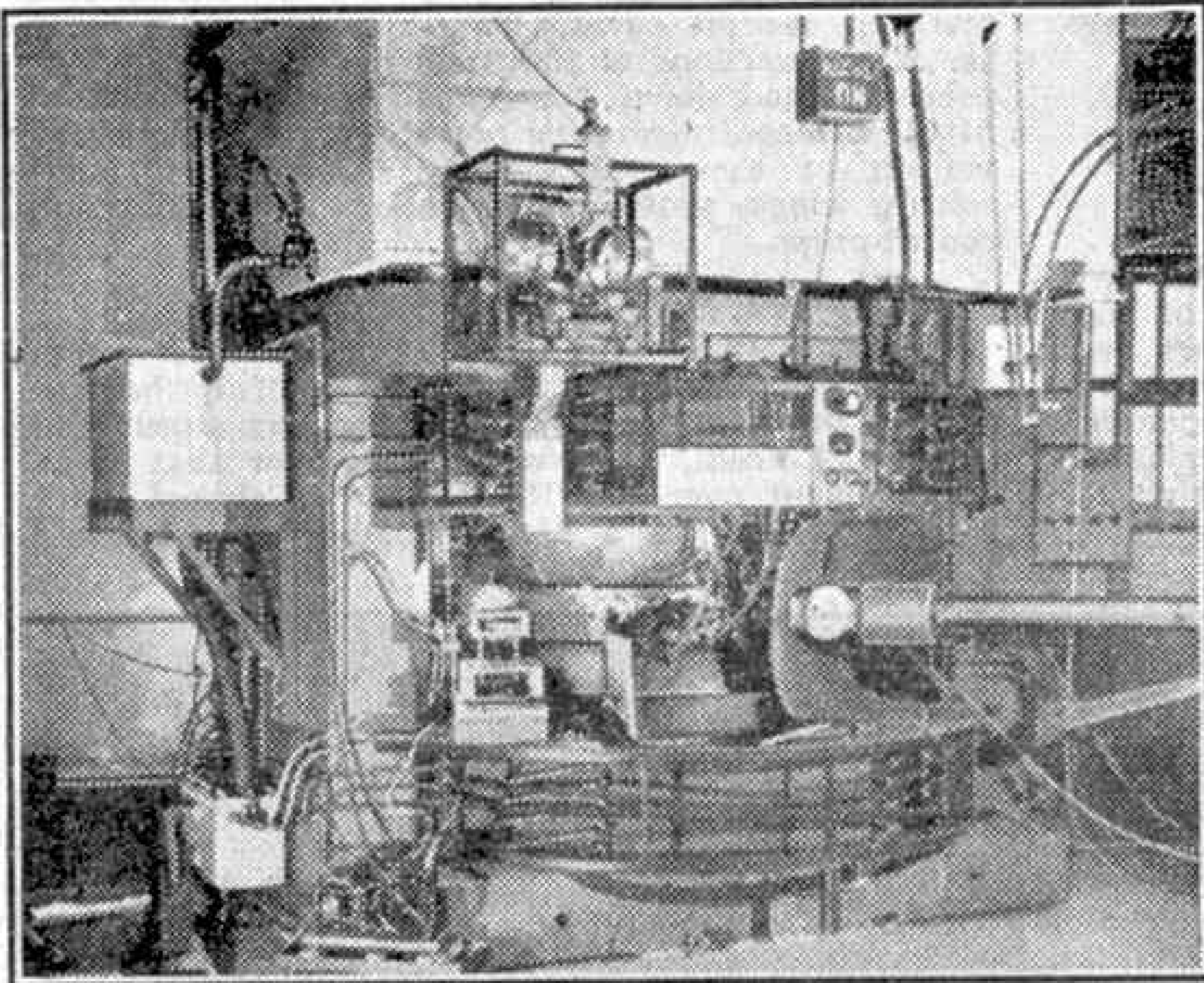
The cyclotron at Liverpool University. This machine gives high speeds to charged particles by whirling them in a spiral course under the influence of two powerful electro-magnets, and the particles are then used for atomic bombardments. Photograph by courtesy of the Physics Department, University of Liverpool.
