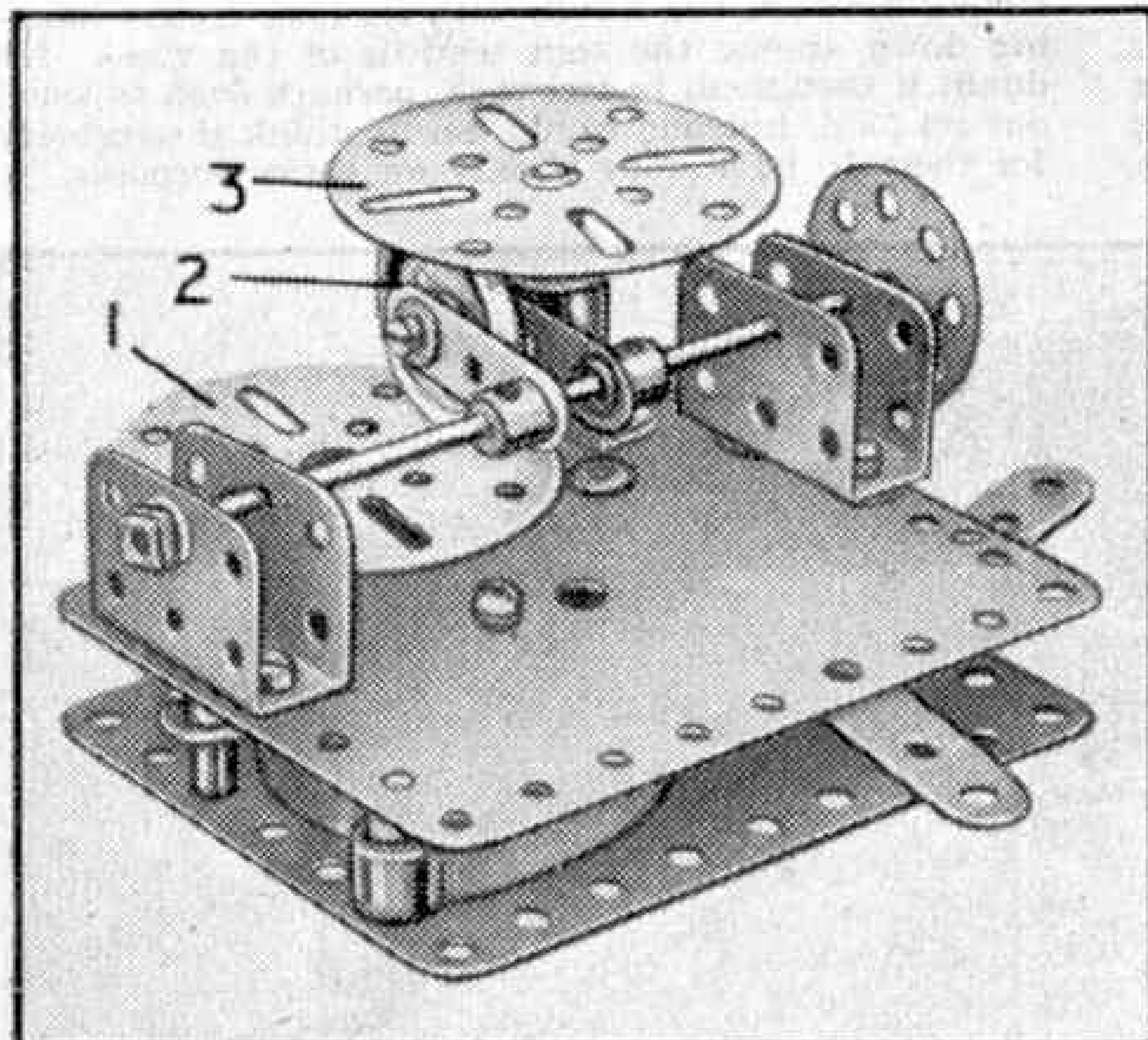
Fig. 2. A variable speed drive mechanism designed by A. Bedford, Hull.
