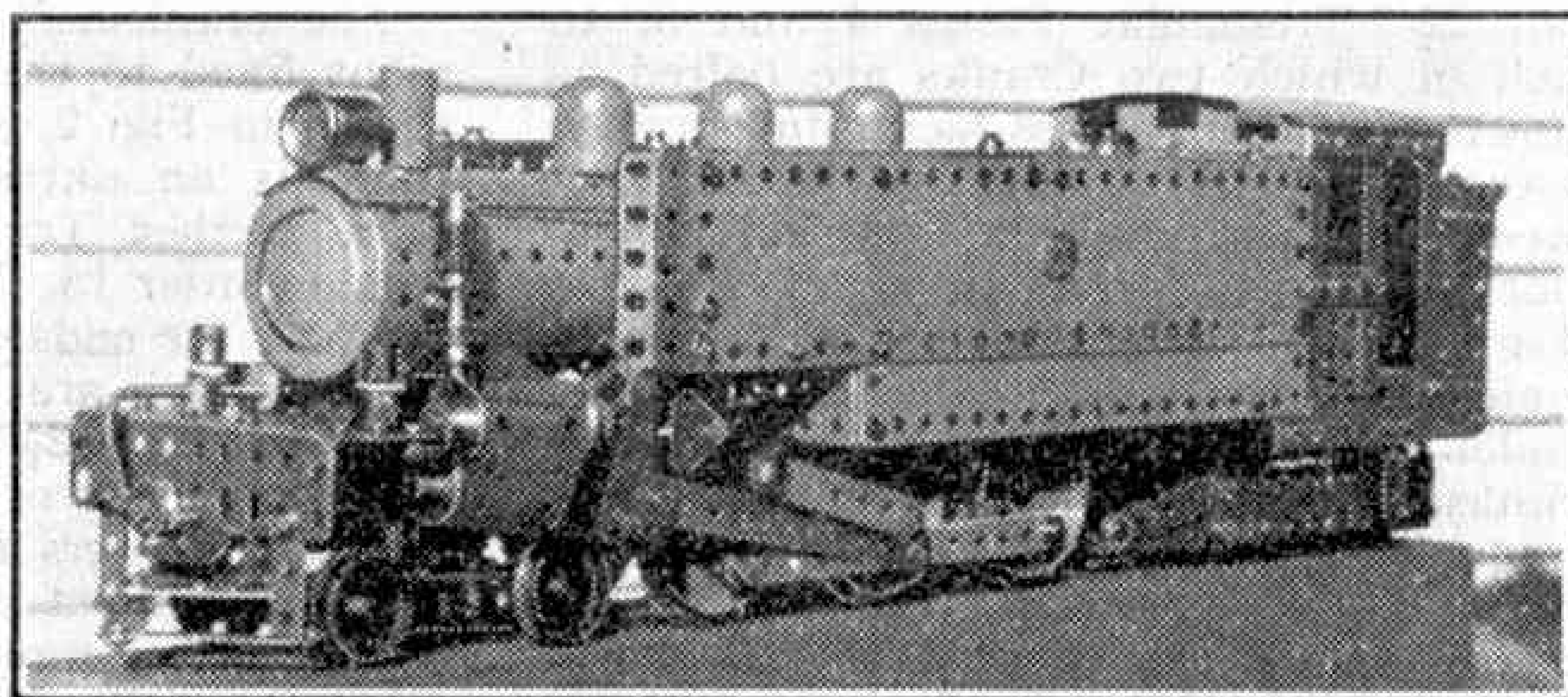
Fig. 5. This fine model 4-6-4 tank locomotive was built by N. Candish, Christchurch, New Zealand. It represents a type in service on the N.Z. Railways.
