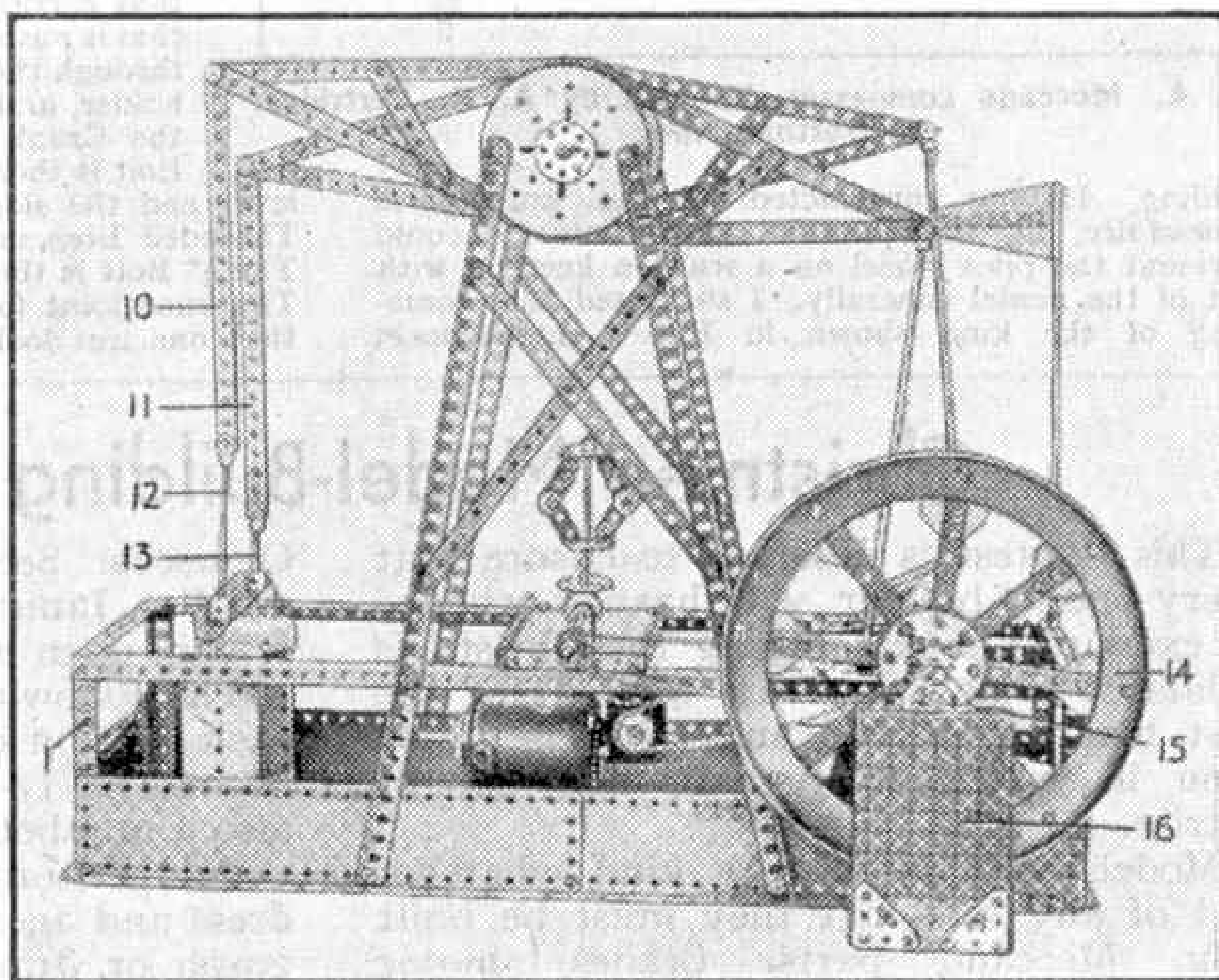
Fig. 1. A fine working model Twin Beam Engine.
