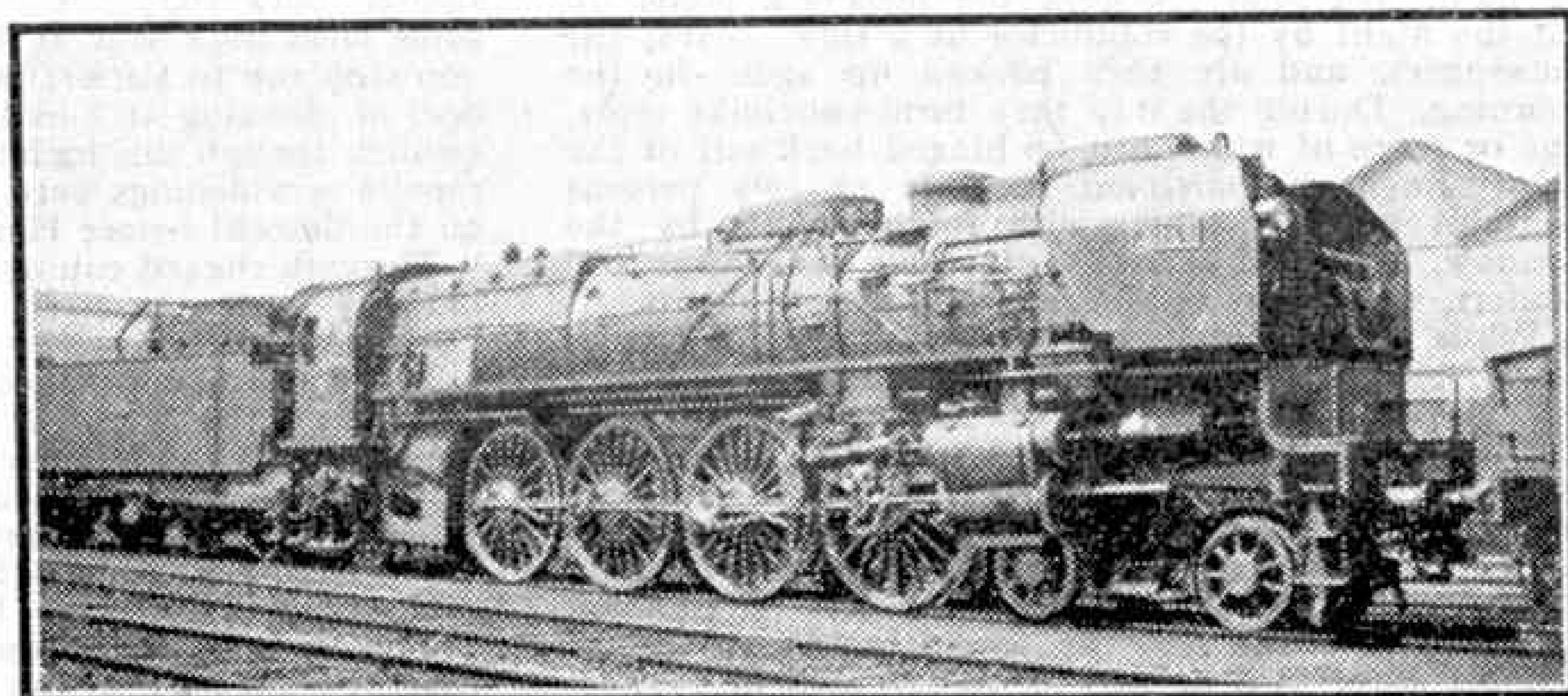
Est 4-8-2 No. 241-011 after working a Paris-Belfort express. Photograph by O. S. Nock.
