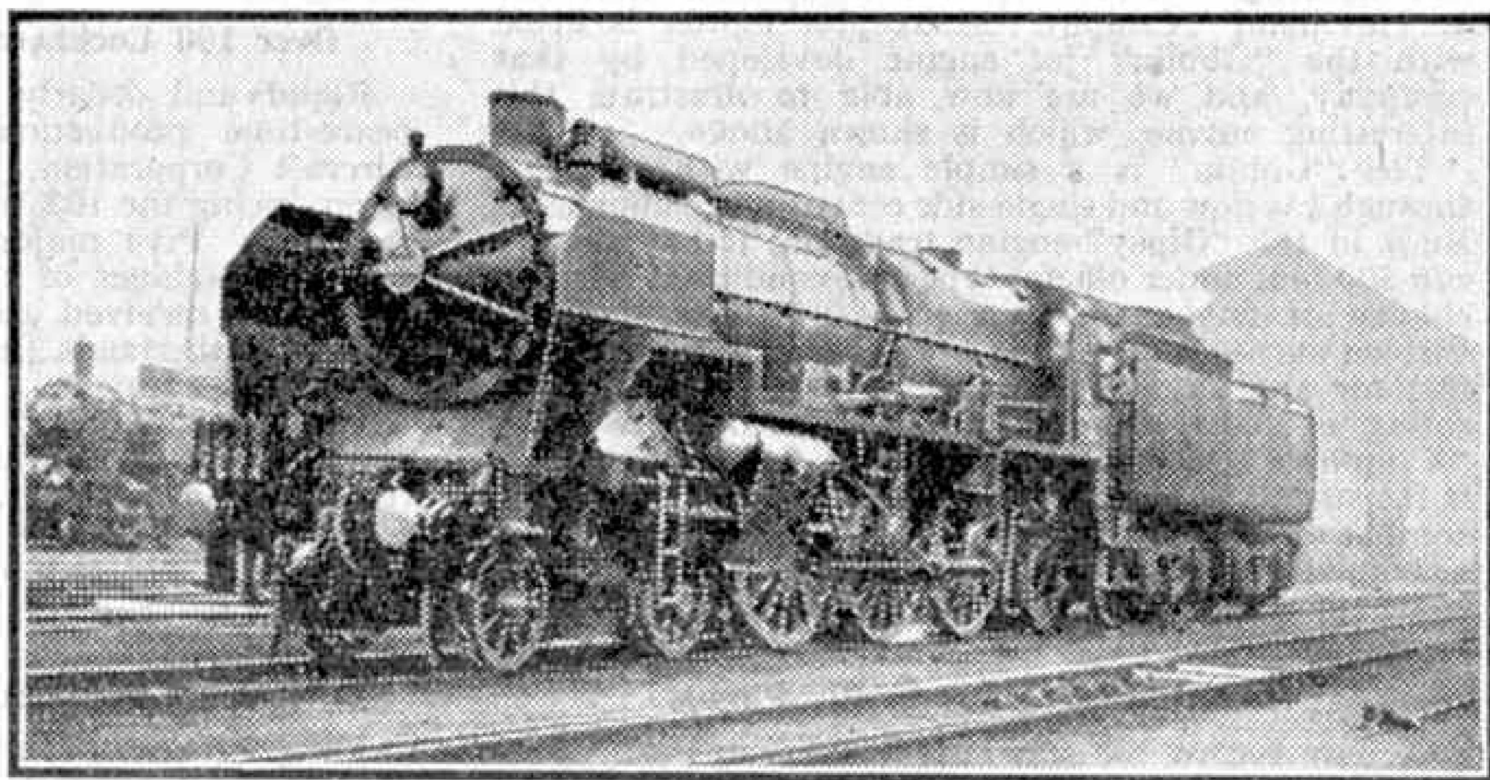
Nord 4-cyl. "Pacific" compound working an English boat train from Paris. Photograph by O. S. Nock.
