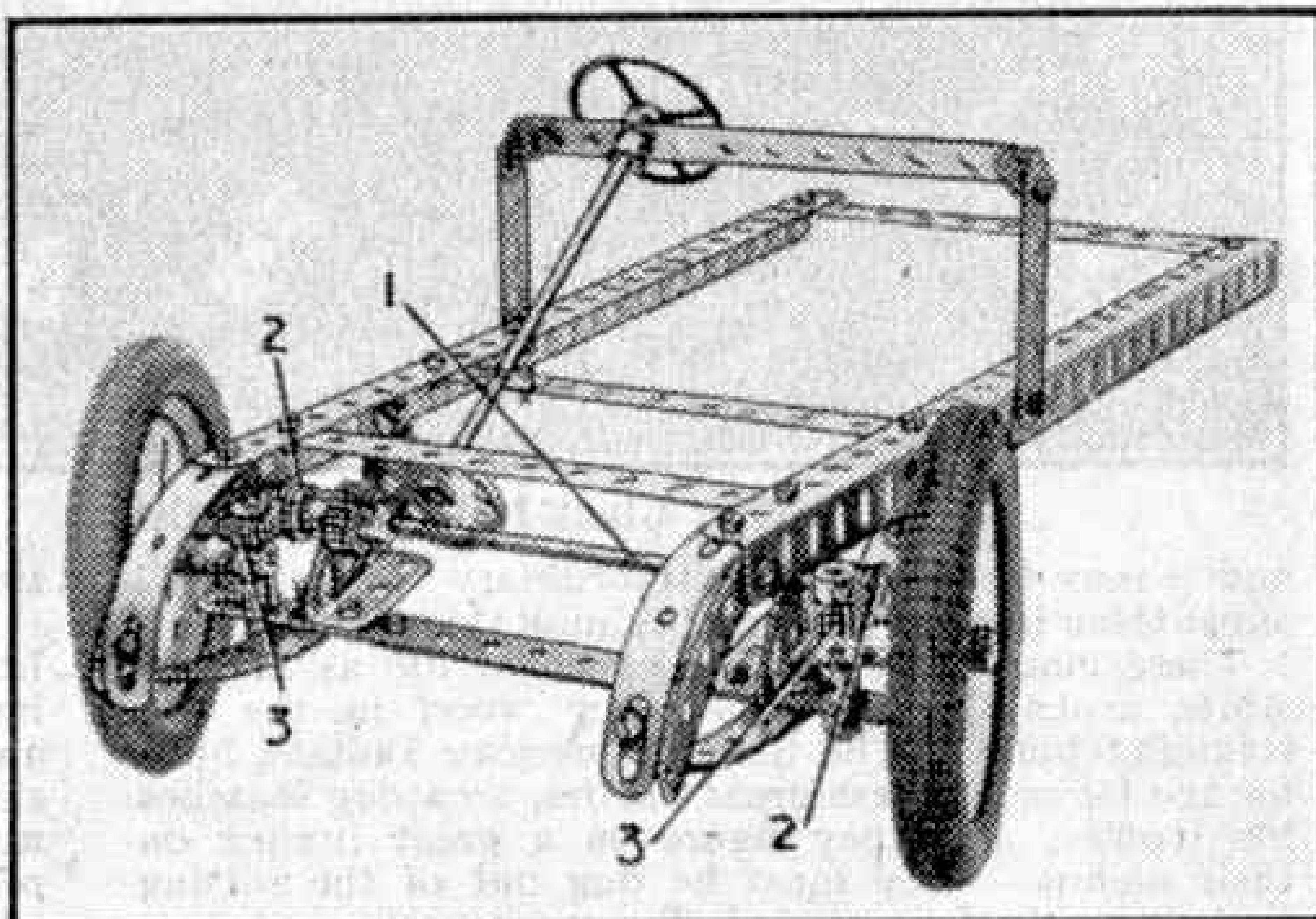
Fig. 1. Positive front wheel steering gear for model motor vehicles.
