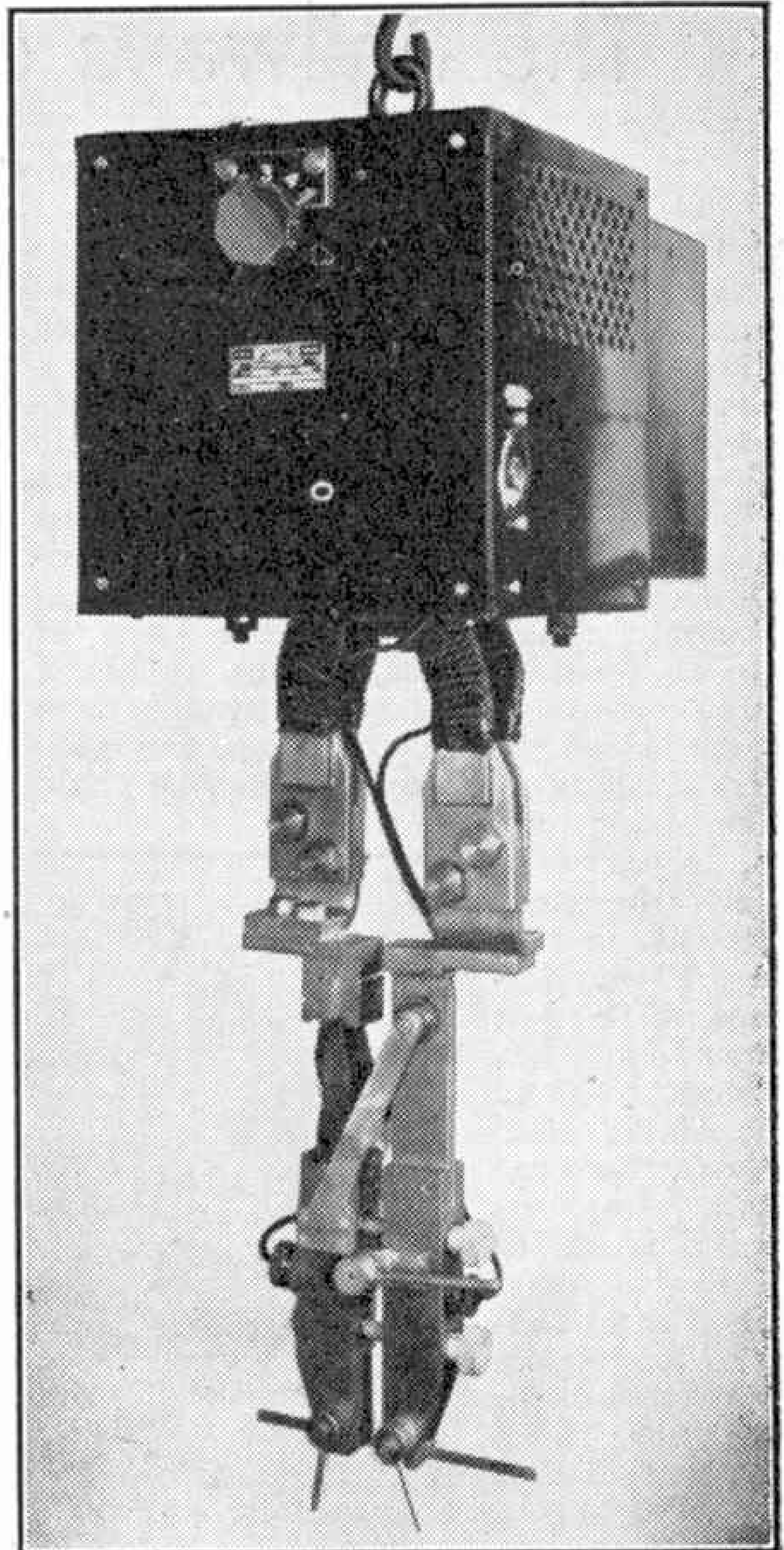
A portable butt welding machine manufactured by Metropolitan-Vickers Electrical Co. Ltd., to whom we are indebted for our illustration.
