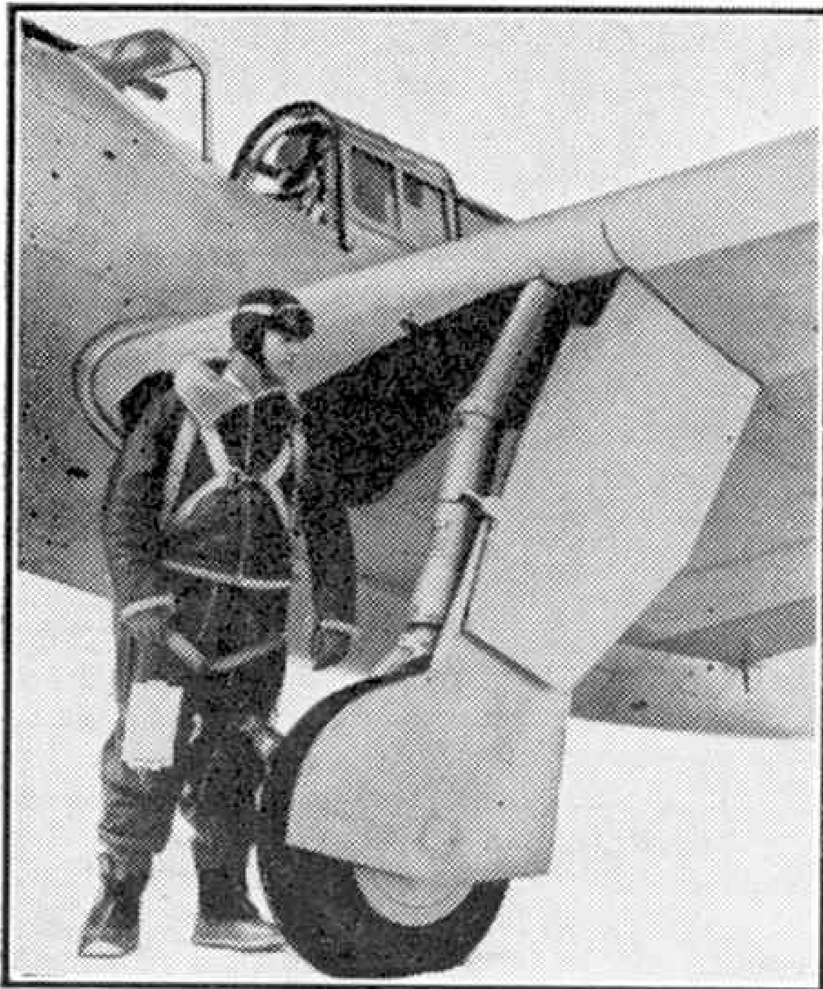
Lloyd Child, Curtiss-Wright chief test pilot, inspecting the retractable landing gear of the new dive-bomber. Photographs by courtesy of Curtiss-Wright Corporation, U.S.A.
