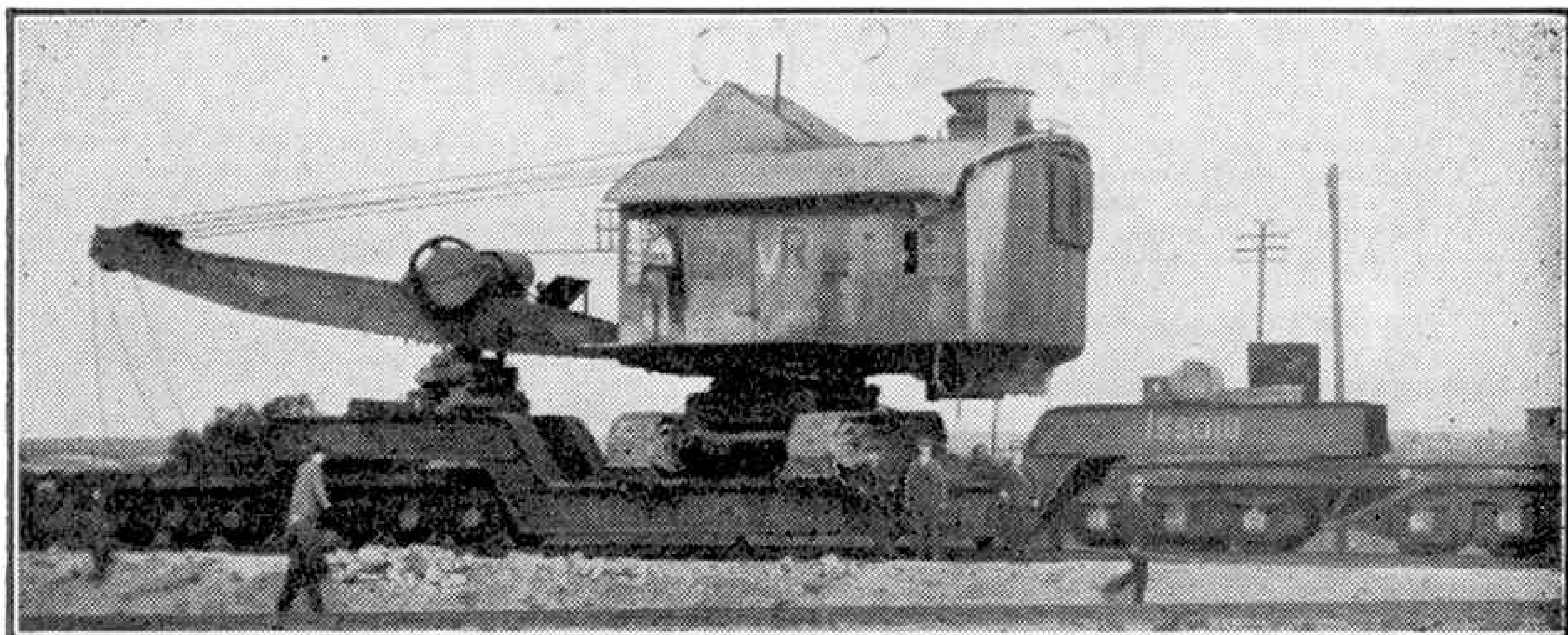
A 74-ton Diesel-engined navy mounted on a 110-ton L.N.E.R. trolley wagon for transport by rail. Photograph by courtesy of the "London and North Eastern Railway Magazine."
