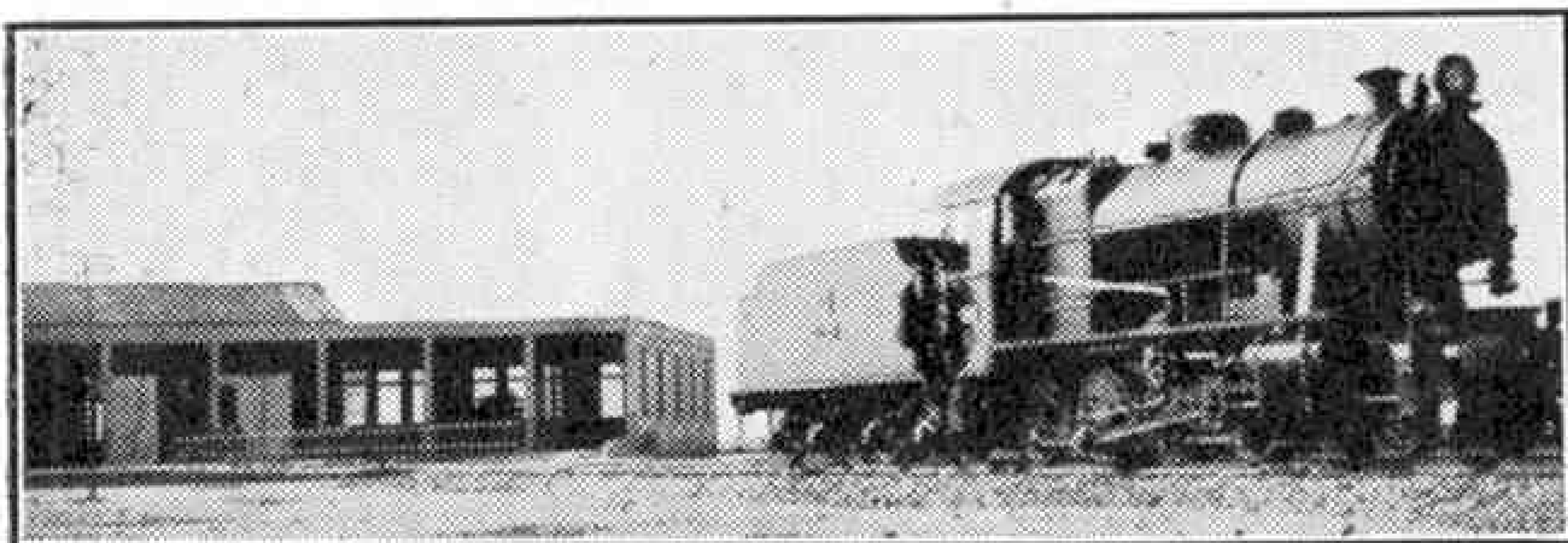
A Beyer-Peacock 2-8-0 locomotive outside Ahwaz running shed. Photograph by courtesy of Beyer, Peacock and Co. Ltd.
