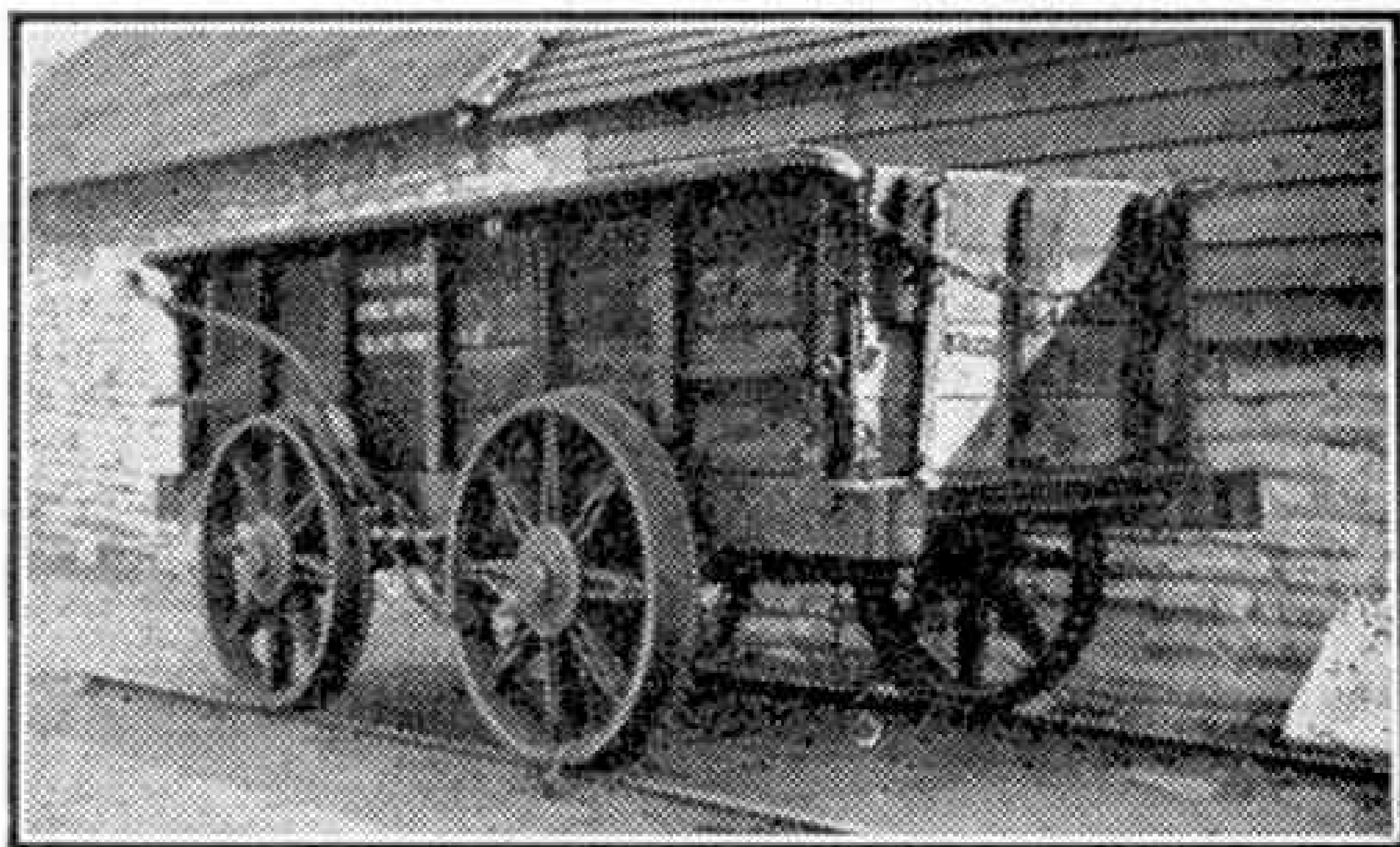
A horse-drawn goods truck constructed in 1826. This was in use on the Stratford and Moreton-in-the-Marsh railway. Photograph by C. R. Rowson, Liverpool.
