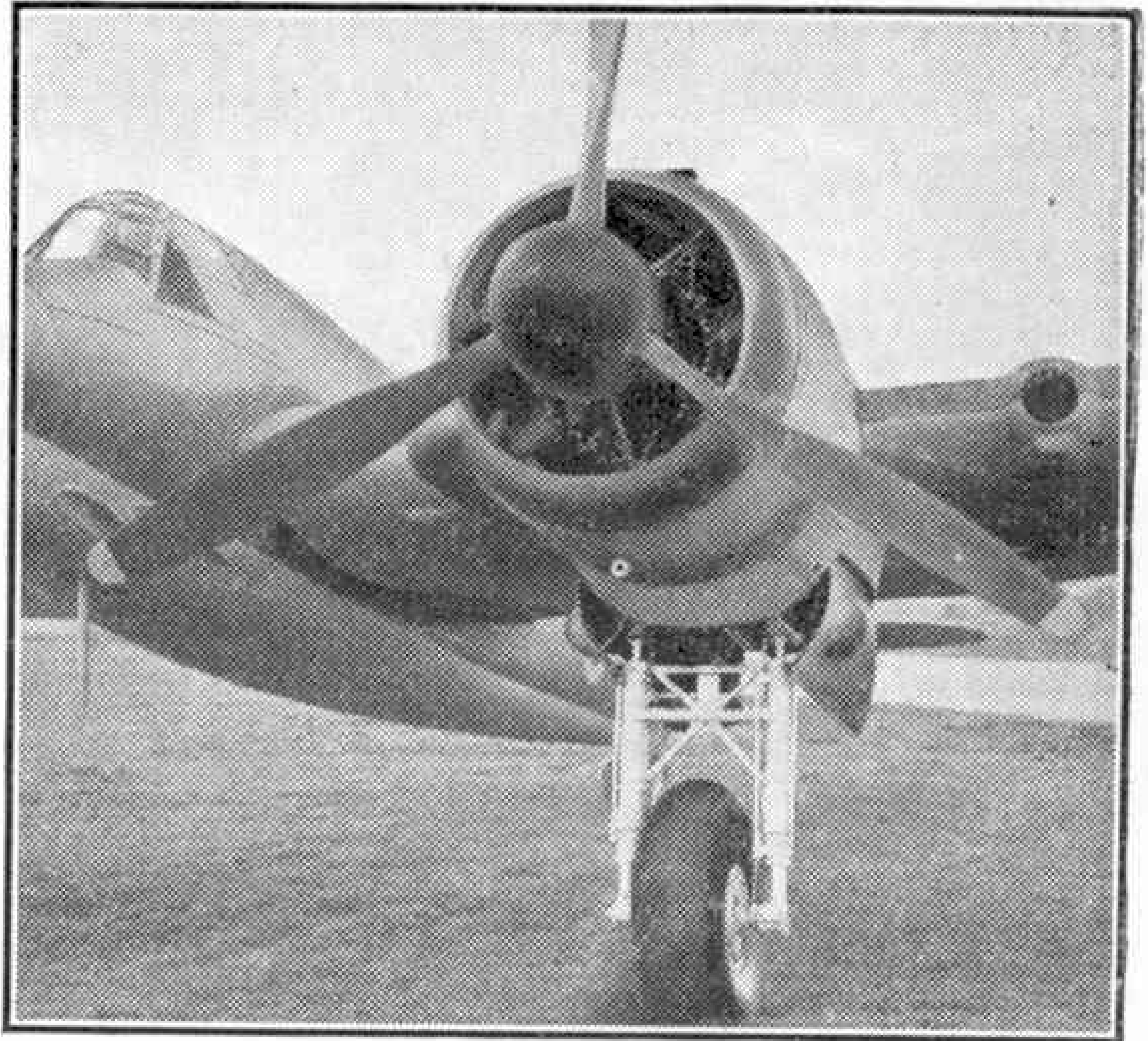
Close-up of the port engine and undercarriage leg of a "Bristol" Beaufighter. Note the curved doors which close over the undercarriage unit when this is retracted. Photograph by courtesy of Bristol Aeroplane Co. Ltd.
