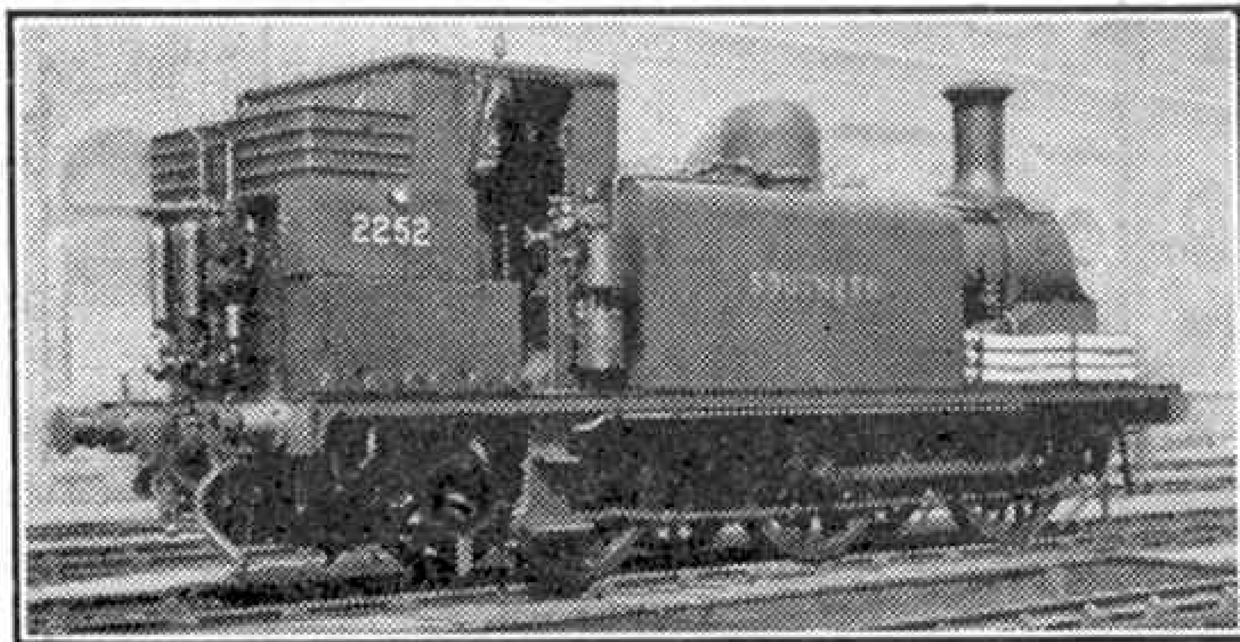
S.R. locomotive fitted with fire-pumps.
