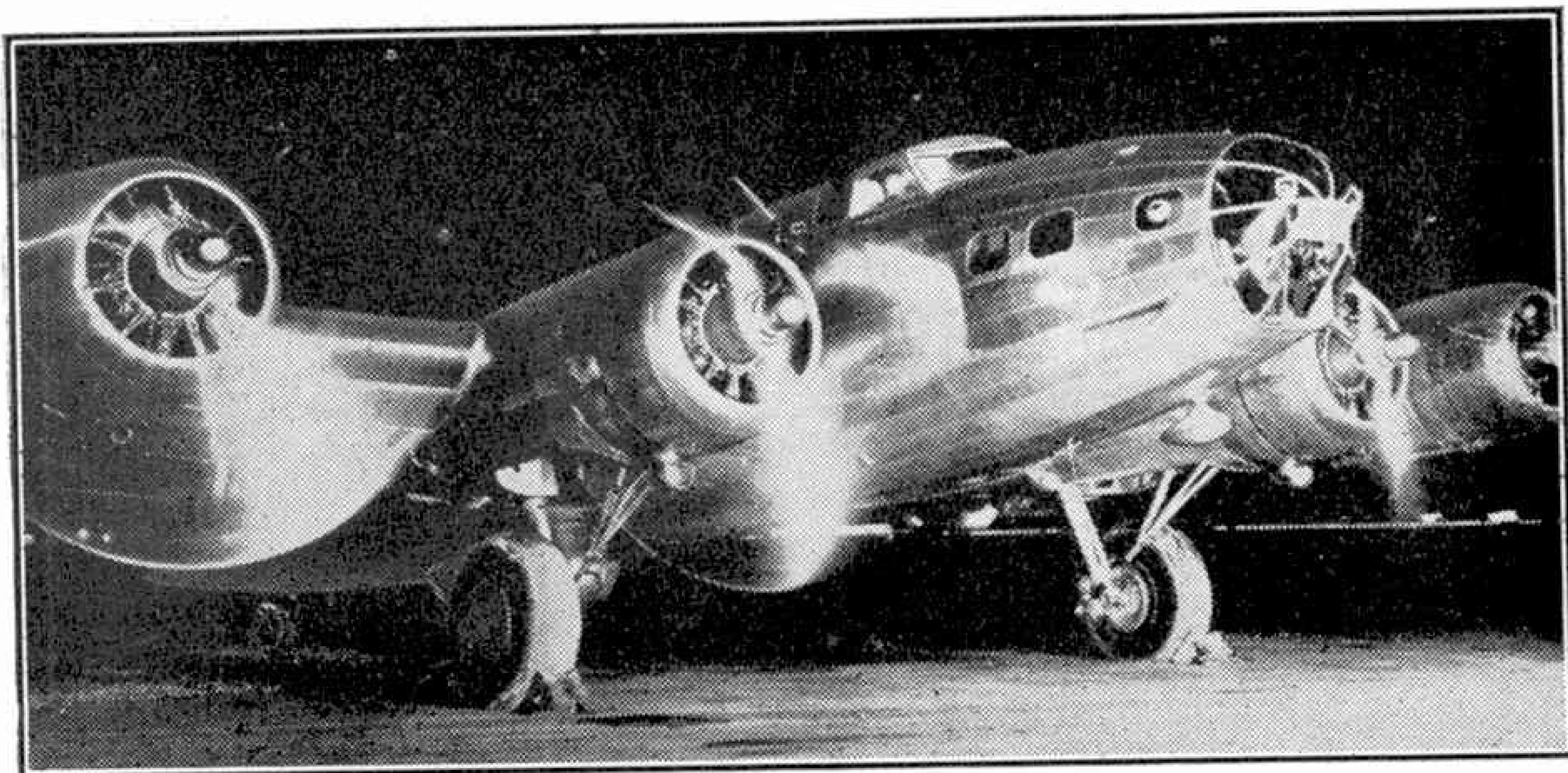
"Running in" the newly-installed 1,200 h.p. Wright "Cyclone" engines of a Boeing "Flying Fortress" bomber. The job is being done during the night shift, preparatory to flight testing the machine the next day. Photograph by courtesy of the Boeing Aircraft Company, U.S.A.
