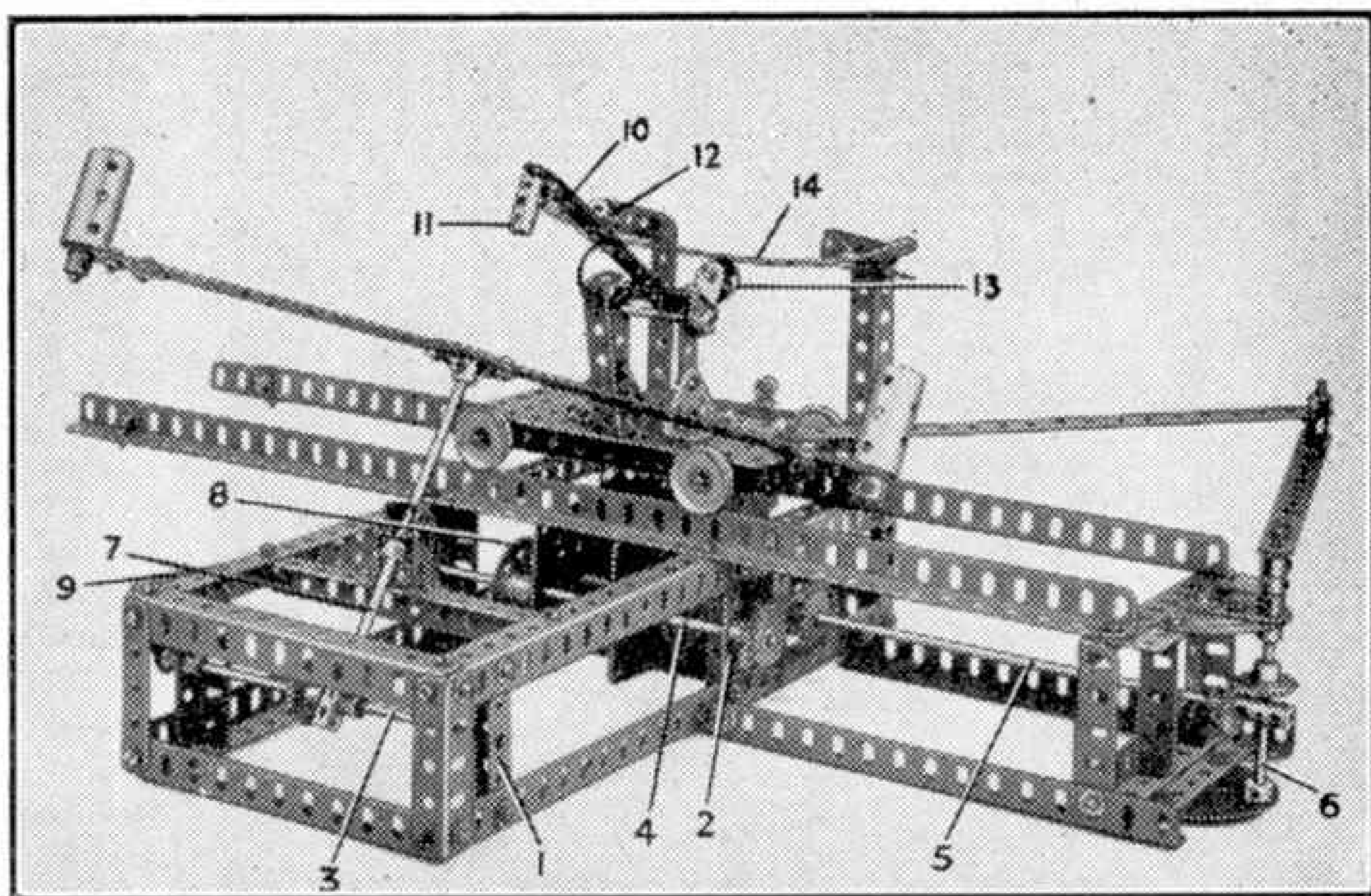
Fig. 1. A useful wool-winding machine that is interesting to construct and operate.
