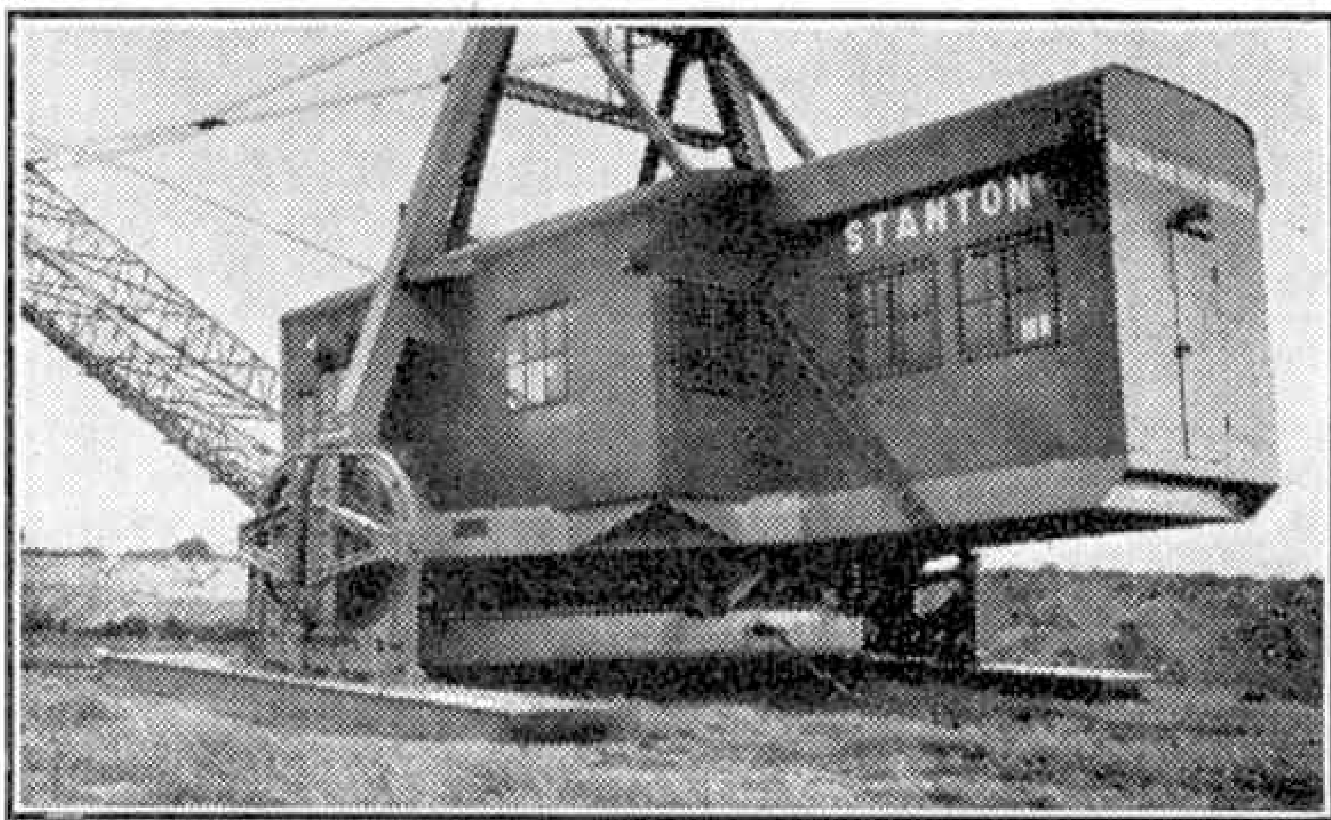
A 5-W Ruston Bucyrus-Monighan walking dragline showing the action. The walking shoes are hard down on the ground, and it is just "stepping back." The illustrations to this article are by courtesy of Ruston-Bucyrus Ltd., Lincoln, England.
