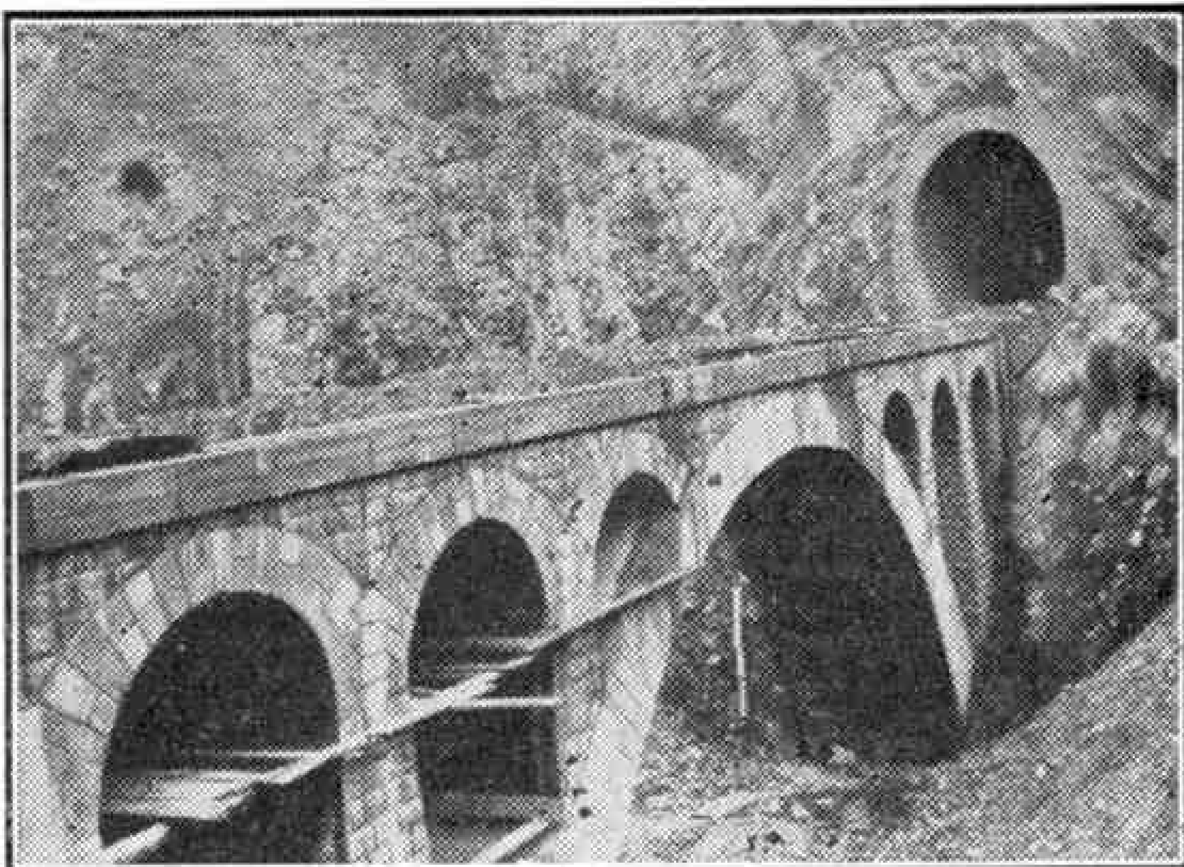
A tunnel portal. Photograph by courtesy of Richard Costain Ltd.
