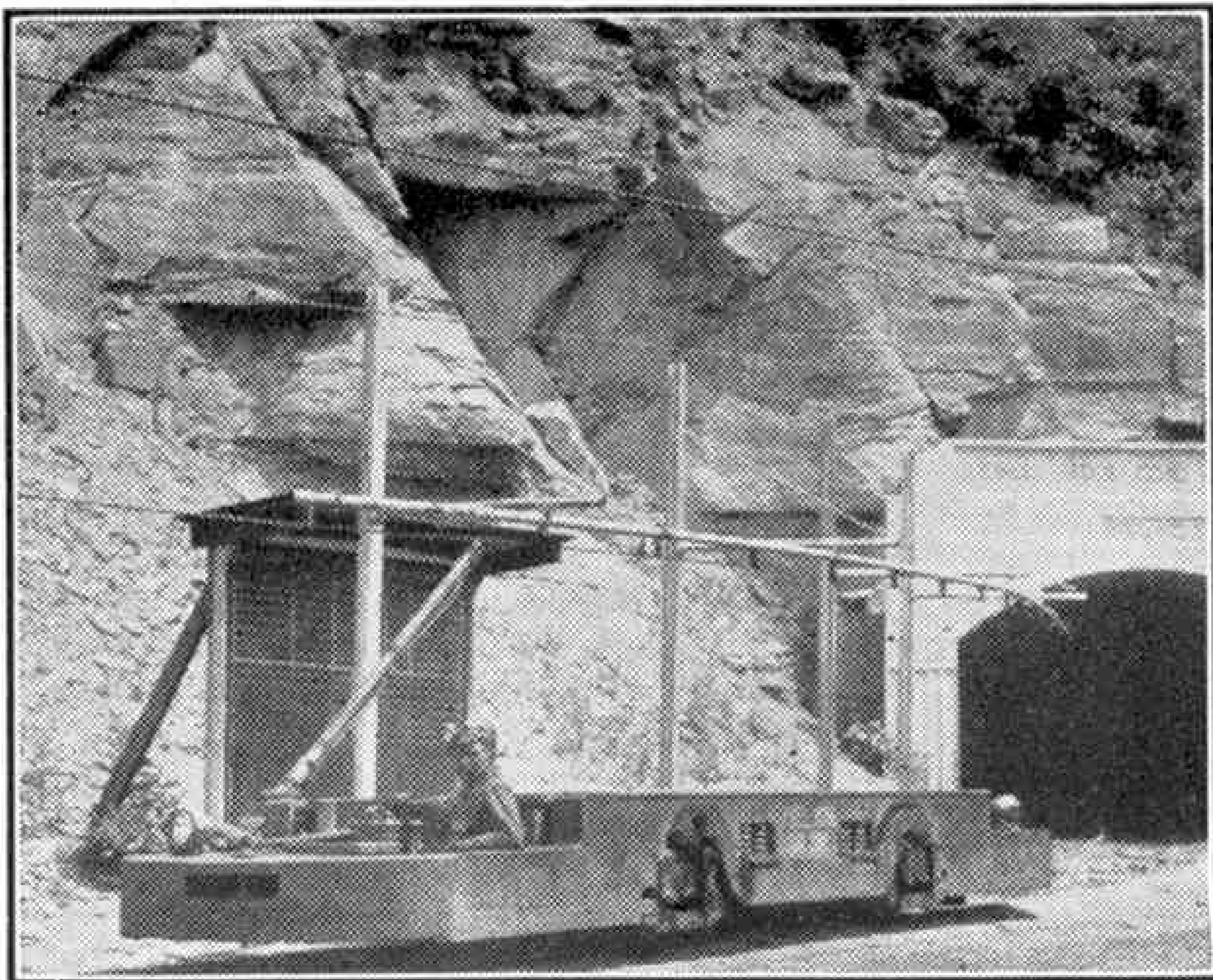
The first of a new type of low height electric locomotives. It is at work at the mines of the Jewell Ridge Coal Corporation, in the United States, and entry to the workings is by a tunnel instead of the more usual shaft. Photograph by courtesy of the General Electric Company, of New York.
