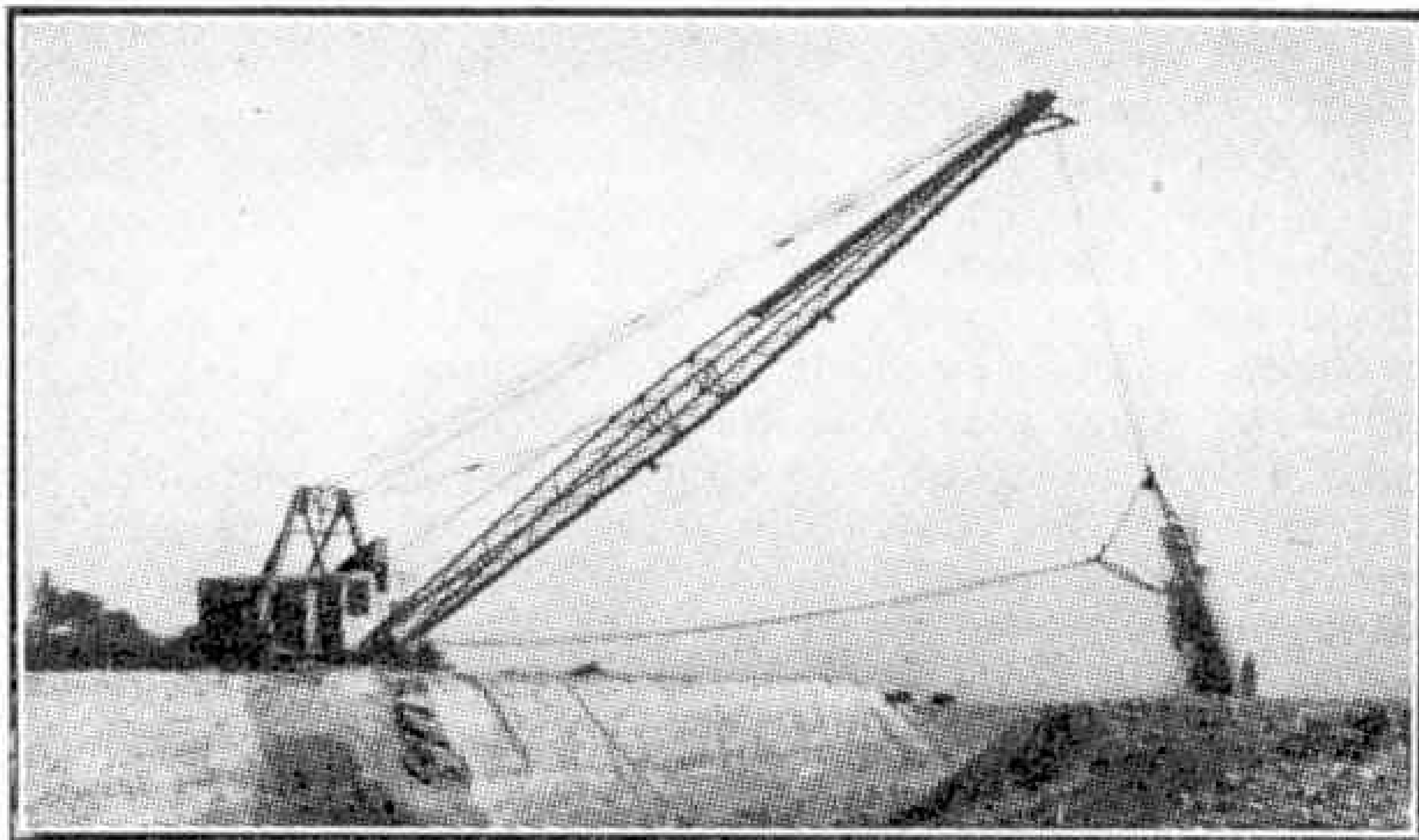
A Ruston Bucyrus-Monighan walking dragline stripping a bed of ironstone.
