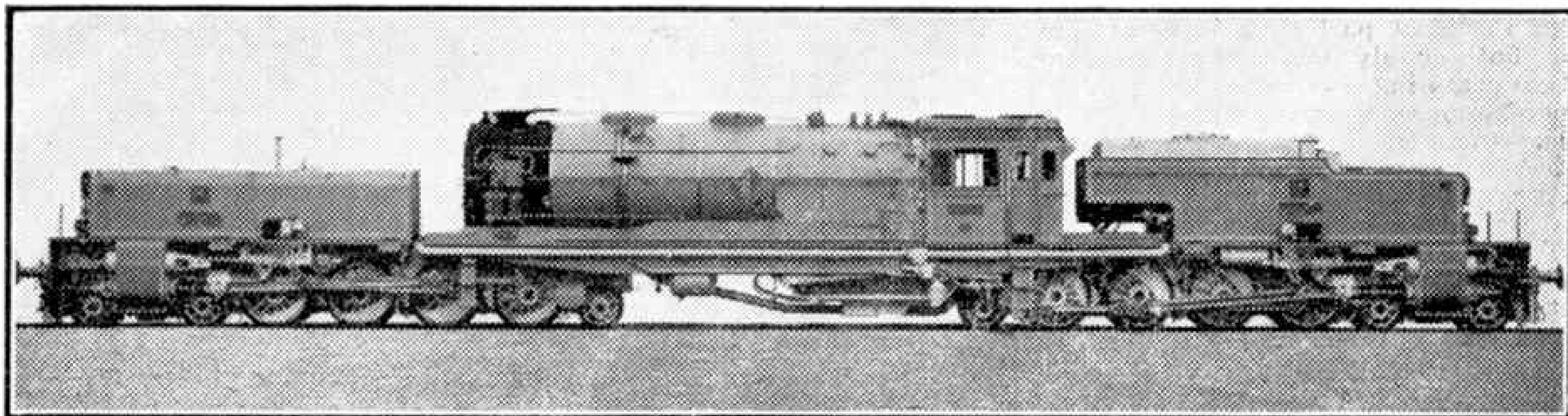
One of the enormous Beyer-Garratt engines now at work on the Northern section of the Trans-Iranian Railway. Photograph by courtesy of Beyer, Peacock and Co. Ltd.
