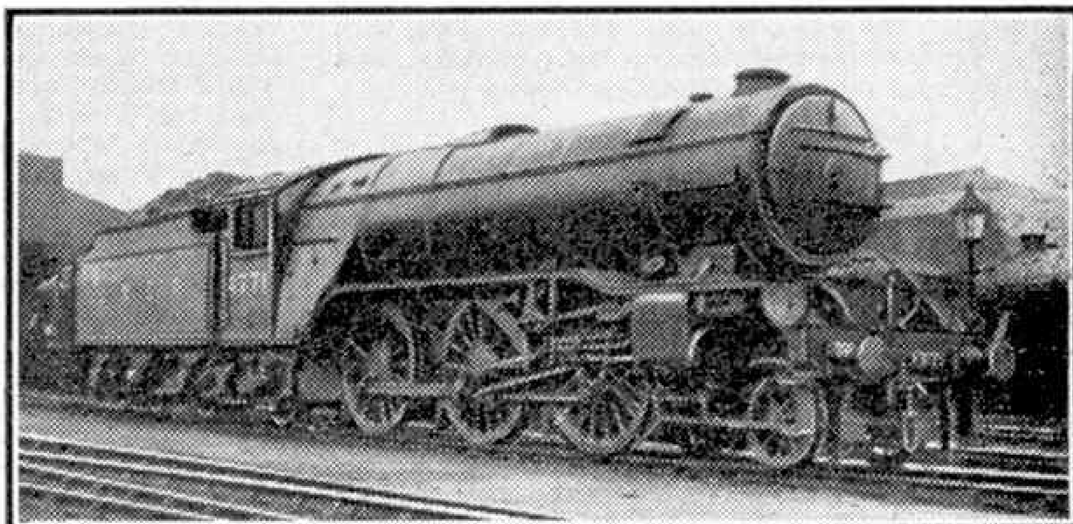
L.N.E.R. "V2" Class 2-6-2 locomotive No. 4771 "Green Arrow." These engines frequently haul express passenger or freight trains weighing up to 750 tons.
